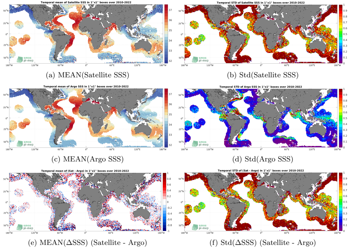
Figure 6: Temporal mean (left) and Std (right) of SSS from SMOS SSS L2Q v330 - 0.25 Deg (CATDS-CPDC) (top), Argo (middle), and of \Delta SSS (Satellite - Argo). Only match-up pairs are used to generate these maps.
