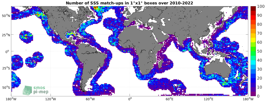
Figure 4: Number of SSS match-ups between Argo SSS and the SMOS SSS L2Q v330 - 0.25 Deg (CATDS-CPDC) SSS product for the SMOS coastal zone (<800km) 60N-60S Pi-MEP region over 1^\circ \times 1^\circ boxes and for the full satellite product period.
