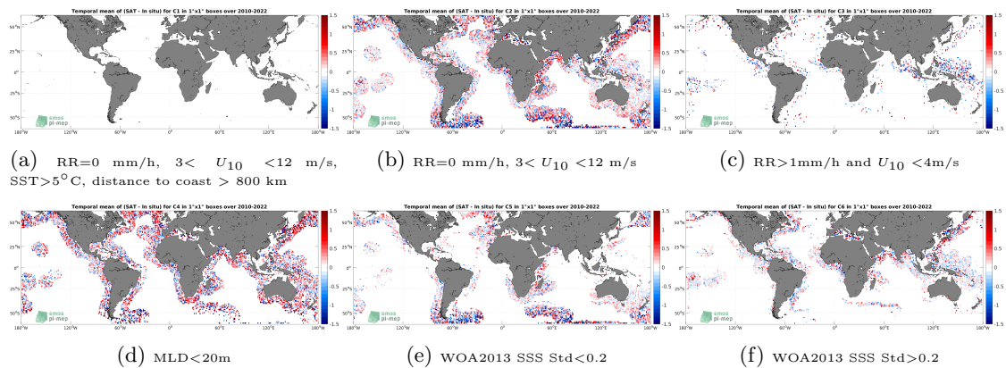
Figure 12: Temporal mean gridded over spatial boxes of size 1^\circ \times 1^\circ of \Delta SSS (SMOS SSS L2Q v330 - 0.25 Deg (CATDS-CPDC) - Argo) for 6 different subdatasets corresponding to:RR=0 mm/h, 3 < U_{10} < 12 m/s, SST >5^\circ C, distance to coast > 800 km (a), RR=0 mm/h, 3 < U_{10} < 12 m/s (b), RR >1 mm/h and U_{10} < 4 m/s (c),MLD <20 m (d),WOA2013 SSS Std <0.2 (e),WOA2013 SSS Std >0.2 (f).
