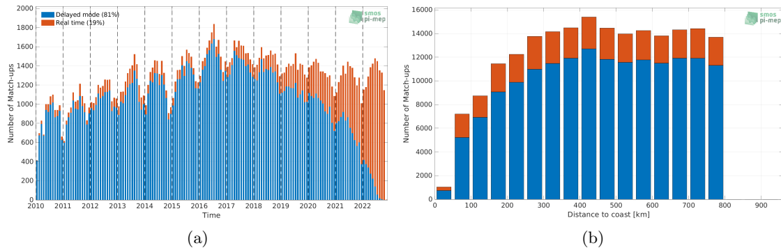
Figure 1: Number of match-ups between Argo and SMOS SSS L2Q v330 - 0.25 Deg (CATDS-CPDC) SSS as a function of time (a) and as function of the distance to coast (b) over the SMOS coastal zone (<800km) 60N-60S Pi-MEP region and for the full satellite product period.
