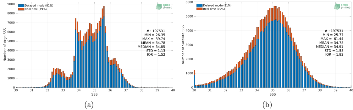
Figure 2: Histograms of SSS from Argo (a) and SMOS SSS L2Q v330 - 0.25 Deg (CATDS-CPDC) (b) considering all match-up pairs per bins of 0.1 over the SMOS coastal zone (<800km) 60N-60S Pi-MEP region and for the full satellite product period.
