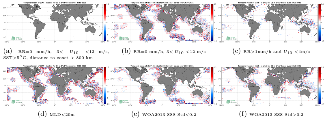
Figure 12: Temporal mean gridded over spatial boxes of size 1^\circ \times 1^\circ of \Delta SSS (SMOS SSS L2Q v330 - 0.25 Deg (CATDS-CPDC) - Argo) for 6 different subdatasets corresponding to: RR=0 mm/h, 3 < U_{10} < 12 m/s, SST > 5°C, distance to coast > 800 km (a), RR=0 mm/h, 3 < U_{10} < 12 m/s (b), RR > 1mm/h and U_{10} < 4 m/s (c), MLD < 20m (d), WOA2013 SSS Std < 0.2 (e), WOA2013 SSS Std > 0.2 (f).
