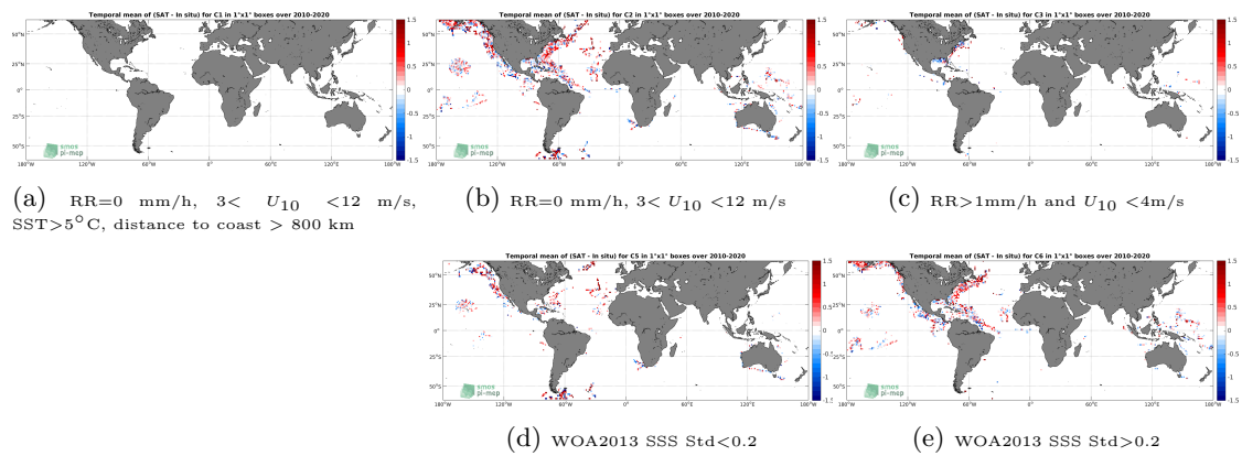
Figure 12: Temporal mean gridded over spatial boxes of size 1^\circ \times 1^\circ of \Delta\text{SSS} (SMOS SSS L2Q v321 - 0.25 Deg (CATDS-CPDC) - TSG (SAMOS)) for 5 different subdatasets corresponding to: RR=0 mm/h, 3 < U_{10} < 12 m/s, SST > 5°C, distance to coast > 800 km (a), RR=0 mm/h, 3 < U_{10} < 12 m/s (b), RR > 1mm/h and U_{10} < 4 m/s (c), WOA2013 SSS Std < 0.2 (d), WOA2013 SSS Std > 0.2 (e).
