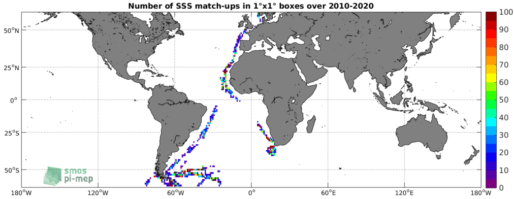
Figure 4: Number of SSS match-ups between TSG (Polarstern) SSS and the SMOS SSS L2Q v321 - 0.25 Deg (CATDS-CPDC) SSS product for the SMOS coastal zone (<800km) 60N-60S Pi-MEP region over 1^\circ \times 1^\circ boxes and for the full satellite product period.
