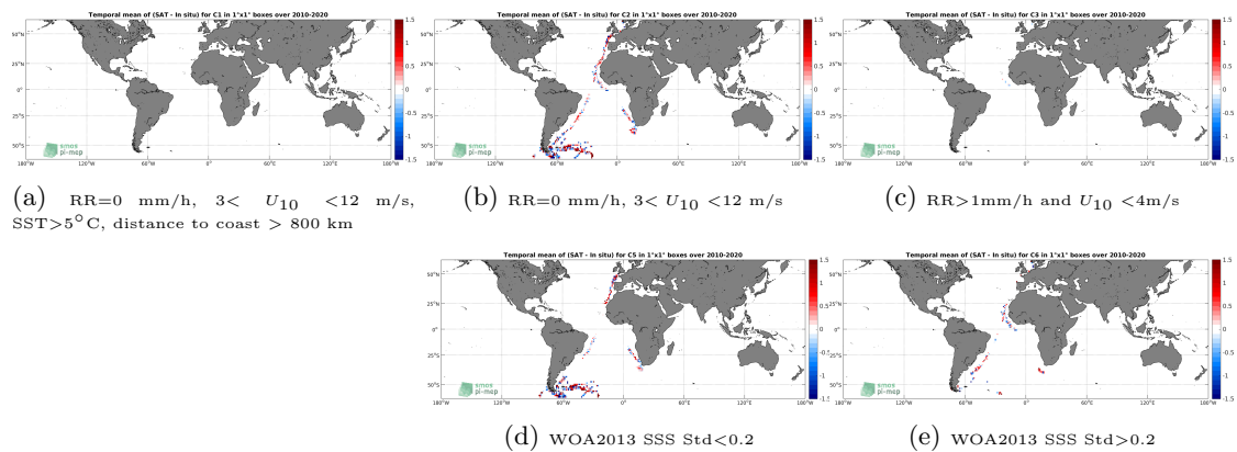
Figure 12: Temporal mean gridded over spatial boxes of size 1^\circ \times 1^\circ of \Delta SSS (SMOS SSS L2Q v321 - 0.25 Deg (CATDS-CPDC) - TSG (Polarstern)) for 5 different subdatasets corresponding to:RR=0 mm/h, 3 < U_{10} < 12 m/s, SST >5^\circ C, distance to coast > 800 km (a), RR=0 mm/h, 3 < U_{10} < 12 m/s (b), RR >1 mm/h and U_{10} < 4 m/s (c), WOA2013 SSS Std <0.2 (d), WOA2013 SSS Std >0.2 (e).
