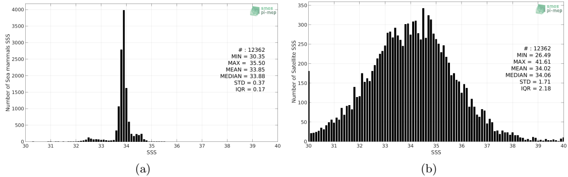
Figure 2: Histograms of SSS from Marine mammals (a) and SMOS SSS L2Q v321 - 0.25 Deg (CATDS-CPDC) (b) considering all match-up pairs per bins of 0.1 over the SMOS coastal zone (<800km) 60N-60S Pi-MEP region and for the full satellite product period.
