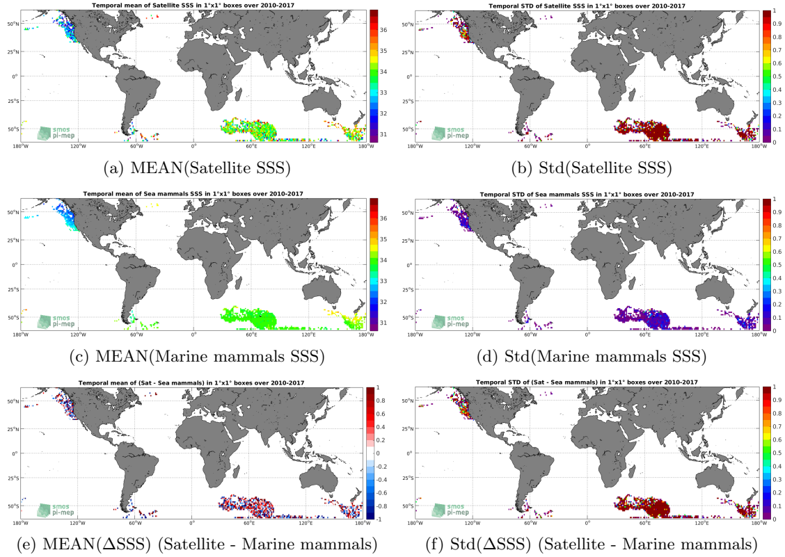
Figure 6: Temporal mean (left) and Std (right) of SSS from SMOS SSS L2Q v321 - 0.25 Deg (CATDS-CPDC) (top), Marine mammals (middle), and of \Delta SSS (Satellite - Marine mammals). Only match-up pairs are used to generate these maps.
