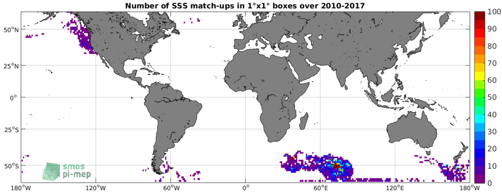
Figure 4: Number of SSS match-ups between Marine mammals SSS and the SMOS SSS L2Q v321 - 0.25 Deg (CATDS-CPDC) SSS product for the SMOS coastal zone (<800km) 60N-60S Pi-MEP region over 1^\circ \times 1^\circ boxes and for the full satellite product period.
