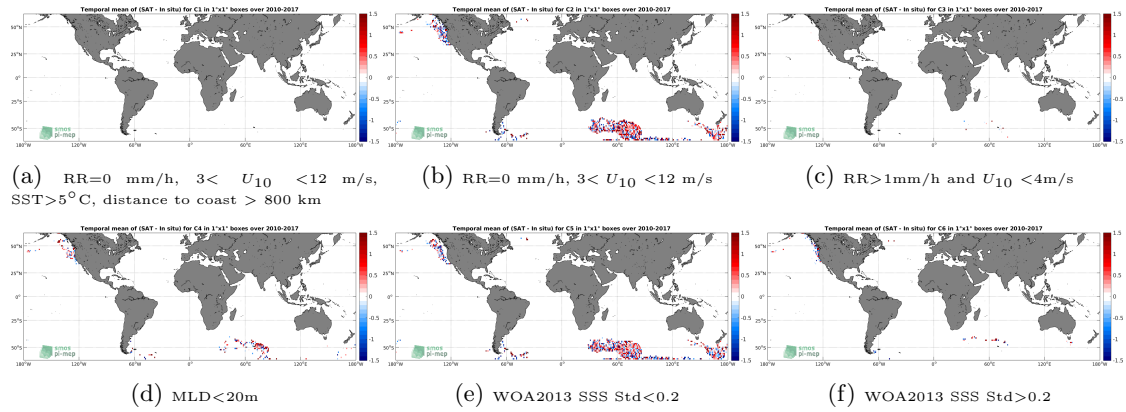
Figure 12: Temporal mean gridded over spatial boxes of size 1^\circ \times 1^\circ of \Delta SSS (SMOS SSS L2Q v321 - 0.25 Deg (CATDS-CPDC) - Marine mammals) for 6 different subdatasets corresponding to: RR=0 mm/h, 3 < U_{10} < 12 m/s, SST > 5°C, distance to coast > 800 km (a), RR=0 mm/h, 3 < U_{10} < 12 m/s (b), RR > 1mm/h and U_{10} < 4 m/s (c), MLD < 20m (d), WOA2013 SSS Std < 0.2 (e), WOA2013 SSS Std > 0.2 (f).
