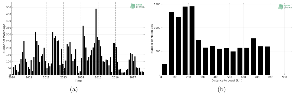
Figure 1: Number of match-ups between Marine mammals and SMOS SSS L2Q v321 - 0.25 Deg (CATDS-CPDC) SSS as a function of time (a) and as function of the distance to coast (b) over the SMOS coastal zone (<800km) 60N-60S Pi-MEP region and for the full satellite product period.
