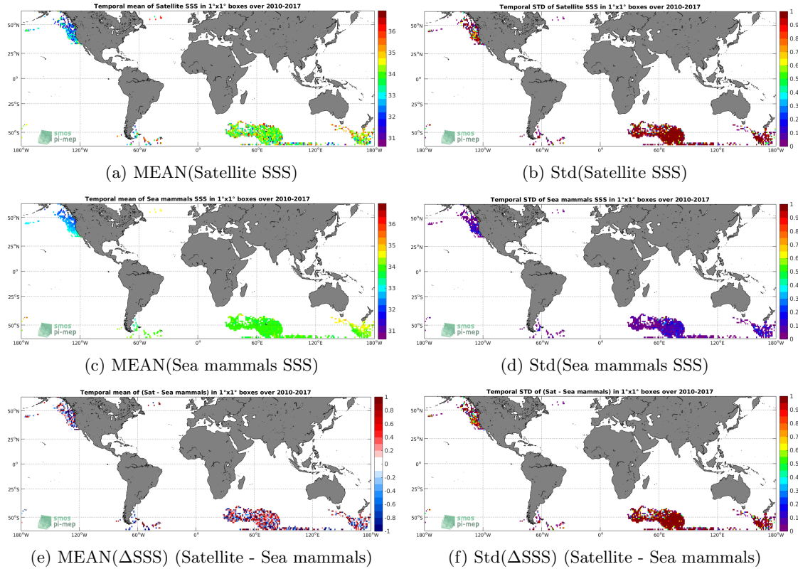
Figure 6: Temporal mean (left) and Std (right) of SSS from SMOS SSS L2Q v321 - 0.25 Deg (CATDS-CPDC) (top), Sea mammals (middle), and of \Delta SSS (Satellite - Sea mammals). Only match-up pairs are used to generate these maps.
