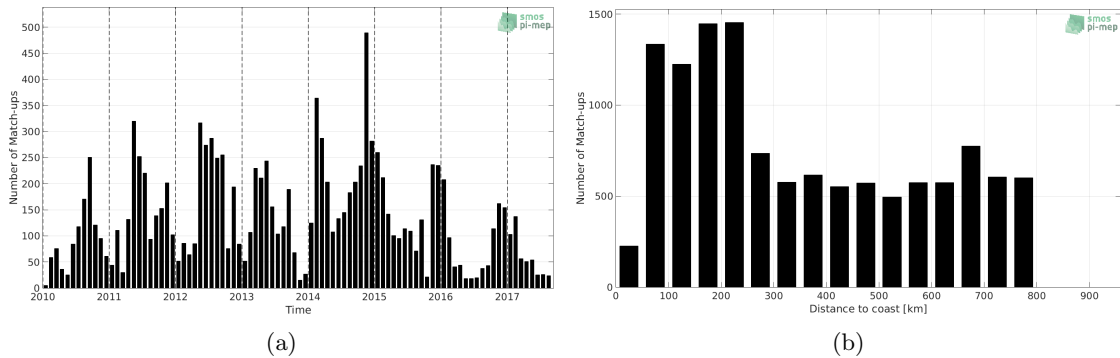
Figure 1: Number of match-ups between Sea mammals and SMOS SSS L2Q v321 - 0.25 Deg (CATDS-CPDC) SSS as a function of time (a) and as function of the distance to coast (b) over the SMOS coastal zone (<800km) 60N-60S Pi-MEP region and for the full satellite product period.
