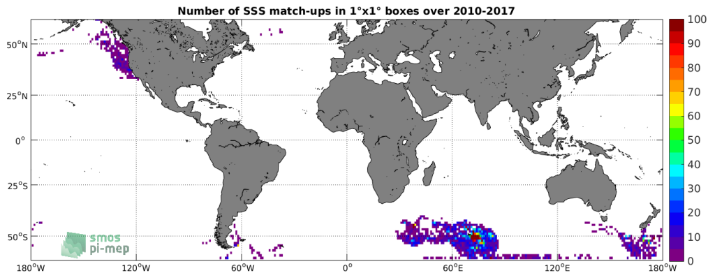
Figure 4: Number of SSS match-ups between Sea mammals SSS and the SMOS SSS L2Q v321 - 0.25 Deg (CATDS-CPDC) SSS product for the SMOS coastal zone (<800km) 60N-60S Pi-MEP region over 1°x1° boxes and for the full satellite product period.
