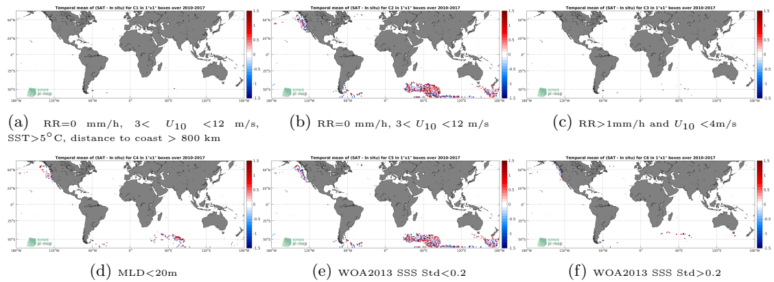
Figure 12: Temporal mean gridded over spatial boxes of size 1°x1° of \Delta SSS (SMOS SSS L2Q v321 - 0.25 Deg (CATDS-CPDC) - Sea mammals) for 6 different subdatasets corresponding to: RR=0 mm/h, 3 < U_{10} < 12 m/s, SST > 5°C, distance to coast > 800 km (a), RR=0 mm/h, 3 < U_{10} < 12 m/s (b), RR > 1mm/h and U_{10} < 4 m/s (c), MLD < 20m (d), WOA2013 SSS Std < 0.2 (e), WOA2013 SSS Std > 0.2 (f).
