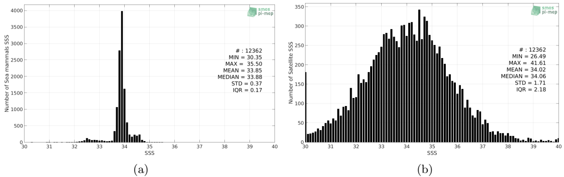
Figure 2: Histograms of SSS from Sea mammals (a) and SMOS SSS L2Q v321 - 0.25 Deg (CATDS-CPDC) (b) considering all match-up pairs per bins of 0.1 over the SMOS coastal zone (<800km) 60N-60S Pi-MEP region and for the full satellite product period.
