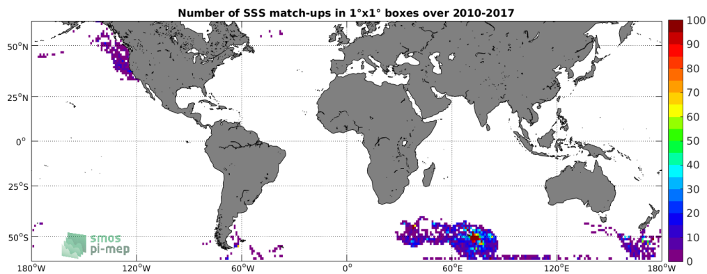
Figure 4: Number of SSS match-ups between Sea mammals SSS and the SMOS L2Q v321 - 0.25 Deg (CATDS-CPDC) SSS product for the SMOS coastal zone (<800km) 60N-60S Pi-MEP region over 1°x1° boxes and for the full satellite product period.
