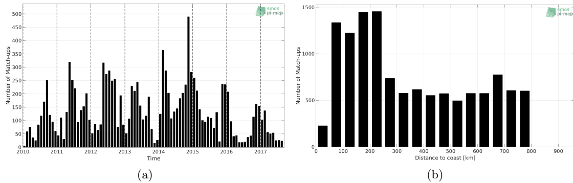
Figure 1: Number of match-ups between Sea mammals and SMOS L2Q v321 - 0.25 Deg (CATDS-CPDC) SSS as a function of time (a) and as function of the distance to coast (b) over the SMOS coastal zone (<800km) 60N-60S Pi-MEP region and for the full satellite product period.
