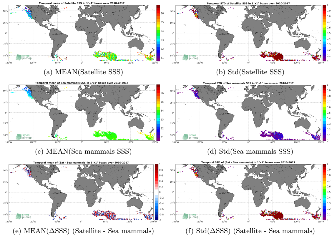
Figure 6: Temporal mean (left) and Std (right) of SSS from SMOS L2Q v321 - 0.25 Deg (CATDS-CPDC) (top), Sea mammals (middle), and of \Delta SSS (Satellite - Sea mammals). Only match-up pairs are used to generate these maps.
