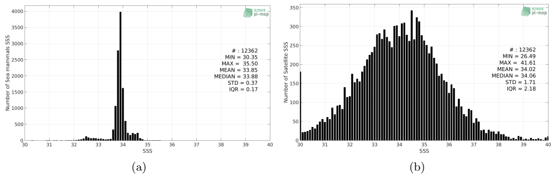
Figure 2: Histograms of SSS from Sea mammals (a) and SMOS L2Q v321 - 0.25 Deg (CATDS-CPDC) (b) considering all match-up pairs per bins of 0.1 over the SMOS coastal zone (<800km) 60N-60S Pi-MEP region and for the full satellite product period.
