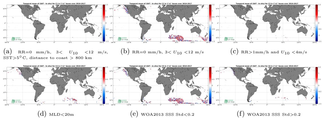
Figure 12: Temporal mean gridded over spatial boxes of size 1^\circ \times 1^\circ of \Delta SSS (SMOS L2Q v321 - 0.25 Deg (CATDS-CPDC) - Sea mammals) for 6 different subdatasets corresponding to:RR=0 mm/h, 3 < U_{10} < 12 m/s, SST >5^\circ C, distance to coast > 800 km (a), RR=0 mm/h, 3 < U_{10} < 12 m/s (b), RR >1 mm/h and U_{10} < 4 m/s (c),MLD <20 m (d),WOA2013 SSS Std <0.2 (e),WOA2013 SSS Std >0.2 (f).
