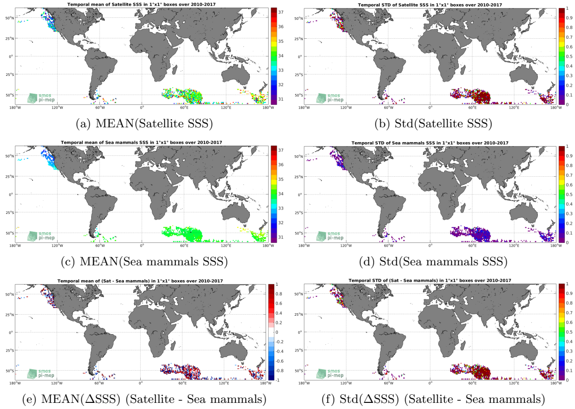
Figure 6: Temporal mean (left) and Std (right) of SSS from SMOS-L3-CATDS-CPDC-V321-L2Q (top), Sea mammals (middle), and of \Delta SSS (Satellite - Sea mammals). Only match-up pairs are used to generate these maps.
