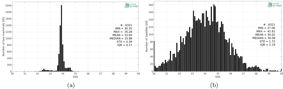
Figure 2: Histograms of SSS from Sea mammals (a) and SMOS-L3-CATDS-CPDC-V321-L2Q (b) considering all match-up pairs per bins of 0.1 over the SMOS coastal zone ( \geq 800\text{km} ) 60N-60S Pi-MEP region and for the full satellite product period.
