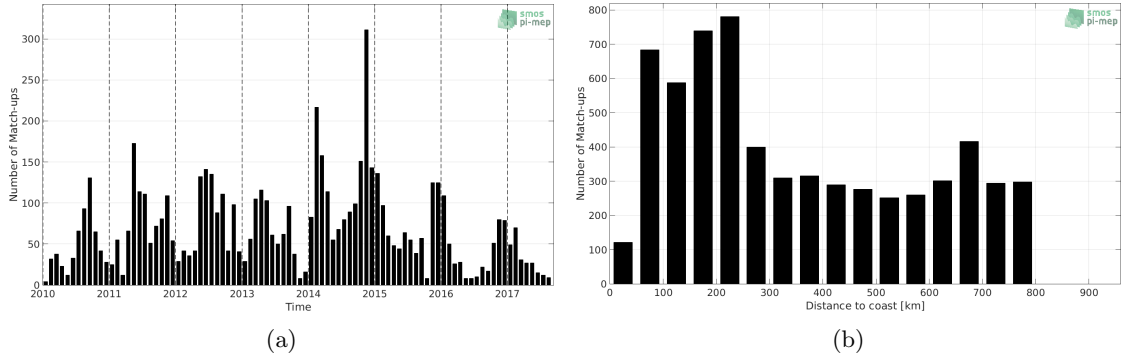
Figure 1: Number of match-ups between Sea mammals and SMOS-L3-CATDS-CPDC-V321-L2Q SSS as a function of time (a) and as function of the distance to coast (b) over the SMOS coastal zone ( \geq 800\text{km} ) 60N-60S Pi-MEP region and for the full satellite product period.
