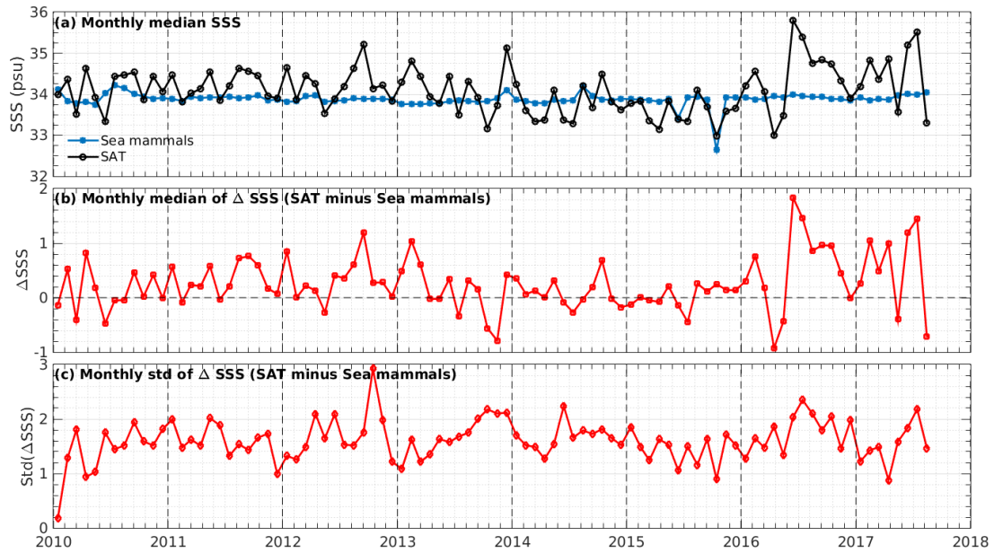
Figure 7: Time series of the monthly median SSS (top), median of \Delta SSS (Satellite - Sea mammals) and Std of \Delta SSS (Satellite - Sea mammals) over the SMOS coastal zone ( \geq 800 km) 60N-60S Pi-MEP region considering all match-ups collected by the Pi-MEP.
