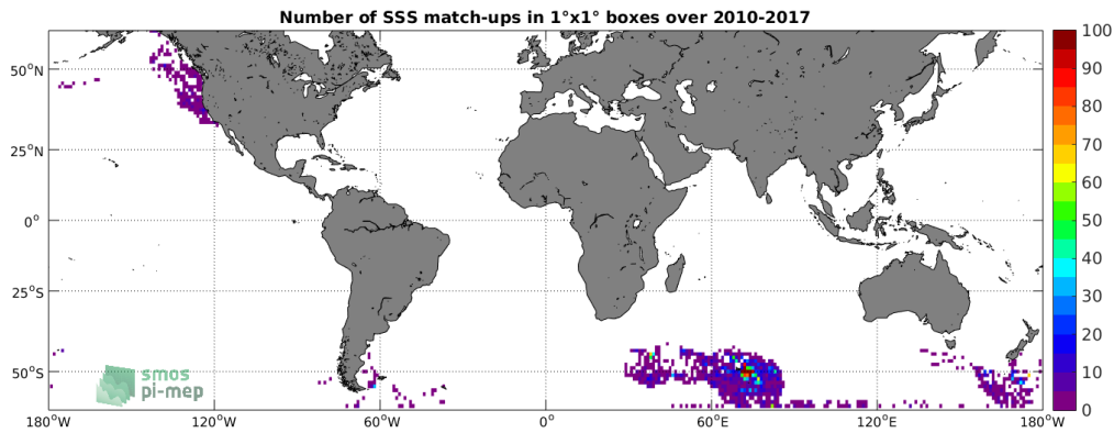
Figure 4: Number of SSS match-ups between Sea mammals SSS and the SMOS-L3-CATDS-CPDC-V321-L2Q SSS product for the SMOS coastal zone ( \pm 800\text{km} ) 60N-60S Pi-MEP region over 1^\circ \times 1^\circ boxes and for the full satellite product period.
