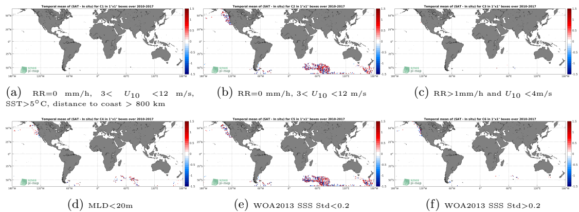
Figure 12: Temporal mean gridded over spatial boxes of size 1^\circ \times 1^\circ of \Delta SSS (SMOS-L3-CATDS-CPDC-V321-L2Q - Sea mammals) for 6 different subdatasets corresponding to:RR=0 mm/h, 3 < U_{10} < 12 m/s, SST >5^\circ C, distance to coast > 800 km (a), RR=0 mm/h, 3 < U_{10} < 12 m/s (b), RR >1 mm/h and U_{10} < 4 m/s (c),MLD <20 m (d),WOA2013 SSS Std <0.2 (e),WOA2013 SSS Std >0.2 (f).
