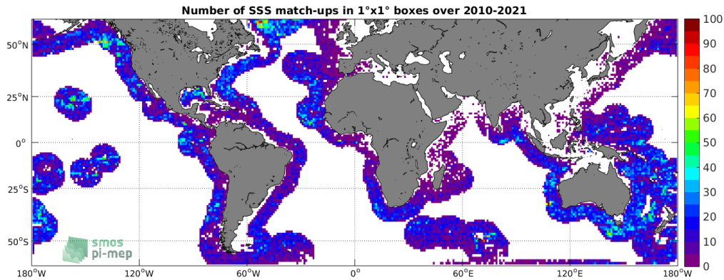
Figure 4: Number of SSS match-ups between Argo SSS and the SMOS SSS L2Q v321 - 0.25 Deg (CATDS-CPDC) SSS product for the SMOS coastal zone (<800km) 60N-60S Pi-MEP region over 1°x1° boxes and for the full satellite product period.
