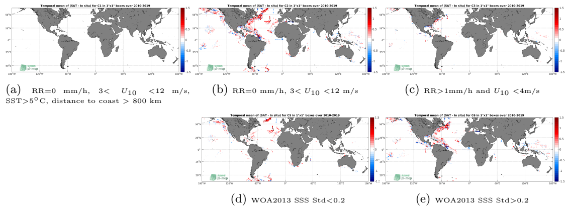
Figure 12: Temporal mean gridded over spatial boxes of size 1^\circ \times 1^\circ of \Delta SSS (SMOS-L3-CATDS-CPDC-V317-MONTHLY-25KM - TSG-SAMOS) for 5 different subdatasets corresponding to:RR=0 mm/h, 3 < U_{10} < 12 m/s, SST >5^\circ C, distance to coast > 800 km (a), RR=0 mm/h, 3 < U_{10} < 12 m/s (b), RR >1 mm/h and U_{10} < 4 m/s (c), WOA2013 SSS Std <0.2 (d), WOA2013 SSS Std >0.2 (e).
