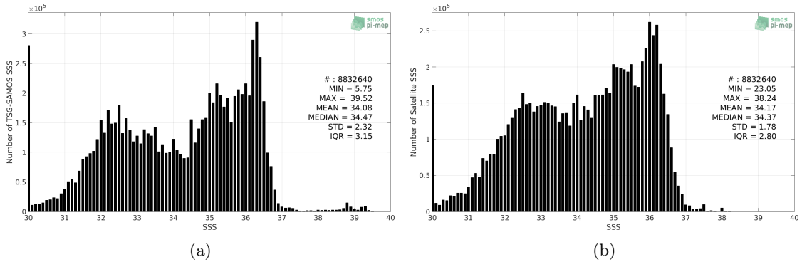
Figure 2: Histograms of SSS from TSG-SAMOS (a) and SMOS-L3-CATDS-CPDC-V317-MONTHLY-25KM (b) considering all match-up pairs per bins of 0.1 over the SMOS coastal zone ( \approx 800 km) 60N-60S Pi-MEP region and for the full satellite product period.
