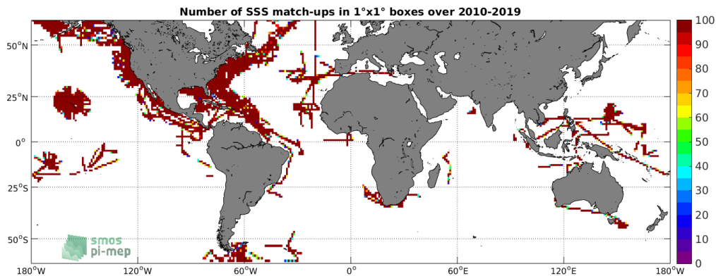
Figure 4: Number of SSS match-ups between TSG-SAMOS SSS and the SMOS-L3-CATDS-CPDC-V317-MONTHLY-25KM SSS product for the SMOS coastal zone ( \approx 800 km) 60N-60S Pi-MEP region over 1^\circ \times 1^\circ boxes and for the full satellite product period.
