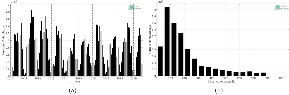
Figure 1: Number of match-ups between TSG-SAMOS and SMOS-L3-CATDS-CPDC-V317-MONTHLY-25KM SSS as a function of time (a) and as function of the distance to coast (b) over the SMOS coastal zone ( \approx 800 km) 60N-60S Pi-MEP region and for the full satellite product period.
