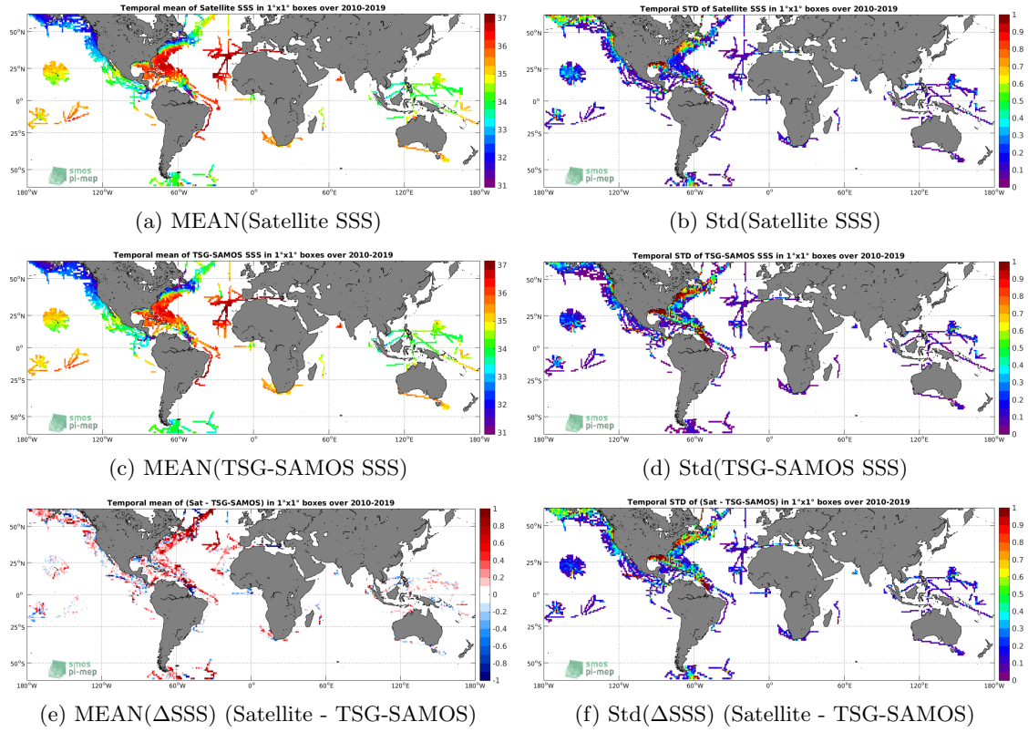
Figure 6: Temporal mean (left) and Std (right) of SSS from SMOS-L3-CATDS-CPDC-V317-MONTHLY-25KM (top), TSG-SAMOS (middle), and of \Delta SSS (Satellite - TSG-SAMOS). Only match-up pairs are used to generate these maps.
