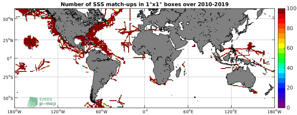
Figure 4: Number of SSS match-ups between TSG-SAMOS SSS and the SMOS-L3-CATDS-CPDC-V317-MONTHLY-25KM SSS product for the SMOS coastal zone ( \approx 800\text{km} ) 60N-60S Pi-MEP region over 1^\circ \times 1^\circ boxes and for the full satellite product period.
