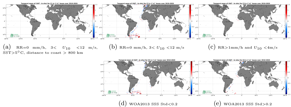
Figure 12: Temporal mean gridded over spatial boxes of size 1^\circ \times 1^\circ of \Delta SSS (SMOS SSS L3 v317 - Monthly - 25 km (CATDS-CPDC) - TSG (Polarstern)) for 5 different subdatasets corresponding to: RR=0 mm/h, 3 < U_{10} < 12 m/s, SST > 5^\circ\text{C} , distance to coast > 800 km (a), RR=0 mm/h, 3 < U_{10} < 12 m/s (b), RR > 1 mm/h and U_{10} < 4 m/s (c), WOA2013 SSS Std < 0.2 (d), WOA2013 SSS Std > 0.2 (e).
