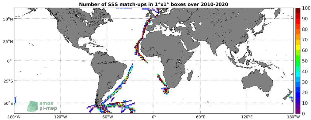
Figure 4: Number of SSS match-ups between TSG (Polarstern) SSS and the SMOS SSS L3 v317 - Monthly - 25 km (CATDS-CPDC) SSS product for the SMOS coastal zone (<800km) 60N-60S Pi-MEP region over 1°x1° boxes and for the full satellite product period.
