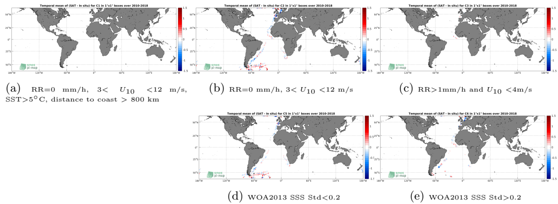
Figure 12: Temporal mean gridded over spatial boxes of size 1^\circ \times 1^\circ of \Delta SSS (SMOS-L3-CATDS-CPDC-V317-MONTHLY-25KM - TSG-POLARSTERN) for 5 different subdatasets corresponding to:RR=0 mm/h, 3 < U_{10} < 12 m/s, SST >5^\circ C, distance to coast > 800 km (a), RR=0 mm/h, 3 < U_{10} < 12 m/s (b), RR >1 mm/h and U_{10} < 4 m/s (c), WOA2013 SSS Std <0.2 (d), WOA2013 SSS Std >0.2 (e).
