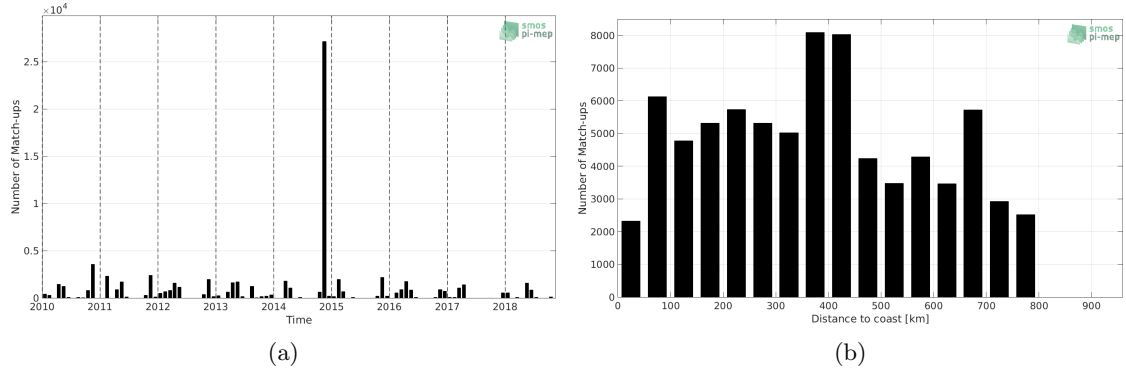
Figure 1: Number of match-ups between TSG-POLARSTERN and SMOS-L3-CATDS-CPDC-V317-MONTHLY-25KM SSS as a function of time (a) and as function of the distance to coast (b) over the SMOS coastal zone ( \approx 800 km) 60N-60S Pi-MEP region and for the full satellite product period.
