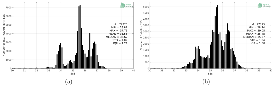
Figure 2: Histograms of SSS from TSG-POLARSTERN (a) and SMOS-L3-CATDS-CPDC-V317-MONTHLY-25KM (b) considering all match-up pairs per bins of 0.1 over the SMOS coastal zone ( \approx 800 km) 60N-60S Pi-MEP region and for the full satellite product period.
