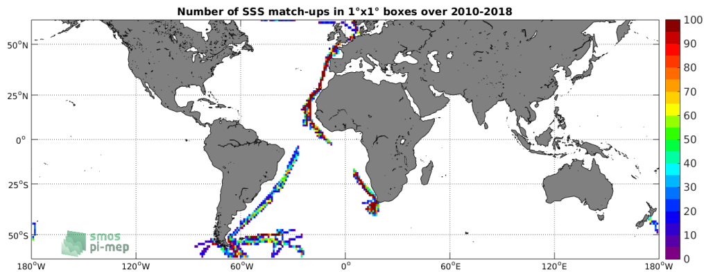
Figure 4: Number of SSS match-ups between TSG-POLARSTERN SSS and the SMOS-L3-CATDS-CPDC-V317-MONTHLY-25KM SSS product for the SMOS coastal zone ( \pm 800\text{km} ) 60N-60S Pi-MEP region over 1^\circ \times 1^\circ boxes and for the full satellite product period.
