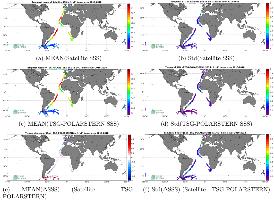
Figure 6: Temporal mean (left) and Std (right) of SSS from SMOS-L3-CATDS-CPDC-V317-MONTHLY-25KM (top), TSG-POLARSTERN (middle), and of \Delta SSS (Satellite - TSG-POLARSTERN). Only match-up pairs are used to generate these maps.
