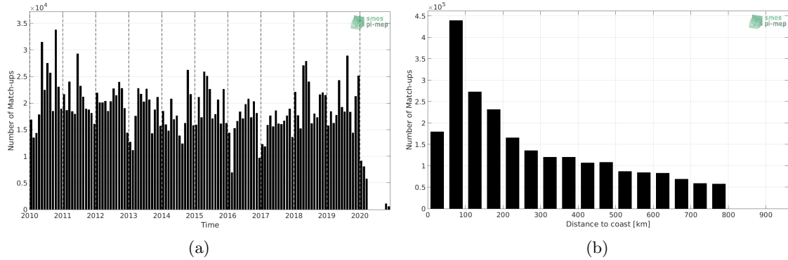
Figure 1: Number of match-ups between TSG (LEGOS-DM) and SMOS SSS L3 v317 - Monthly - 25 km (CATDS-CPDC) SSS as a function of time (a) and as function of the distance to coast (b) over the SMOS coastal zone (<800km) 60N-60S Pi-MEP region and for the full satellite product period.
