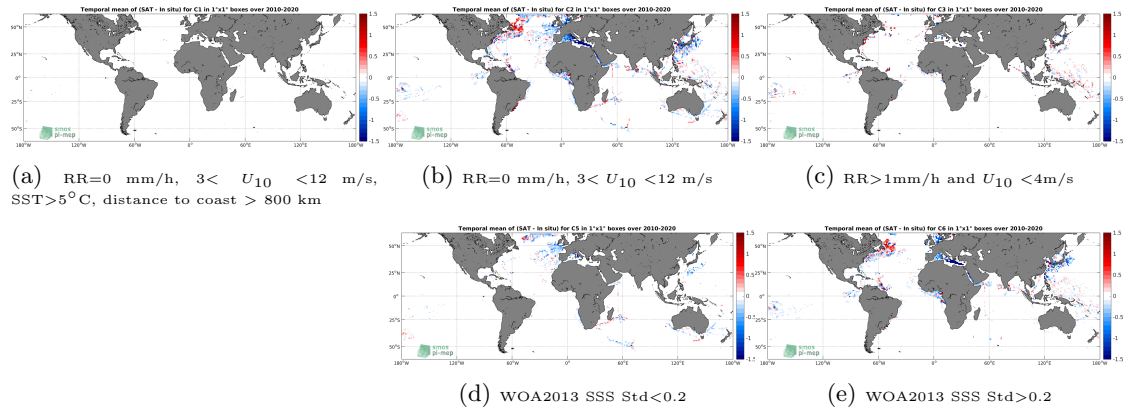
Figure 12: Temporal mean gridded over spatial boxes of size 1^\circ \times 1^\circ of \Delta SSS (SMOS SSS L3 v317 - Monthly - 25 km (CATDS-CPDC) - TSG (LEGOS-DM)) for 5 different subdatasets corresponding to:RR=0 mm/h, 3 < U_{10} < 12 m/s, SST >5^\circ\text{C} , distance to coast > 800 km (a), RR=0 mm/h, 3 < U_{10} < 12 m/s (b), RR >1 mm/h and U_{10} < 4 m/s (c), WOA2013 SSS Std <0.2 (d), WOA2013 SSS Std >0.2 (e).
