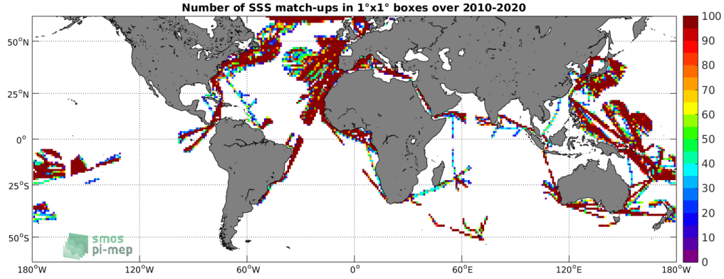
Figure 4: Number of SSS match-ups between TSG (LEGOS-DM) SSS and the SMOS SSS L3 v317 - Monthly - 25 km (CATDS-CPDC) SSS product for the SMOS coastal zone ( <800\text{km} ) 60N-60S Pi-MEP region over 1^\circ \times 1^\circ boxes and for the full satellite product period.
