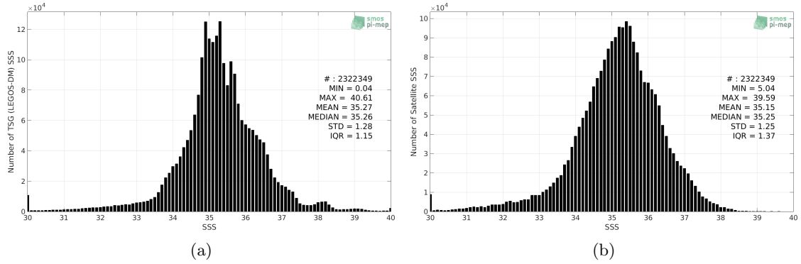
Figure 2: Histograms of SSS from TSG (LEGOS-DM) (a) and SMOS SSS L3 v317 - Monthly - 25 km (CATDS-CPDC) (b) considering all match-up pairs per bins of 0.1 over the SMOS coastal zone (<800km) 60N-60S Pi-MEP region and for the full satellite product period.
