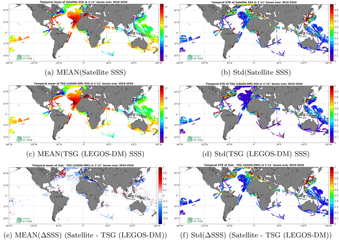
Figure 6: Temporal mean (left) and Std (right) of SSS from SMOS SSS L3 v317 - Monthly - 25 km (CATDS-CPDC) (top), TSG (LEGOS-DM) (middle), and of \Delta SSS (Satellite - TSG (LEGOS-DM)). Only match-up pairs are used to generate these maps.
