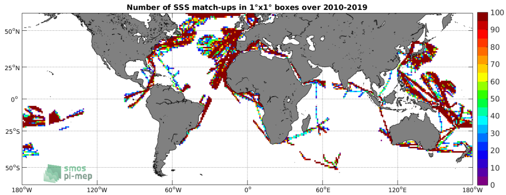
Figure 4: Number of SSS match-ups between TSG-LEGOS-DM SSS and the SMOS L3 v317 - Monthly - 25 km (CATDS-CPDC) SSS product for the SMOS coastal zone (<800km) 60N-60S Pi-MEP region over 1^\circ \times 1^\circ boxes and for the full satellite product period.
