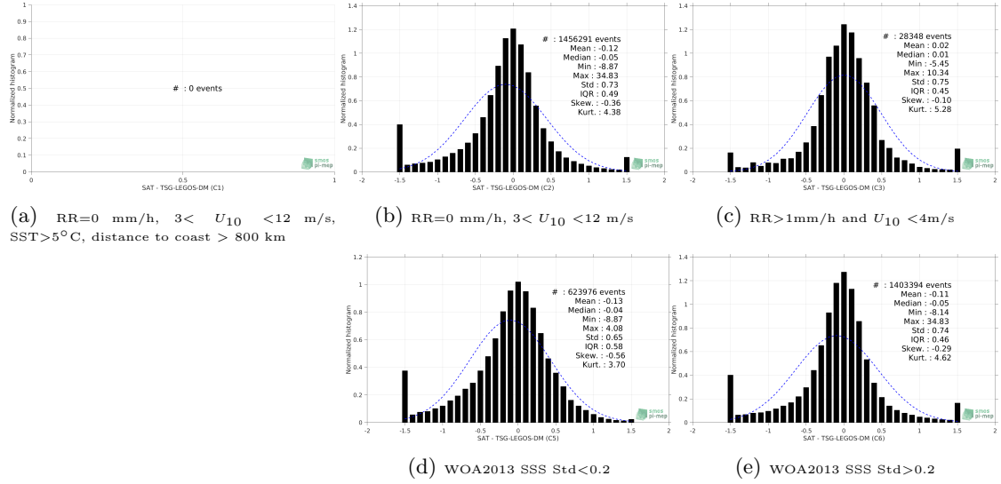
Figure 13: Normalized histogram of \Delta SSS (SMOS L3 v317 - Monthly - 25 km (CATDS-CPDC) - TSG-LEGOS-DM) for 5 different subdatasets corresponding to: RR=0 mm/h, 3 < U_{10} < 12 m/s, SST > 5^\circ C , distance to coast > 800 km (a), RR=0 mm/h, 3 < U_{10} < 12 m/s (b), RR > 1 mm/h and U_{10} < 4 m/s (c), WOA2013 SSS Std < 0.2 (d), WOA2013 SSS Std > 0.2 (e).
