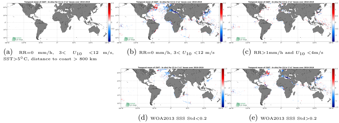
Figure 12: Temporal mean gridded over spatial boxes of size 1^\circ \times 1^\circ of \Delta SSS (SMOS L3 v317 - Monthly - 25 km (CATDS-CPDC) - TSG-LEGOS-DM) for 5 different subdatasets corresponding to: RR=0 mm/h, 3 < U_{10} < 12 m/s, SST > 5^\circ\text{C} , distance to coast > 800 km (a), RR=0 mm/h, 3 < U_{10} < 12 m/s (b), RR > 1 mm/h and U_{10} < 4 m/s (c), WOA2013 SSS Std < 0.2 (d), WOA2013 SSS Std > 0.2 (e).
