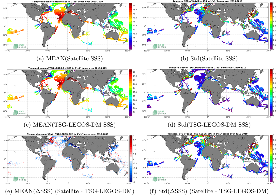
Figure 6: Temporal mean (left) and Std (right) of SSS from SMOS L3 v317 - Monthly - 25 km (CATDS-CPDC) (top), TSG-LEGOS-DM (middle), and of \Delta SSS (Satellite - TSG-LEGOS-DM). Only match-up pairs are used to generate these maps.
