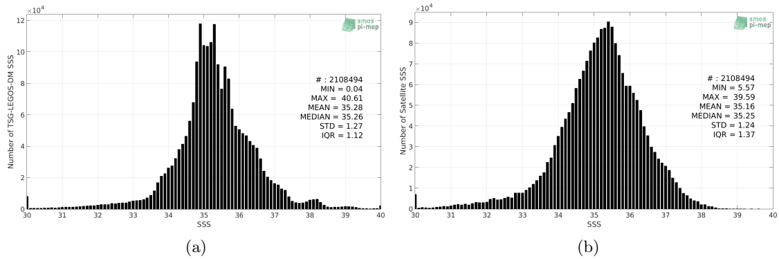
Figure 2: Histograms of SSS from TSG-LEGOS-DM (a) and SMOS L3 v317 - Monthly - 25 km (CATDS-CPDC) (b) considering all match-up pairs per bins of 0.1 over the SMOS coastal zone (<800km) 60N-60S Pi-MEP region and for the full satellite product period.
