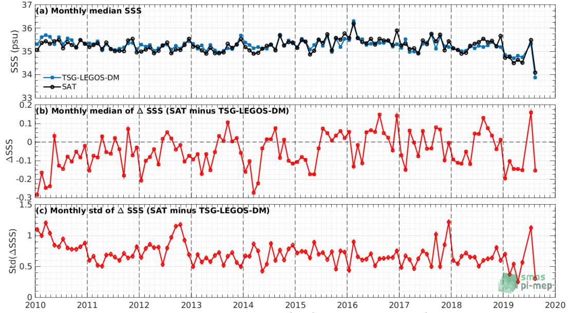
Figure 7: Time series of the monthly median SSS (top), median of \Delta SSS (Satellite - TSG-LEGOS-DM) and Std of \Delta SSS (Satellite - TSG-LEGOS-DM) over the SMOS coastal zone ( <800\text{km} ) 60N-60S Pi-MEP region considering all match-ups collected by the Pi-MEP.
