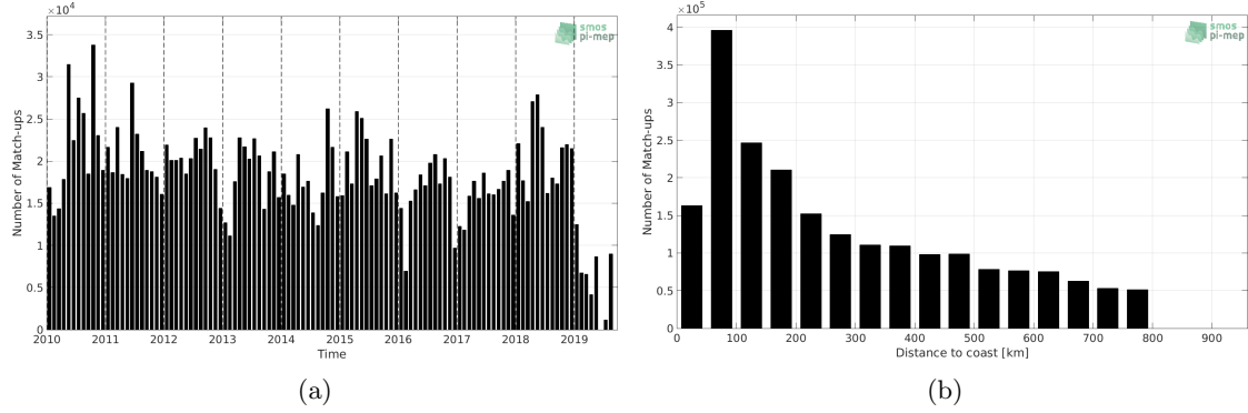
Figure 1: Number of match-ups between TSG-LEGOS-DM and SMOS L3 v317 - Monthly - 25 km (CATDS-CPDC) SSS as a function of time (a) and as function of the distance to coast (b) over the SMOS coastal zone (<800km) 60N-60S Pi-MEP region and for the full satellite product period.
