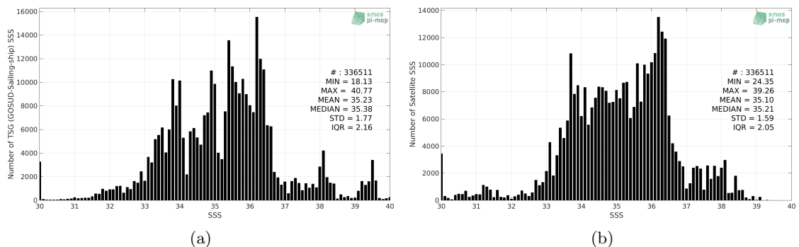
Figure 2: Histograms of SSS from TSG (GOSUD-Sailing-ship) (a) and SMOS SSS L3 v317 - Monthly - 25 km (CATDS-CPDC) (b) considering all match-up pairs per bins of 0.1 over the SMOS coastal zone (<800km) 60N-60S Pi-MEP region and for the full satellite product period.
