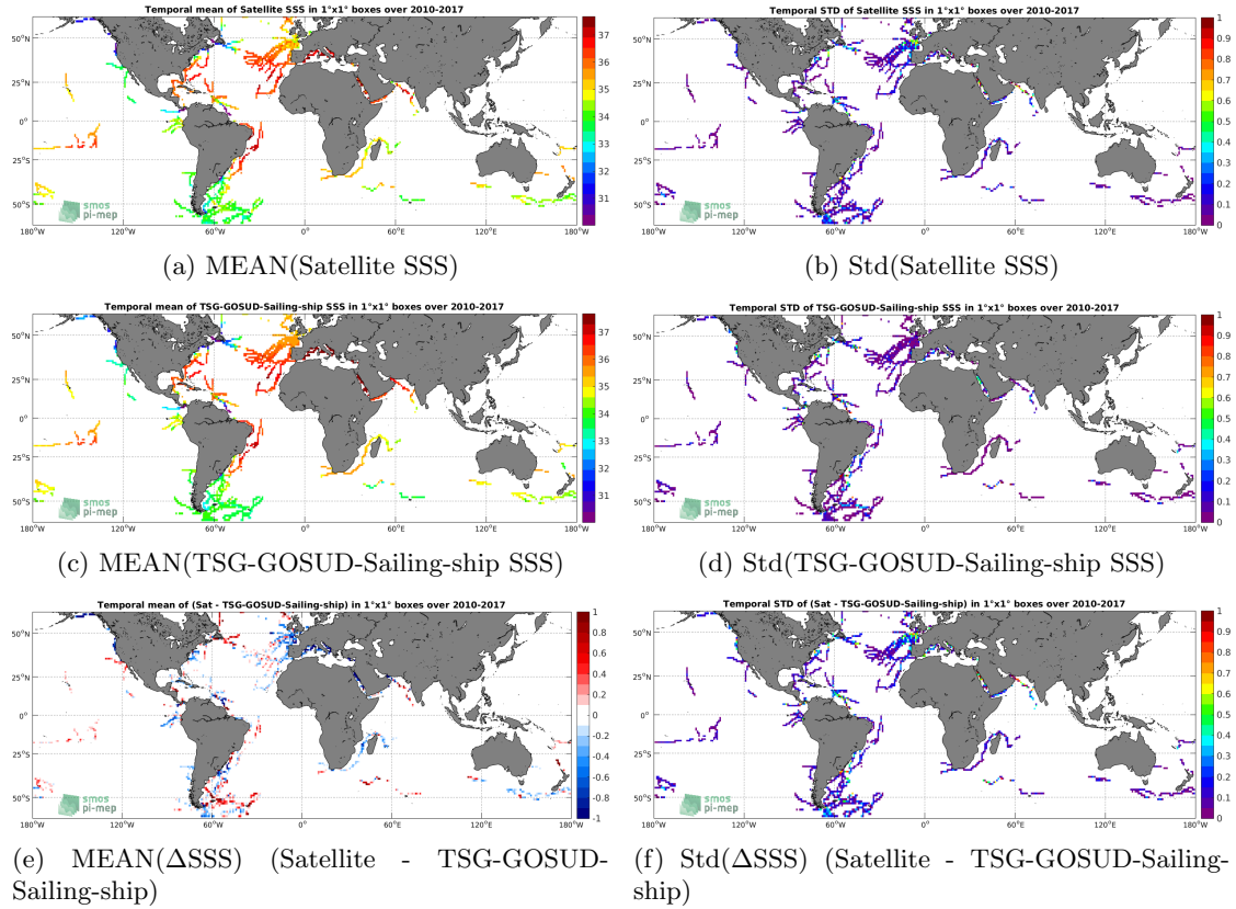
Figure 6: Temporal mean (left) and Std (right) of SSS from SMOS-L3-CATDS-CPDC-V317-MONTHLY-25KM (top), TSG-GOSUD-Sailing-ship (middle), and of \Delta SSS (Satellite - TSG-GOSUD-Sailing-ship). Only match-up pairs are used to generate these maps.
