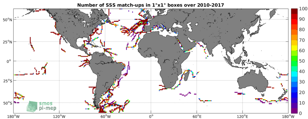
Figure 4: Number of SSS match-ups between TSG-GOSUD-Sailing-ship SSS and the SMOS-L3-CATDS-CPDC-V317-MONTHLY-25KM SSS product for the SMOS coastal zone ( \pm 800\text{km} ) 60N-60S Pi-MEP region over 1^\circ \times 1^\circ boxes and for the full satellite product period.
