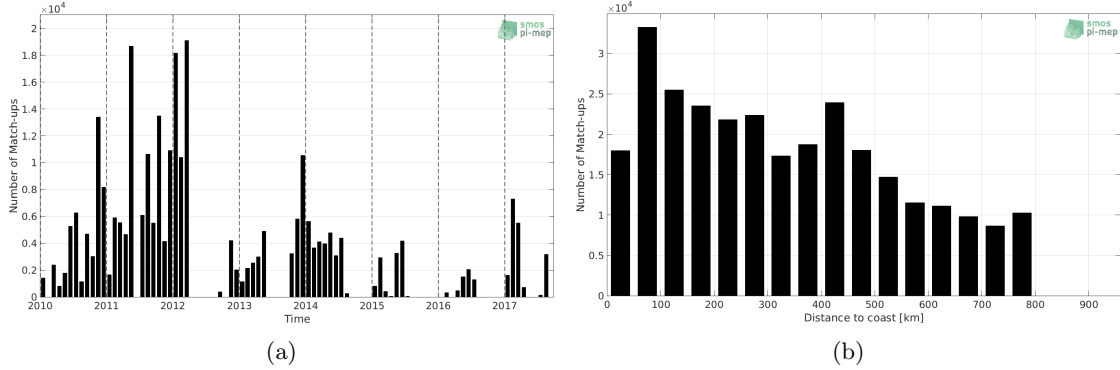
Figure 1: Number of match-ups between TSG-GOSUD-Sailing-ship and SMOS-L3-CATDS-CPDC-V317-MONTHLY-25KM SSS as a function of time (a) and as function of the distance to coast (b) over the SMOS coastal zone ( \approx 800 km) 60N-60S Pi-MEP region and for the full satellite product period.
