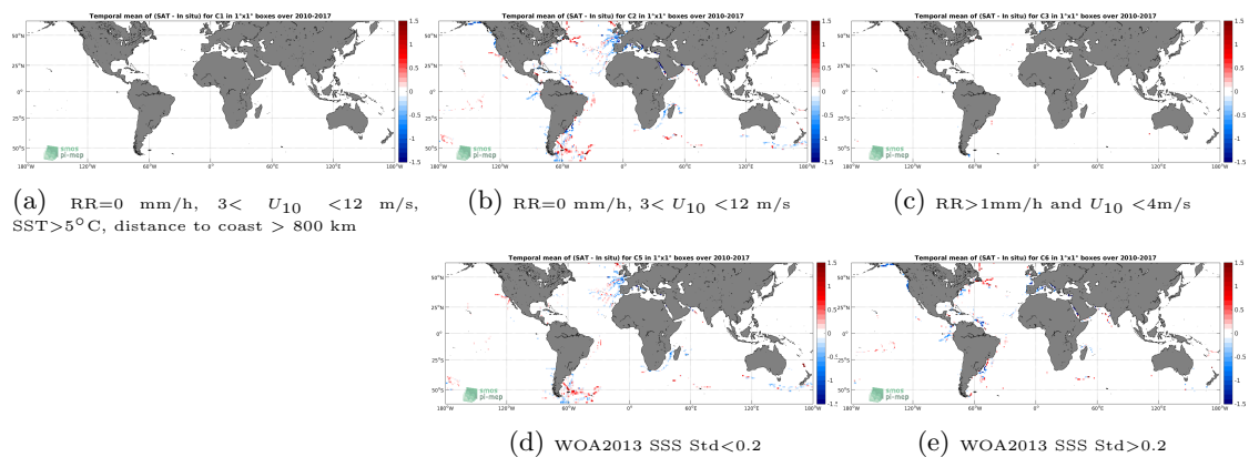
Figure 12: Temporal mean gridded over spatial boxes of size 1^\circ \times 1^\circ of \Delta SSS (SMOS-L3-CATDS-CPDC-V317-MONTHLY-25KM - TSG-GOSUD-Sailing-ship) for 5 different subdatasets corresponding to:RR=0 mm/h, 3 < U_{10} < 12 m/s, SST >5^\circ C, distance to coast > 800 km (a), RR=0 mm/h, 3 < U_{10} < 12 m/s (b), RR >1 mm/h and U_{10} < 4 m/s (c), WOA2013 SSS Std <0.2 (d), WOA2013 SSS Std >0.2 (e).
