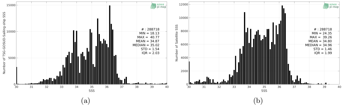
Figure 2: Histograms of SSS from TSG-GOSUD-Sailing-ship (a) and SMOS-L3-CATDS-CPDC-V317-MONTHLY-25KM (b) considering all match-up pairs per bins of 0.1 over the SMOS coastal zone ( \approx 800 km) 60N-60S Pi-MEP region and for the full satellite product period.
