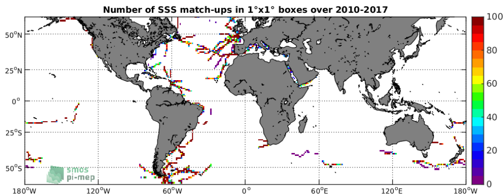
Figure 4: Number of SSS match-ups between TSG-GOSUD-Sailing-ship SSS and the SMOS-L3-CATDS-CPDC-V317-MONTHLY-25KM SSS product for the SMOS coastal zone ( \approx 800\text{km} ) 60N-60S Pi-MEP region over 1^\circ \times 1^\circ boxes and for the full satellite product period.
