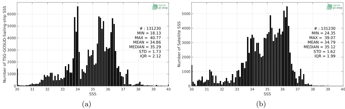
Figure 2: Histograms of SSS from TSG-GOSUD-Sailing-ship (a) and SMOS-L3-CATDS-CPDC-V317-MONTHLY-25KM (b) considering all match-up pairs per bins of 0.1 over the SMOS coastal zone ( \approx 800 km) 60N-60S Pi-MEP region and for the full satellite product period.
