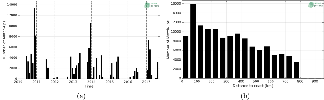
Figure 1: Number of match-ups between TSG-GOSUD-Sailing-ship and SMOS-L3-CATDS-CPDC-V317-MONTHLY-25KM SSS as a function of time (a) and as function of the distance to coast (b) over the SMOS coastal zone ( \approx 800 km) 60N-60S Pi-MEP region and for the full satellite product period.
