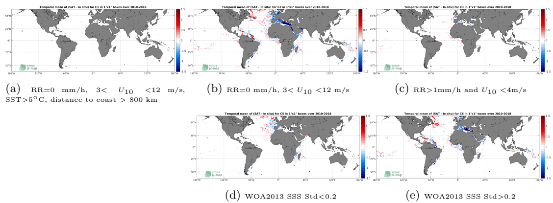
Figure 12: Temporal mean gridded over spatial boxes of size 1^\circ \times 1^\circ of \Delta SSS (SMOS SSS L3 v317 - Monthly - 25 km (CATDS-CPDC) - TSG (GOSUD-Research-vessel)) for 5 different subdatasets corresponding to:RR=0 mm/h, 3 < U_{10} < 12 m/s, SST>5°C, distance to coast > 800 km (a), RR=0 mm/h, 3 < U_{10} < 12 m/s (b), RR>1mm/h and U_{10} < 4 m/s (c), WOA2013 SSS Std<0.2 (d), WOA2013 SSS Std>0.2 (e).
