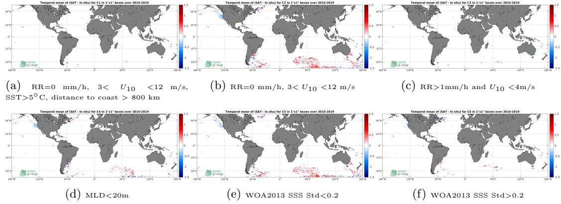
Figure 12: Temporal mean gridded over spatial boxes of size 1^\circ \times 1^\circ of \Delta SSS (SMOS SSS L3 v317 - Monthly - 25 km (CATDS-CPDC) - Marine mammals) for 6 different subdatasets corresponding to: RR=0 mm/h, 3 < U_{10} < 12 m/s, SST > 5^\circ C , distance to coast > 800 km (a), RR=0 mm/h, 3 < U_{10} < 12 m/s (b), RR > 1 mm/h and U_{10} < 4 m/s (c), MLD < 20 m (d), WOA2013 SSS Std < 0.2 (e), WOA2013 SSS Std > 0.2 (f).
