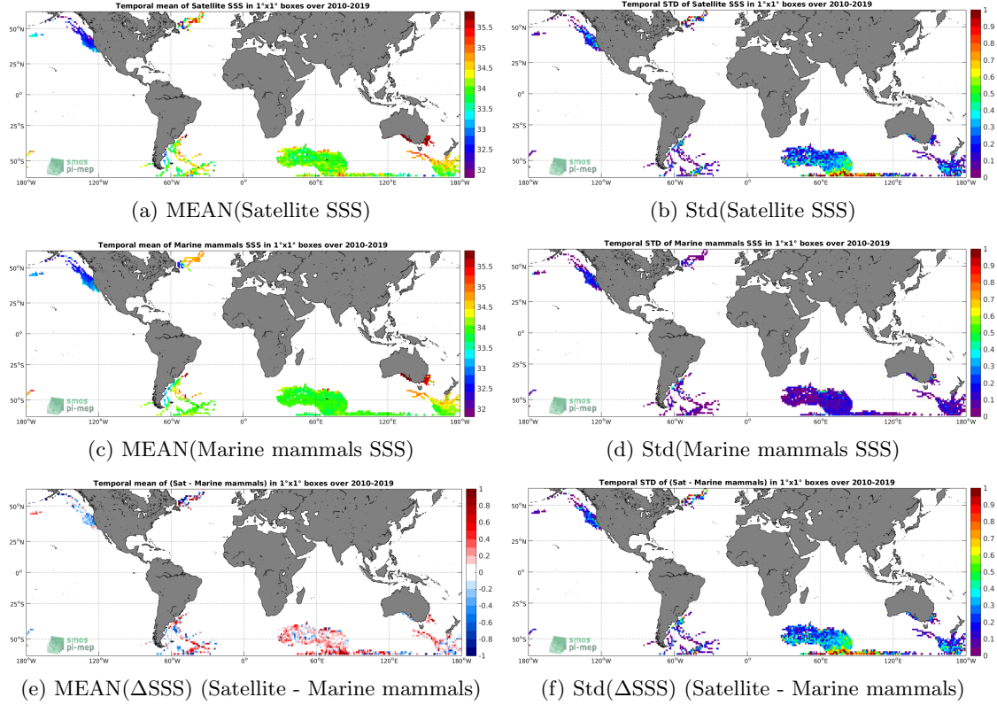
Figure 6: Temporal mean (left) and Std (right) of SSS from SMOS SSS L3 v317 - Monthly - 25 km (CATDS-CPDC) (top), Marine mammals (middle), and of \Delta SSS (Satellite - Marine mammals). Only match-up pairs are used to generate these maps.
