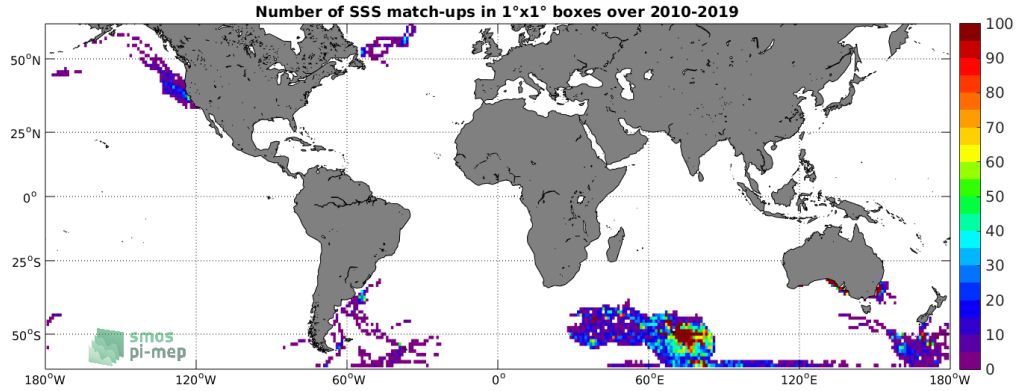
Figure 4: Number of SSS match-ups between Marine mammals SSS and the SMOS SSS L3 v317 - Monthly - 25 km (CATDS-CPDC) SSS product for the SMOS coastal zone (<800km) 60N-60S Pi-MEP region over 1^\circ \times 1^\circ boxes and for the full satellite product period.
