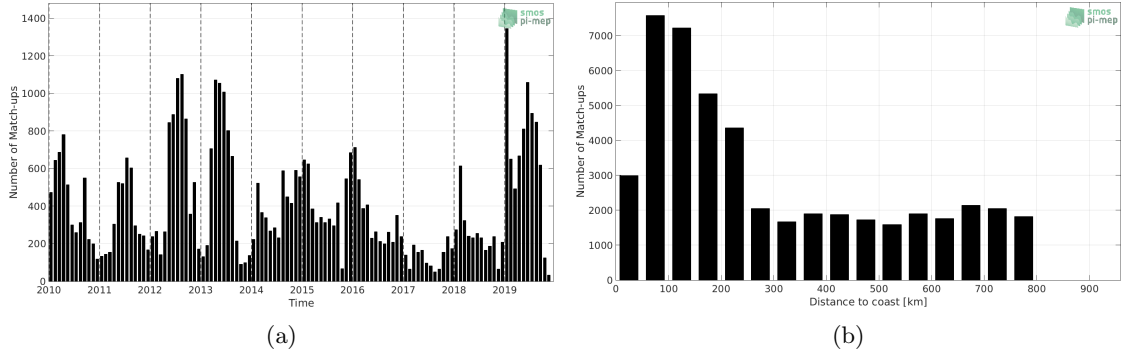
Figure 1: Number of match-ups between Marine mammals and SMOS SSS L3 v317 - Monthly - 25 km (CATDS-CPDC) SSS as a function of time (a) and as function of the distance to coast (b) over the SMOS coastal zone (<800km) 60N-60S Pi-MEP region and for the full satellite product period.
