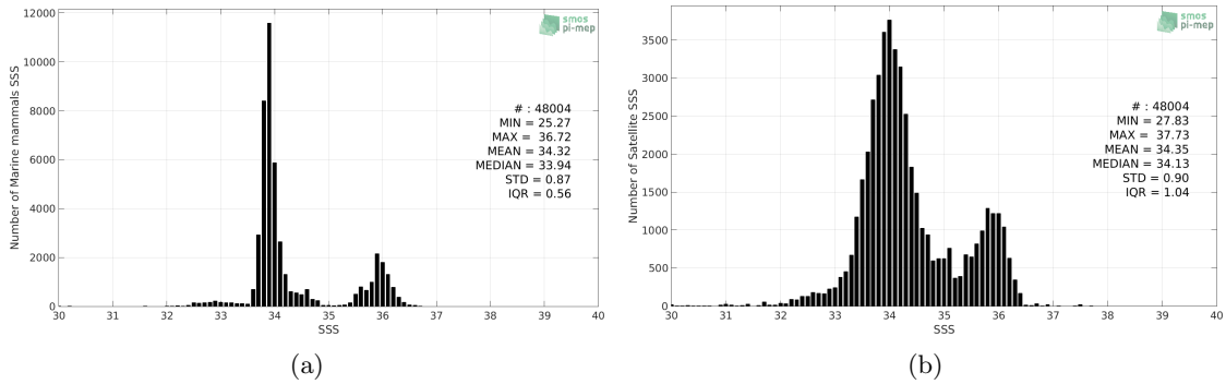
Figure 2: Histograms of SSS from Marine mammals (a) and SMOS SSS L3 v317 - Monthly - 25 km (CATDS-CPDC) (b) considering all match-up pairs per bins of 0.1 over the SMOS coastal zone (<800km) 60N-60S Pi-MEP region and for the full satellite product period.
