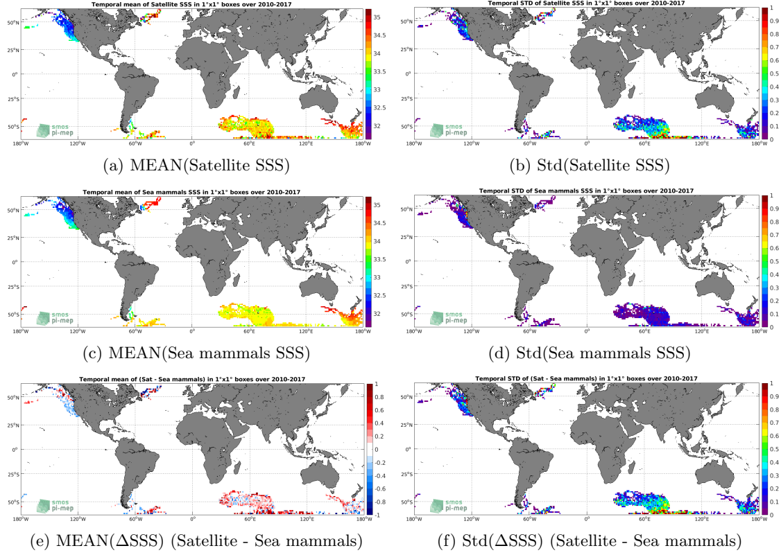
Figure 6: Temporal mean (left) and Std (right) of SSS from SMOS SSS L3 v317 - Monthly - 25 km (CATDS-CPDC) (top), Sea mammals (middle), and of \Delta SSS (Satellite - Sea mammals). Only match-up pairs are used to generate these maps.
