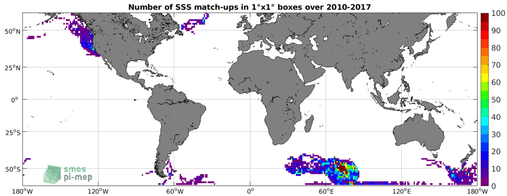
Figure 4: Number of SSS match-ups between Sea mammals SSS and the SMOS SSS L3 v317 - Monthly - 25 km (CATDS-CPDC) SSS product for the SMOS coastal zone (<800km) 60N-60S Pi-MEP region over 1°x1° boxes and for the full satellite product period.
