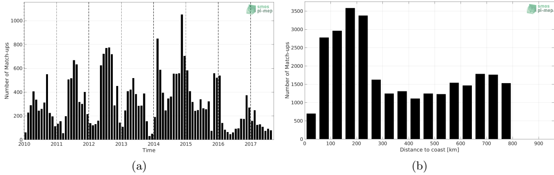
Figure 1: Number of match-ups between Sea mammals and SMOS SSS L3 v317 - Monthly - 25 km (CATDS-CPDC) SSS as a function of time (a) and as function of the distance to coast (b) over the SMOS coastal zone (<800km) 60N-60S Pi-MEP region and for the full satellite product period.
