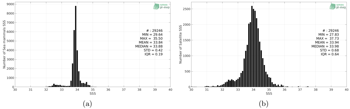
Figure 2: Histograms of SSS from Sea mammals (a) and SMOS SSS L3 v317 - Monthly - 25 km (CATDS-CPDC) (b) considering all match-up pairs per bins of 0.1 over the SMOS coastal zone (<800km) 60N-60S Pi-MEP region and for the full satellite product period.
