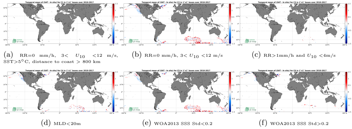
Figure 12: Temporal mean gridded over spatial boxes of size 1^\circ \times 1^\circ of \Delta SSS (SMOS SSS L3 v317 - Monthly - 25 km (CATDS-CPDC) - Sea mammals) for 6 different subdatasets corresponding to: RR=0 mm/h, 3 < U_{10} < 12 m/s, SST > 5^\circ C , distance to coast > 800 km (a), RR=0 mm/h, 3 < U_{10} < 12 m/s (b), RR > 1 mm/h and U_{10} < 4 m/s (c), MLD < 20 m (d), WOA2013 SSS Std < 0.2 (e), WOA2013 SSS Std > 0.2 (f).
