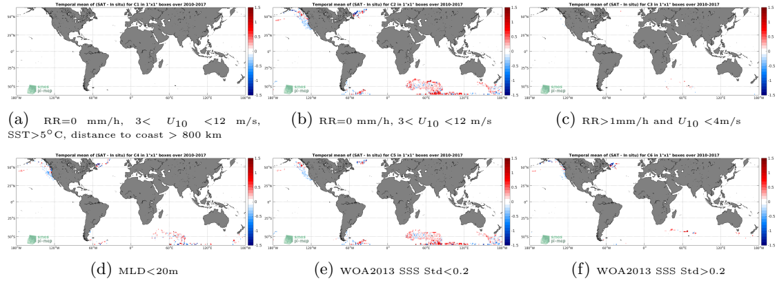
Figure 12: Temporal mean gridded over spatial boxes of size 1^\circ \times 1^\circ of \Delta SSS (SMOS L3 v317 - Monthly - 25 km (CATDS-CPDC) - Sea mammals) for 6 different subdatasets corresponding to: RR=0 mm/h, 3 < U_{10} < 12 m/s, SST > 5^\circ C , distance to coast > 800 km (a), RR=0 mm/h, 3 < U_{10} < 12 m/s (b), RR > 1 mm/h and U_{10} < 4 m/s (c), MLD < 20 m (d), WOA2013 SSS Std < 0.2 (e), WOA2013 SSS Std > 0.2 (f).
