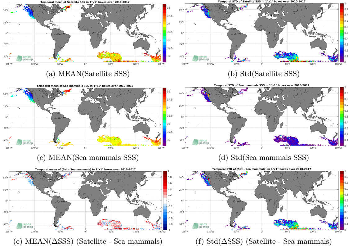
Figure 6: Temporal mean (left) and Std (right) of SSS from SMOS L3 v317 - Monthly - 25 km (CATDS-CPDC) (top), Sea mammals (middle), and of \Delta SSS (Satellite - Sea mammals). Only match-up pairs are used to generate these maps.
