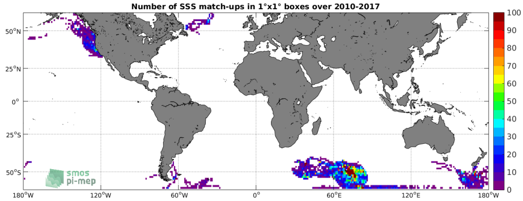
Figure 4: Number of SSS match-ups between Sea mammals SSS and the SMOS L3 v317 - Monthly - 25 km (CATDS-CPDC) SSS product for the SMOS coastal zone (<800km) 60N-60S Pi-MEP region over 1°x1° boxes and for the full satellite product period.
