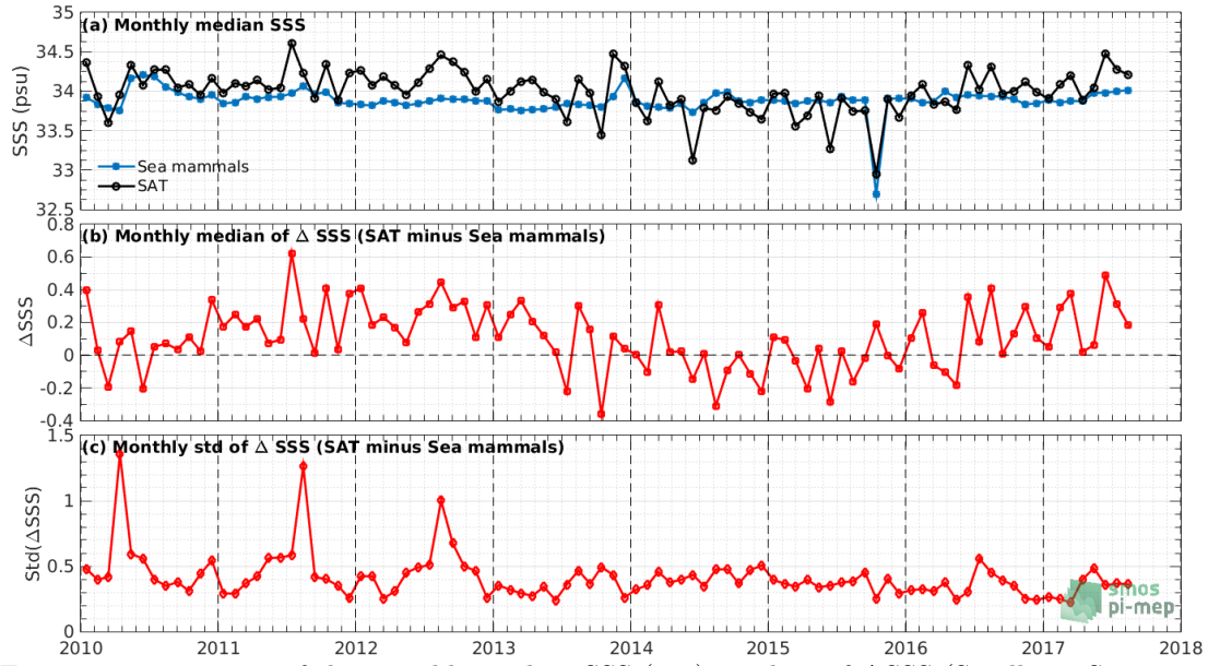
Figure 7: Time series of the monthly median SSS (top), median of \Delta\text{SSS} (Satellite - Sea mammals) and Std of \Delta\text{SSS} (Satellite - Sea mammals) over the SMOS coastal zone (<800km) 60N-60S Pi-MEP region considering all match-ups collected by the Pi-MEP.
