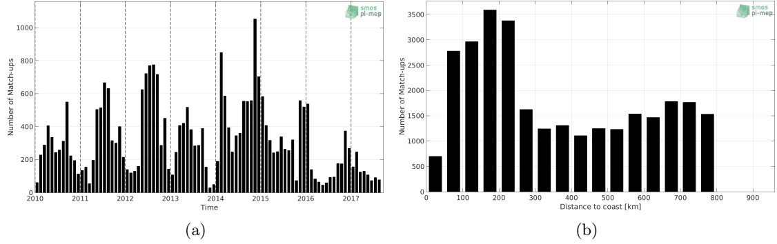
Figure 1: Number of match-ups between Sea mammals and SMOS L3 v317 - Monthly - 25 km (CATDS-CPDC) SSS as a function of time (a) and as function of the distance to coast (b) over the SMOS coastal zone (<800km) 60N-60S Pi-MEP region and for the full satellite product period.
