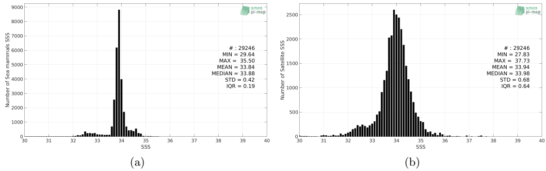
Figure 2: Histograms of SSS from Sea mammals (a) and SMOS L3 v317 - Monthly - 25 km (CATDS-CPDC) (b) considering all match-up pairs per bins of 0.1 over the SMOS coastal zone (<800km) 60N-60S Pi-MEP region and for the full satellite product period.
