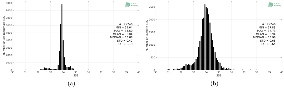
Figure 2: Histograms of SSS from Sea mammals (a) and SMOS-L3-CATDS-CPDC-V317-MONTHLY-25KM (b) considering all match-up pairs per bins of 0.1 over the SMOS coastal zone ( \geq 800\text{km} ) 60N-60S Pi-MEP region and for the full satellite product period.
