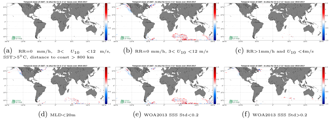
Figure 12: Temporal mean gridded over spatial boxes of size 1^\circ \times 1^\circ of \Delta SSS (SMOS-L3-CATDS-CPDC-V317-MONTHLY-25KM - Sea mammals) for 6 different subdatasets corresponding to: RR=0 mm/h, 3 < U_{10} < 12 m/s, SST > 5^\circ C , distance to coast > 800 km (a), RR=0 mm/h, 3 < U_{10} < 12 m/s (b), RR > 1 mm/h and U_{10} < 4 m/s (c), MLD < 20 m (d), WOA2013 SSS Std < 0.2 (e), WOA2013 SSS Std > 0.2 (f).
