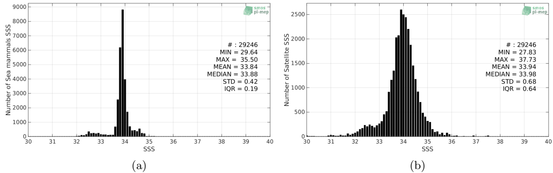
Figure 2: Histograms of SSS from Sea mammals (a) and SMOS-L3-CATDS-CPDC-V317-MONTHLY-25KM (b) considering all match-up pairs per bins of 0.1 over the SMOS coastal zone ( \approx 800 km) 60N-60S Pi-MEP region and for the full satellite product period.
