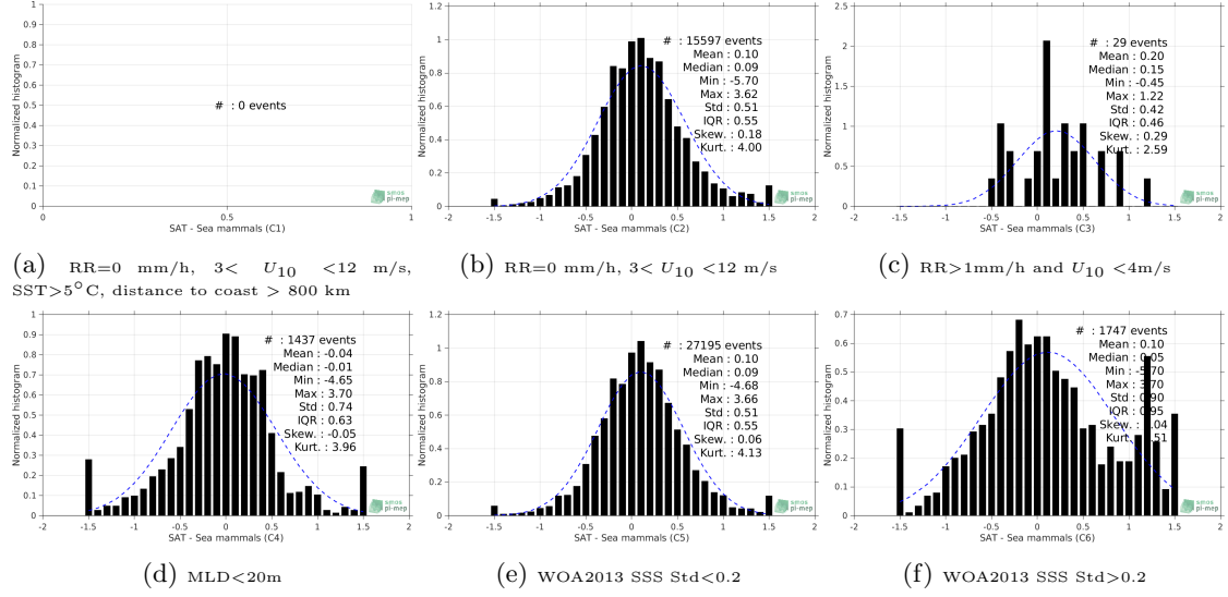
Figure 13: Normalized histogram of \Delta SSS (SMOS-L3-CATDS-CPDC-V317-MONTHLY-25KM - Sea mammals) for 6 different subdatasets corresponding to: RR=0 mm/h, 3 < U_{10} < 12 m/s, SST > 5^\circ C , distance to coast > 800 km (a), RR=0 mm/h, 3 < U_{10} < 12 m/s (b), RR > 1 mm/h and U_{10} < 4 m/s (c), MLD < 20 m (d), WOA2013 SSS Std < 0.2 (e), WOA2013 SSS Std > 0.2 (f).
