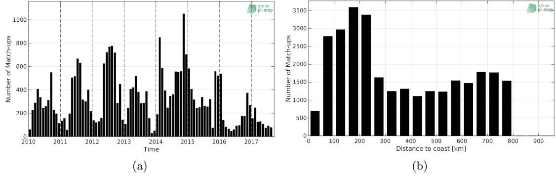
Figure 1: Number of match-ups between Sea mammals and SMOS-L3-CATDS-CPDC-V317-MONTHLY-25KM SSS as a function of time (a) and as function of the distance to coast (b) over the SMOS coastal zone ( \approx 800 km) 60N-60S Pi-MEP region and for the full satellite product period.
