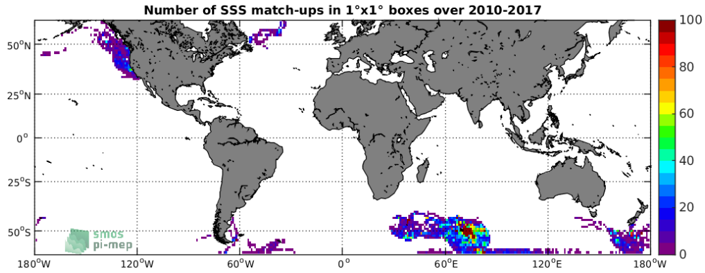
Figure 4: Number of SSS match-ups between Sea mammals SSS and the SMOS-L3-CATDS-CPDC-V317-MONTHLY-25KM SSS product for the SMOS coastal zone ( \pm 800\text{km} ) 60N-60S Pi-MEP region over 1^\circ \times 1^\circ boxes and for the full satellite product period.
