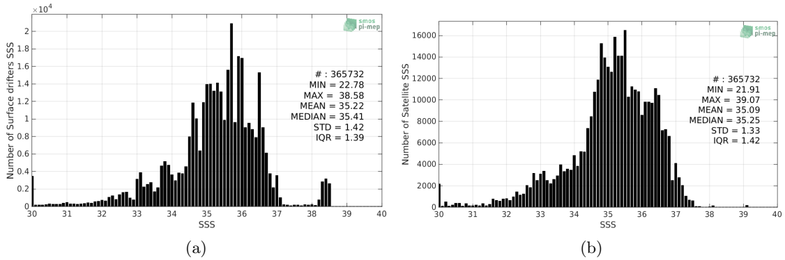
Figure 2: Histograms of SSS from Surface drifters (a) and SMOS-L3-CATDS-CPDC-V317-MONTHLY-25KM (b) considering all match-up pairs per bins of 0.1 over the SMOS coastal zone ( \geq 800 km) 60N-60S Pi-MEP region and for the full satellite product period.
