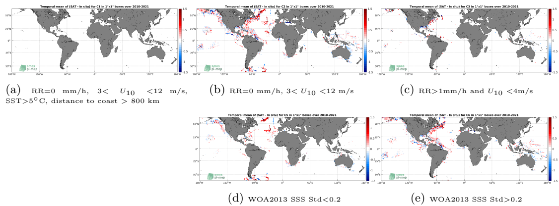
Figure 12: Temporal mean gridded over spatial boxes of size 1^\circ \times 1^\circ of \Delta SSS (SMOS SSS L3 v317 - 10 Days - 25 km (CATDS-CPDC) - TSG (SAMOS)) for 5 different subdatasets corresponding to:RR=0 mm/h, 3 < U_{10} < 12 m/s, SST >5^\circ C, distance to coast > 800 km (a), RR=0 mm/h, 3 < U_{10} < 12 m/s (b), RR >1 mm/h and U_{10} < 4 m/s (c), WOA2013 SSS Std <0.2 (d), WOA2013 SSS Std >0.2 (e).
