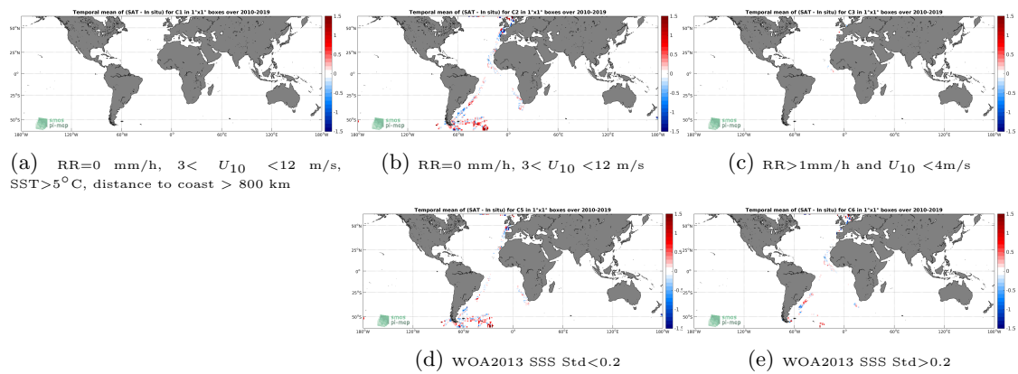
Figure 12: Temporal mean gridded over spatial boxes of size 1^\circ \times 1^\circ of \Delta SSS (SMOS SSS L3 v317 - 10 Days - 25 km (CATDS-CPDC) - TSG (Polarstern)) for 5 different subdatasets corresponding to:RR=0 mm/h, 3 < U_{10} < 12 m/s, SST >5^\circ C, distance to coast > 800 km (a), RR=0 mm/h, 3 < U_{10} < 12 m/s (b), RR >1 mm/h and U_{10} < 4 m/s (c), WOA2013 SSS Std <0.2 (d), WOA2013 SSS Std >0.2 (e).
