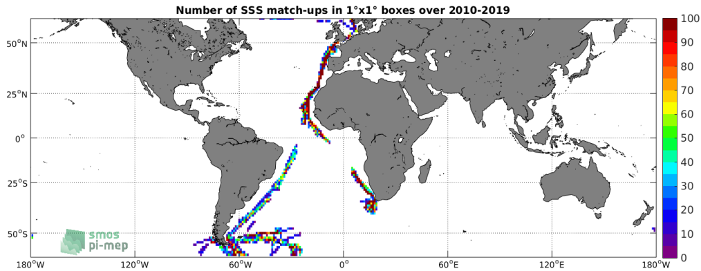
Figure 4: Number of SSS match-ups between TSG (Polarstern) SSS and the SMOS SSS L3 v317 - 10 Days - 25 km (CATDS-CPDC) SSS product for the SMOS coastal zone (<800km) 60N-60S Pi-MEP region over 1°x1° boxes and for the full satellite product period.
