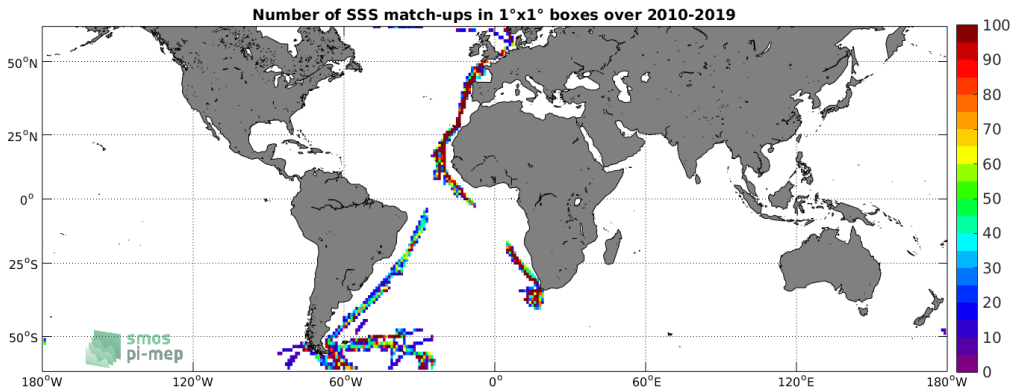
Figure 4: Number of SSS match-ups between TSG-POLARSTERN SSS and the SMOS L3 v317 - 10 Days - 25 km (CATDS-CPDC) SSS product for the SMOS coastal zone (<800km) 60N-60S Pi-MEP region over 1^\circ \times 1^\circ boxes and for the full satellite product period.
