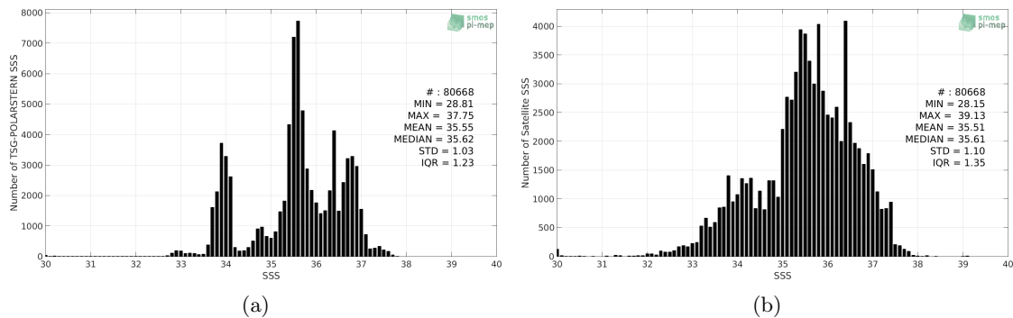
Figure 2: Histograms of SSS from TSG-POLARSTERN (a) and SMOS L3 v317 - 10 Days - 25 km (CATDS-CPDC) (b) considering all match-up pairs per bins of 0.1 over the SMOS coastal zone (<800km) 60N-60S Pi-MEP region and for the full satellite product period.
