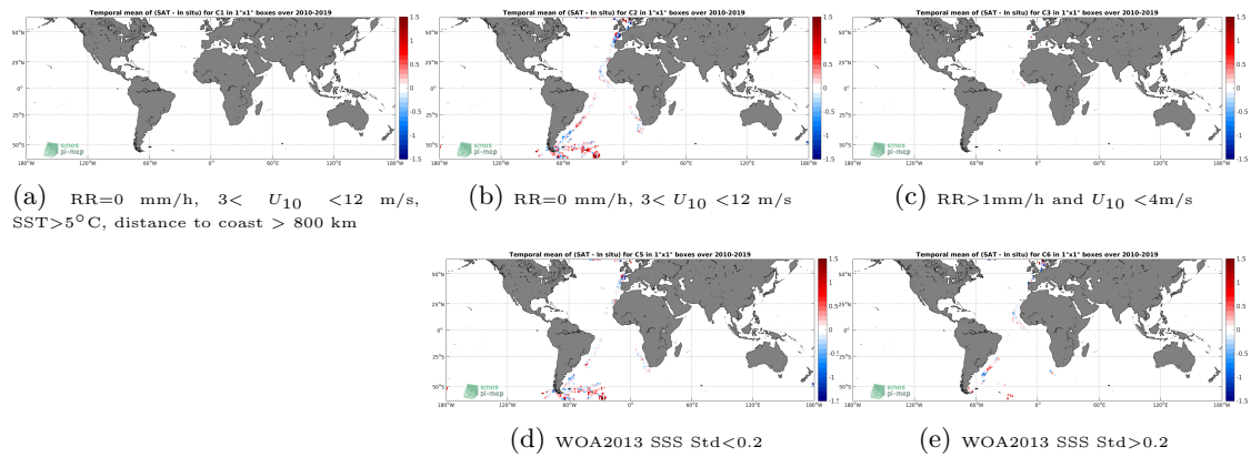
Figure 12: Temporal mean gridded over spatial boxes of size 1^\circ \times 1^\circ of \Delta SSS (SMOS L3 v317 - 10 Days - 25 km (CATDS-CPDC) - TSG-POLARSTERN) for 5 different subdatasets corresponding to:RR=0 mm/h, 3 < U_{10} < 12 m/s, SST >5^\circ C, distance to coast > 800 km (a), RR=0 mm/h, 3 < U_{10} < 12 m/s (b), RR >1 mm/h and U_{10} < 4 m/s (c), WOA2013 SSS Std <0.2 (d), WOA2013 SSS Std >0.2 (e).
