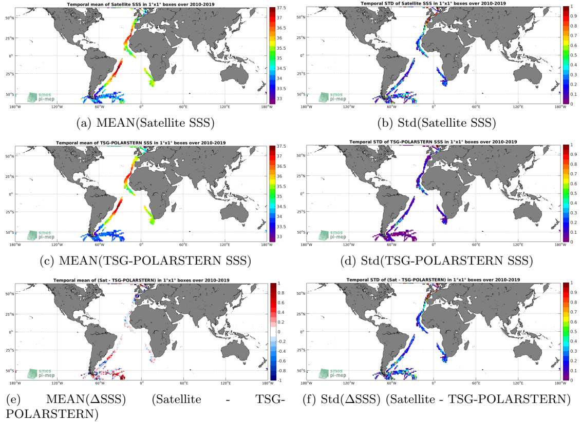
Figure 6: Temporal mean (left) and Std (right) of SSS from SMOS L3 v317 - 10 Days - 25 km (CATDS-CPDC) (top), TSG-POLARSTERN (middle), and of \Delta SSS (Satellite - TSG-POLARSTERN). Only match-up pairs are used to generate these maps.
