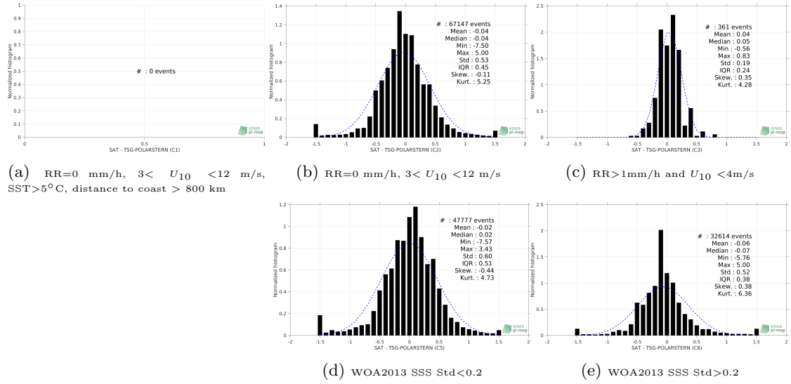
Figure 13: Normalized histogram of \Delta SSS (SMOS L3 v317 - 10 Days - 25 km (CATDS-CPDC) - TSG-POLARSTERN) for 5 different subdatasets corresponding to: RR=0 mm/h, 3 < U_{10} < 12 m/s, SST>5°C, distance to coast > 800 km (a), RR=0 mm/h, 3 < U_{10} < 12 m/s (b), RR>1mm/h and U_{10} < 4 m/s (c), WOA2013 SSS Std<0.2 (d), WOA2013 SSS Std>0.2 (e).
