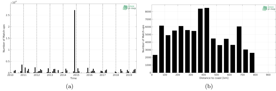
Figure 1: Number of match-ups between TSG-POLARSTERN and SMOS L3 v317 - 10 Days - 25 km (CATDS-CPDC) SSS as a function of time (a) and as function of the distance to coast (b) over the SMOS coastal zone (<800km) 60N-60S Pi-MEP region and for the full satellite product period.
