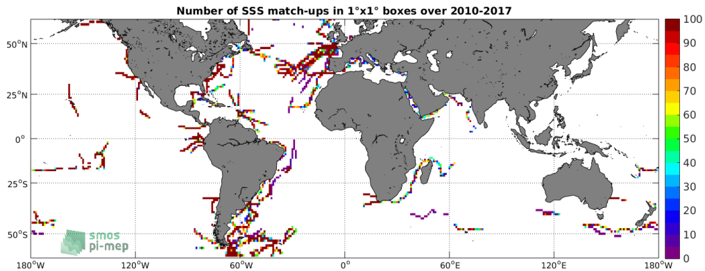
Figure 4: Number of SSS match-ups between TSG (GOSUD-Sailing-ship) SSS and the SMOS SSS L3 v317 - 10 Days - 25 km (CATDS-CPDC) SSS product for the SMOS coastal zone (<800km) 60N-60S Pi-MEP region over 1^\circ \times 1^\circ boxes and for the full satellite product period.
