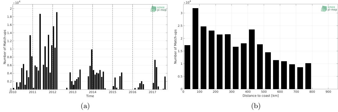
Figure 1: Number of match-ups between TSG-GOSUD-Sailing-ship and SMOS L3 v317 - 10 Days - 25 km (CATDS-CPDC) SSS as a function of time (a) and as function of the distance to coast (b) over the SMOS coastal zone (<800km) 60N-60S Pi-MEP region and for the full satellite product period.
