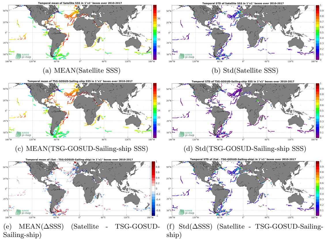
Figure 6: Temporal mean (left) and Std (right) of SSS from SMOS L3 v317 - 10 Days - 25 km (CATDS-CPDC) (top), TSG-GOSUD-Sailing-ship (middle), and of \Delta SSS (Satellite - TSG-GOSUD-Sailing-ship). Only match-up pairs are used to generate these maps.
