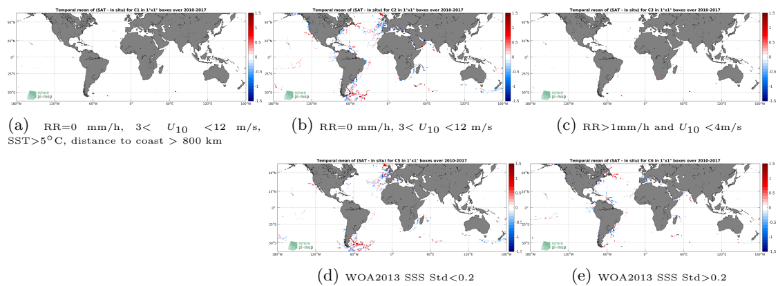
Figure 12: Temporal mean gridded over spatial boxes of size 1^\circ \times 1^\circ of \Delta SSS (SMOS L3 v317 - 10 Days - 25 km (CATDS-CPDC) - TSG-GOSUD-Sailing-ship) for 5 different subdatasets corresponding to:RR=0 mm/h, 3 < U_{10} < 12 m/s, SST >5^\circ\text{C} , distance to coast > 800 km (a), RR=0 mm/h, 3 < U_{10} < 12 m/s (b), RR >1 mm/h and U_{10} < 4 m/s (c), WOA2013 SSS Std <0.2 (d), WOA2013 SSS Std >0.2 (e).
