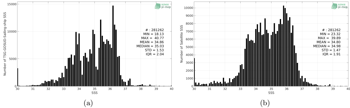
Figure 2: Histograms of SSS from TSG-GOSUD-Sailing-ship (a) and SMOS L3 v317 - 10 Days - 25 km (CATDS-CPDC) (b) considering all match-up pairs per bins of 0.1 over the SMOS coastal zone (<800km) 60N-60S Pi-MEP region and for the full satellite product period.
