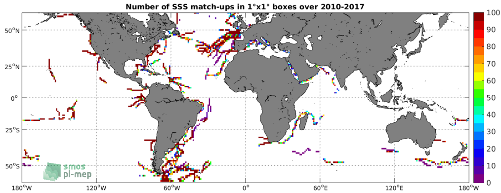
Figure 4: Number of SSS match-ups between TSG-GOSUD-Sailing-ship SSS and the SMOS L3 v317 - 10 Days - 25 km (CATDS-CPDC) SSS product for the SMOS coastal zone (<800km) 60N-60S Pi-MEP region over 1°x1° boxes and for the full satellite product period.
