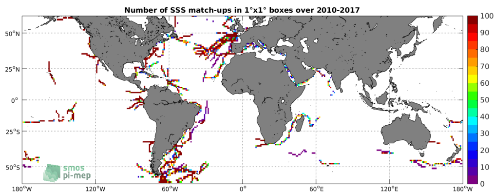
Figure 4: Number of SSS match-ups between TSG-GOSUD-Sailing-ship SSS and the SMOS-L3-CATDS-CPDC-V317-10DAYS-25KM SSS product for the SMOS coastal zone ( \pm 800\text{km} ) 60N-60S Pi-MEP region over 1^\circ \times 1^\circ boxes and for the full satellite product period.
