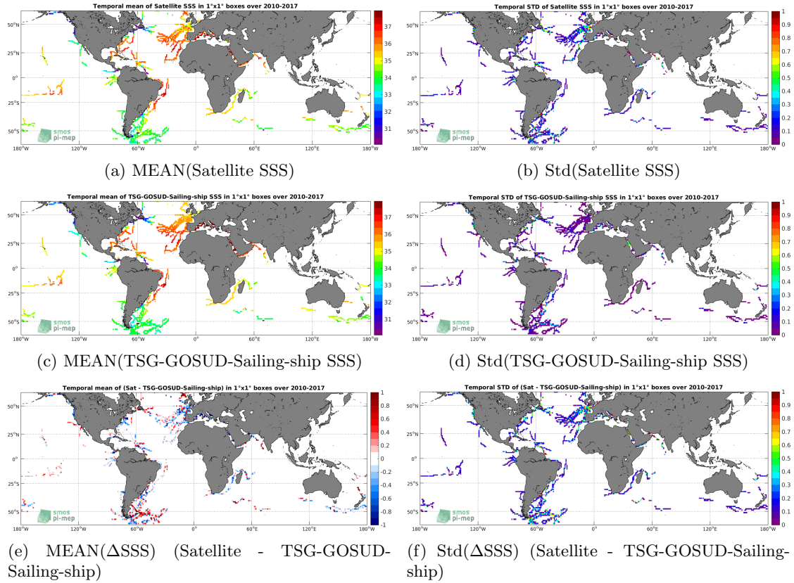
Figure 6: Temporal mean (left) and Std (right) of SSS from SMOS-L3-CATDS-CPDC-V317-10DAYS-25KM (top), TSG-GOSUD-Sailing-ship (middle), and of \Delta SSS (Satellite - TSG-GOSUD-Sailing-ship). Only match-up pairs are used to generate these maps.
