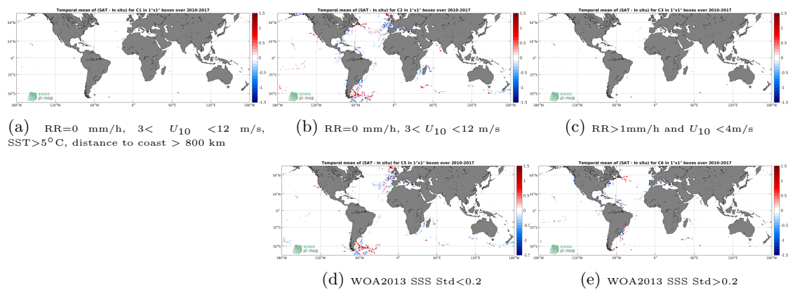
Figure 12: Temporal mean gridded over spatial boxes of size 1^\circ \times 1^\circ of \Delta\text{SSS} (SMOS-L3-CATDS-CPDC-V317-10DAYS-25KM - TSG-GOSUD-Sailing-ship) for 5 different subdatasets corresponding to:RR=0 mm/h, 3 < U_{10} < 12 m/s, SST >5^\circ\text{C} , distance to coast > 800 km (a), RR=0 mm/h, 3 < U_{10} < 12 m/s (b), RR >1 mm/h and U_{10} < 4 m/s (c), WOA2013 SSS Std <0.2 (d), WOA2013 SSS Std >0.2 (e).
