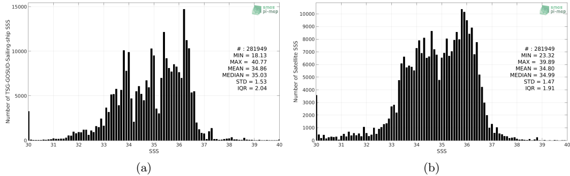
Figure 2: Histograms of SSS from TSG-GOSUD-Sailing-ship (a) and SMOS-L3-CATDS-CPDC-V317-10DAYS-25KM (b) considering all match-up pairs per bins of 0.1 over the SMOS coastal zone ( \approx 800 km) 60N-60S Pi-MEP region and for the full satellite product period.
