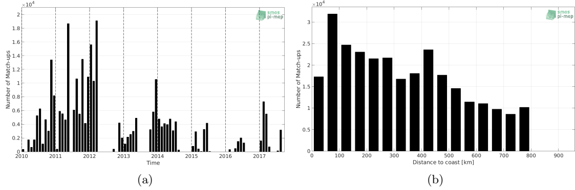
Figure 1: Number of match-ups between TSG-GOSUD-Sailing-ship and SMOS-L3-CATDS-CPDC-V317-10DAYS-25KM SSS as a function of time (a) and as function of the distance to coast (b) over the SMOS coastal zone ( \approx 800 km) 60N-60S Pi-MEP region and for the full satellite product period.
