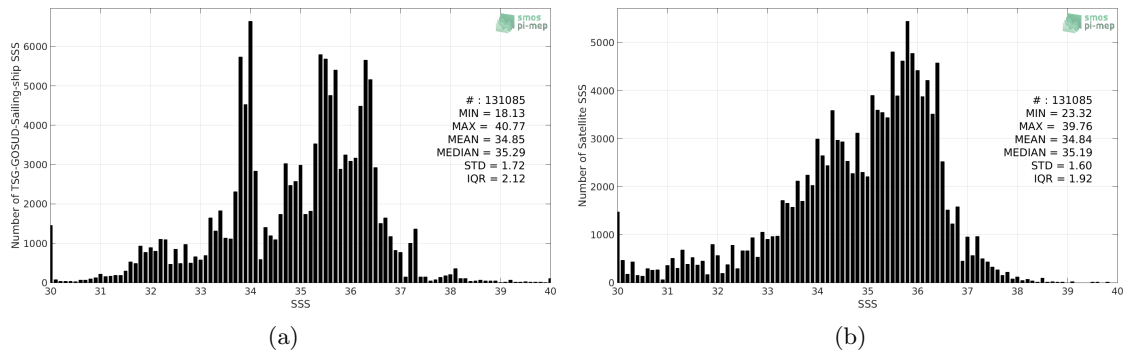
Figure 2: Histograms of SSS from TSG-GOSUD-Sailing-ship (a) and SMOS-L3-CATDS-CPDC-V317-10DAYS-25KM (b) considering all match-up pairs per bins of 0.1 over the SMOS coastal zone ( \approx 800\text{km} ) 60N-60S Pi-MEP region and for the full satellite product period.
