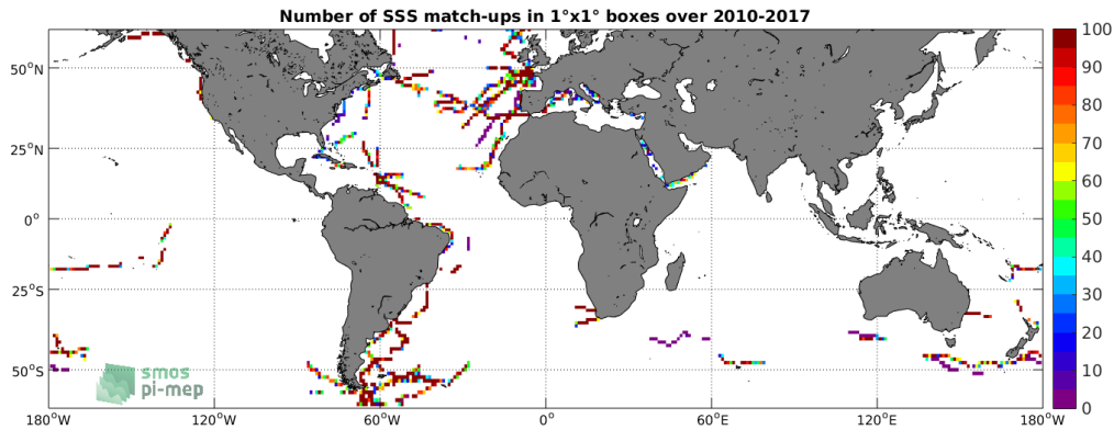
Figure 4: Number of SSS match-ups between TSG-GOSUD-Sailing-ship SSS and the SMOS-L3-CATDS-CPDC-V317-10DAYS-25KM SSS product for the SMOS coastal zone ( \approx 800\text{km} ) 60N-60S Pi-MEP region over 1^\circ \times 1^\circ boxes and for the full satellite product period.
