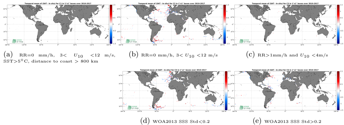
Figure 12: Temporal mean gridded over spatial boxes of size 1^\circ \times 1^\circ of \Delta SSS (SMOS-L3-CATDS-CPDC-V317-10DAYS-25KM - TSG-GOSUD-Sailing-ship) for 5 different subdatasets corresponding to:RR=0 mm/h, 3 < U_{10} < 12 m/s, SST >5^\circ C, distance to coast > 800 km (a), RR=0 mm/h, 3 < U_{10} < 12 m/s (b), RR >1 mm/h and U_{10} < 4 m/s (c), WOA2013 SSS Std <0.2 (d), WOA2013 SSS Std >0.2 (e).
