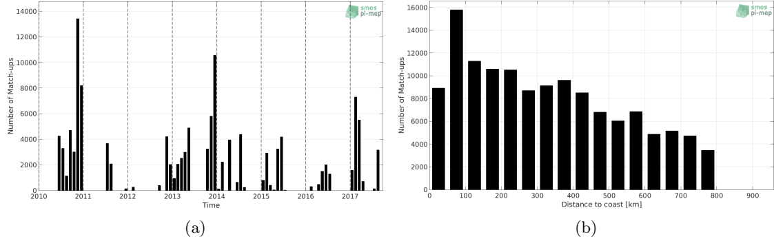
Figure 1: Number of match-ups between TSG-GOSUD-Sailing-ship and SMOS-L3-CATDS-CPDC-V317-10DAYS-25KM SSS as a function of time (a) and as function of the distance to coast (b) over the SMOS coastal zone ( \approx 800\text{km} ) 60N-60S Pi-MEP region and for the full satellite product period.
