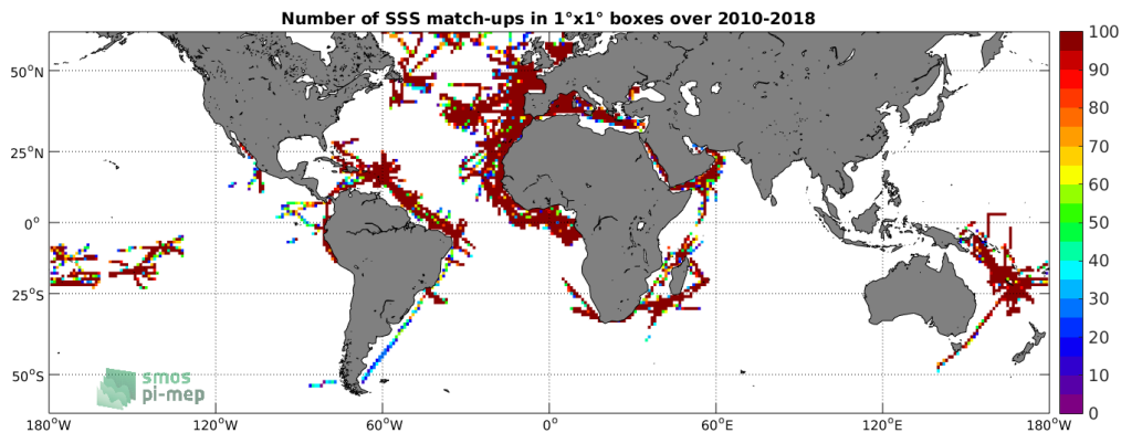
Figure 4: Number of SSS match-ups between TSG-GOSUD-Research-vessel SSS and the SMOS L3 v317 - 10 Days - 25 km (CATDS-CPDC) SSS product for the SMOS coastal zone (<800km) 60N-60S Pi-MEP region over 1^\circ \times 1^\circ boxes and for the full satellite product period.
