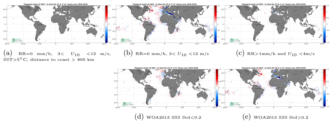
Figure 12: Temporal mean gridded over spatial boxes of size 1^\circ \times 1^\circ of \Delta SSS (SMOS L3 v317 - 10 Days - 25 km (CATDS-CPDC) - TSG-GOSUD-Research-vessel) for 5 different subdatasets corresponding to:RR=0 mm/h, 3 < U_{10} < 12 m/s, SST >5^\circ\text{C} , distance to coast > 800 km (a), RR=0 mm/h, 3 < U_{10} < 12 m/s (b), RR >1 mm/h and U_{10} < 4 m/s (c), WOA2013 SSS Std <0.2 (d), WOA2013 SSS Std >0.2 (e).
