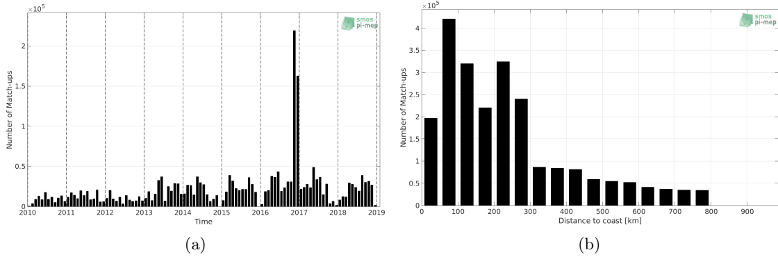
Figure 1: Number of match-ups between TSG-GOSUD-Research-vessel and SMOS L3 v317 - 10 Days - 25 km (CATDS-CPDC) SSS as a function of time (a) and as function of the distance to coast (b) over the SMOS coastal zone (<800km) 60N-60S Pi-MEP region and for the full satellite product period.
