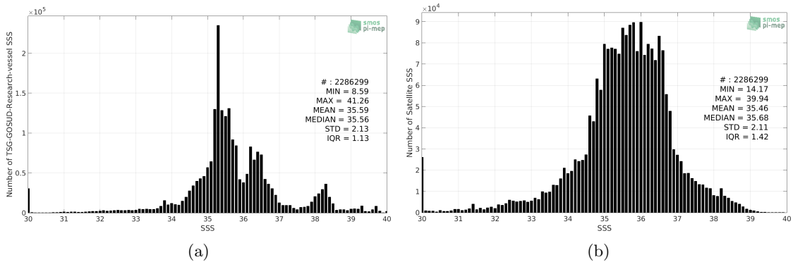
Figure 2: Histograms of SSS from TSG-GOSUD-Research-vessel (a) and SMOS L3 v317 - 10 Days - 25 km (CATDS-CPDC) (b) considering all match-up pairs per bins of 0.1 over the SMOS coastal zone (<800km) 60N-60S Pi-MEP region and for the full satellite product period.
