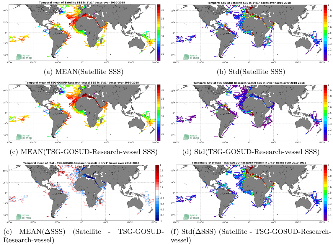
Figure 6: Temporal mean (left) and Std (right) of SSS from SMOS L3 v317 - 10 Days - 25 km (CATDS-CPDC) (top), TSG-GOSUD-Research-vessel (middle), and of \Delta SSS (Satellite - TSG-GOSUD-Research-vessel). Only match-up pairs are used to generate these maps.
