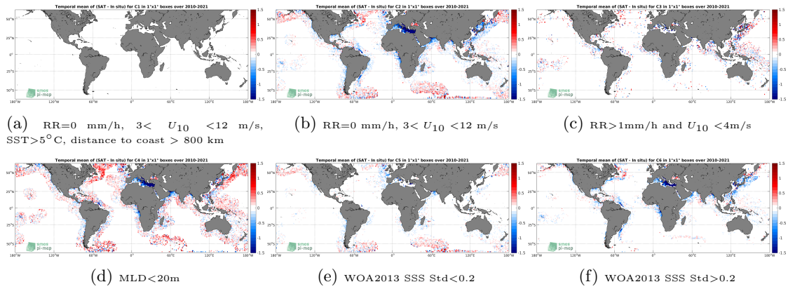
Figure 12: Temporal mean gridded over spatial boxes of size 1^\circ \times 1^\circ of \Delta SSS (SMOS SSS L3 v317 - 10 Days - 25 km (CATDS-CPDC) - Argo) for 6 different subdatasets corresponding to: RR=0 mm/h, 3 < U_{10} < 12 m/s, SST > 5°C, distance to coast > 800 km (a), RR=0 mm/h, 3 < U_{10} < 12 m/s (b), RR > 1mm/h and U_{10} < 4 m/s (c), MLD < 20m (d), WOA2013 SSS Std < 0.2 (e), WOA2013 SSS Std > 0.2 (f).
