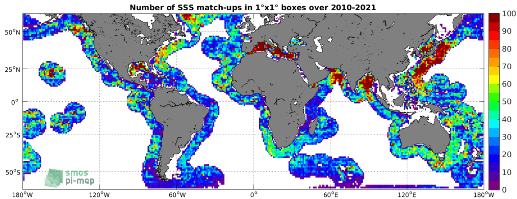
Figure 4: Number of SSS match-ups between Argo SSS and the SMOS SSS L3 v317 - 10 Days - 25 km (CATDS-CPDC) SSS product for the SMOS coastal zone ( <800\text{km} ) 60N-60S Pi-MEP region over 1^\circ \times 1^\circ boxes and for the full satellite product period.
