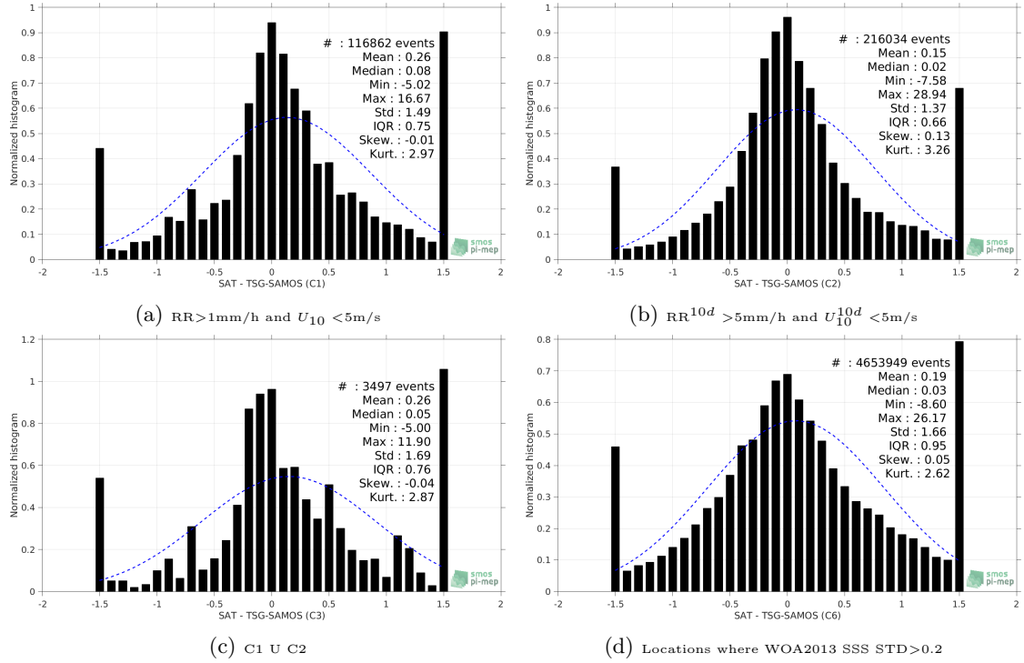
Figure 13: Normalized histogram of \Delta SSS (SMOS-L3-CATDS-CPDC-V3-MONTHLY-25KM - TSG-SAMOS) for 6 different subdatasets corresponding to: RR > 1mm/h and U_{10} < 5 m/s (a), RR^{10d} > 5 mm/h and U_{10}^{10d} < 5 m/s (b), C1 U C2 (c), Locations where WOA2013 SSS STD > 0.2 (d).
