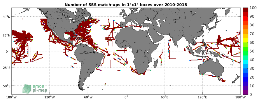
Figure 4: Number of SSS match-ups between TSG-SAMOS SSS and the SMOS-L3-CATDS-CPDC-V3-MONTHLY-25KM SSS product for the SMOS coastal zone ( \pm 800\text{km} ) 60N-60S Pi-MEP region over 1^\circ \times 1^\circ boxes and for the full satellite product period.
