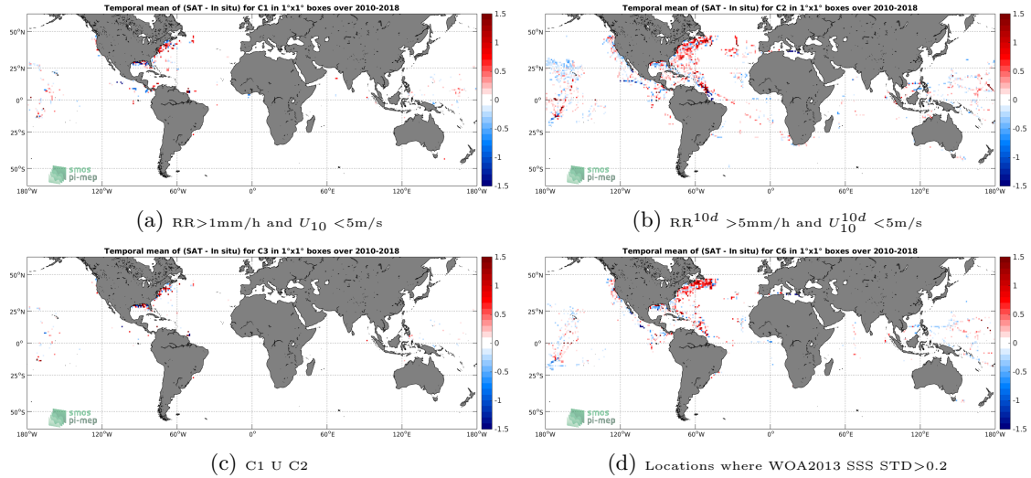
Figure 12: Temporal mean gridded over spatial boxes of size 1^\circ \times 1^\circ of \Delta SSS (SMOS-L3-CATDS-CPDC-V3-MONTHLY-25KM - TSG-SAMOS) for 4 different subdatasets corresponding to: RR > 1\text{mm/h} and U_{10} < 5\text{m/s} (a), RR^{10d} > 5\text{mm/h} and U_{10}^{10d} < 5\text{m/s} (b), C1 U C2 (c), Locations where WOA2013 SSS STD > 0.2 (d).
