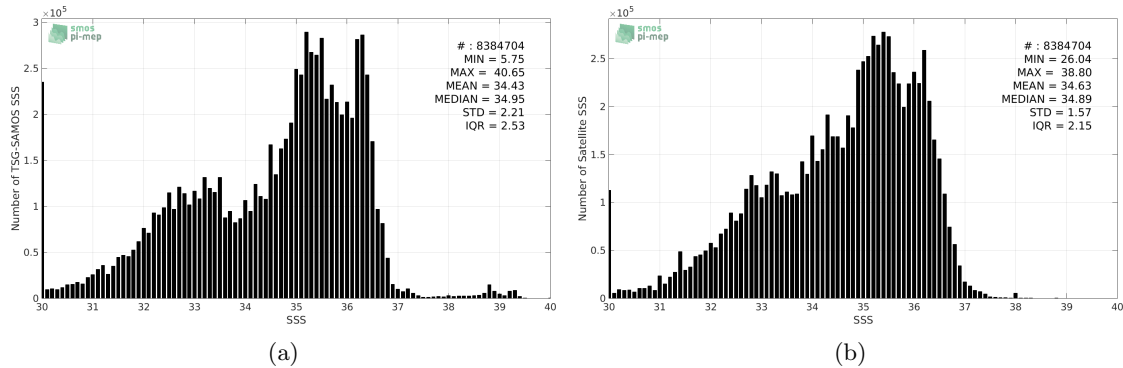
Figure 2: Histograms of SSS from TSG-SAMOS (a) and SMOS-L3-CATDS-CPDC-V3-MONTHLY-25KM (b) considering all match-up pairs per bins of 0.1 over the SMOS coastal zone ( \approx 800 km) 60N-60S Pi-MEP region and for the full satellite product period.
