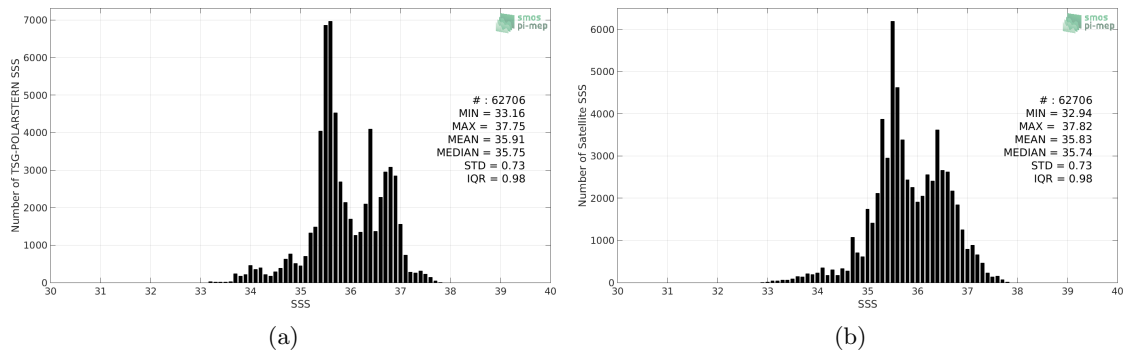
Figure 2: Histograms of SSS from TSG-POLARSTERN (a) and SMOS-L3-CATDS-CPDC-V3-MONTHLY-25KM (b) considering all match-up pairs per bins of 0.1 over the SMOS coastal zone ( \approx 800 km) 60N-60S Pi-MEP region and for the full satellite product period.
