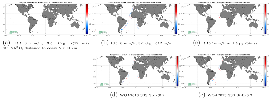
Figure 12: Temporal mean gridded over spatial boxes of size 1^\circ \times 1^\circ of \Delta SSS (SMOS-L3-CATDS-CPDC-V3-MONTHLY-25KM - TSG-POLARSTERN) for 5 different subdatasets corresponding to:RR=0 mm/h, 3 < U_{10} < 12 m/s, SST >5^\circ C, distance to coast > 800 km (a), RR=0 mm/h, 3 < U_{10} < 12 m/s (b), RR >1 mm/h and U_{10} < 4 m/s (c), WOA2013 SSS Std <0.2 (d), WOA2013 SSS Std >0.2 (e).
