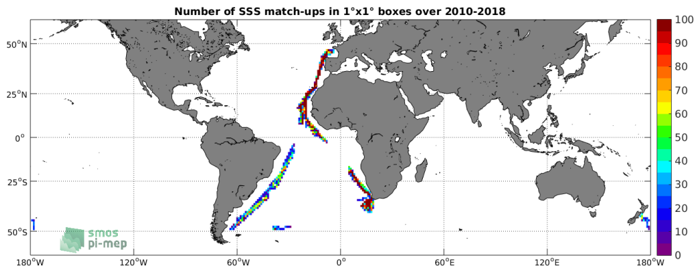
Figure 4: Number of SSS match-ups between TSG-POLARSTERN SSS and the SMOS-L3-CATDS-CPDC-V3-MONTHLY-25KM SSS product for the SMOS coastal zone ( \pm 800\text{km} ) 60N-60S Pi-MEP region over 1^\circ \times 1^\circ boxes and for the full satellite product period.
