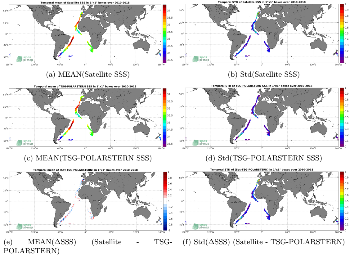
Figure 6: Temporal mean (left) and Std (right) of SSS from SMOS-L3-CATDS-CPDC-V3-MONTHLY-25KM (top), TSG-POLARSTERN (middle), and of \Delta SSS (Satellite - TSG-POLARSTERN). Only match-up pairs are used to generate these maps.
