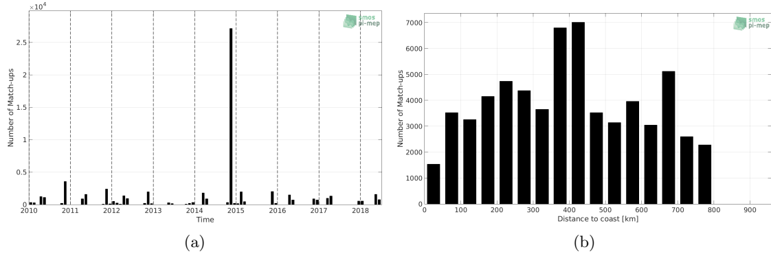
Figure 1: Number of match-ups between TSG-POLARSTERN and SMOS-L3-CATDS-CPDC-V3-MONTHLY-25KM SSS as a function of time (a) and as function of the distance to coast (b) over the SMOS coastal zone ( \approx 800 km) 60N-60S Pi-MEP region and for the full satellite product period.
