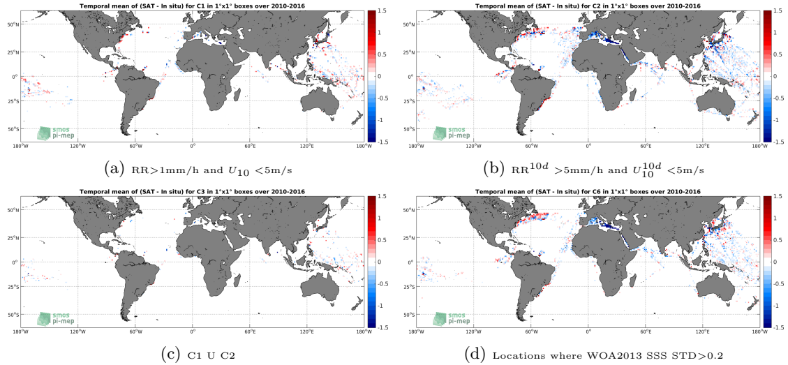
Figure 12: Temporal mean gridded over spatial boxes of size 1^\circ \times 1^\circ of \Delta SSS (SMOS-L3-CATDS-CPDC-V3-MONTHLY-25KM - TSG-LEGOS-DM) for 4 different subdatasets corresponding to: RR > 1\text{mm/h} and U_{10} < 5\text{m/s} (a), RR^{10d} > 5\text{mm/h} and U_{10}^{10d} < 5\text{m/s} (b), C1 U C2 (c), Locations where WOA2013 SSS STD > 0.2 (d).
