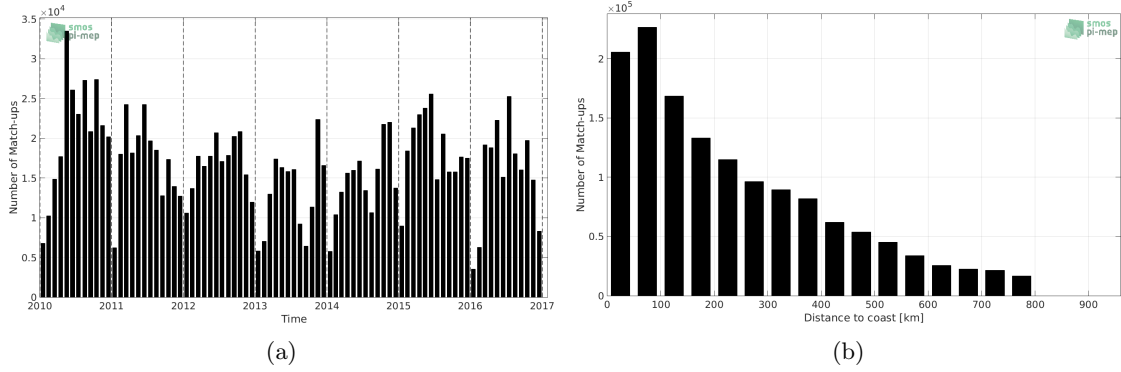
Figure 1: Number of match-ups between TSG-LEGOS-DM and SMOS-L3-CATDS-CPDC-V3-MONTHLY-25KM SSS as a function of time (a) and as function of the distance to coast (b) over the SMOS coastal zone ( \approx 800 km) 60N-60S Pi-MEP region and for the full satellite product period.
