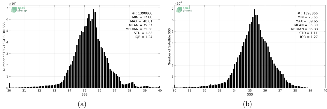
Figure 2: Histograms of SSS from TSG-LEGOS-DM (a) and SMOS-L3-CATDS-CPDC-V3-MONTHLY-25KM (b) considering all match-up pairs per bins of 0.1 over the SMOS coastal zone ( \approx 800 km) 60N-60S Pi-MEP region and for the full satellite product period.
