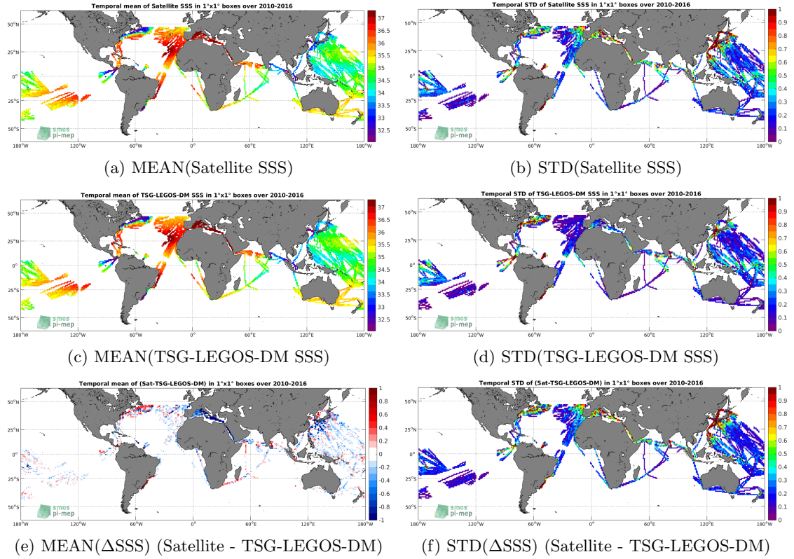
Figure 6: Temporal mean (left) and STD (right) of SSS from SMOS-L3-CATDS-CPDC-V3-MONTHLY-25KM (top), TSG-LEGOS-DM (middle), and of \Delta SSS (Satellite - TSG-LEGOS-DM). Only match-up pairs are used to generate these maps.
