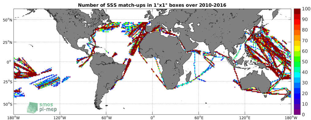
Figure 4: Number of SSS match-ups between TSG-LEGOS-DM SSS and the SMOS-L3-CATDS-CPDC-V3-MONTHLY-25KM SSS product for the SMOS coastal zone ( \pm 800\text{km} ) 60N-60S Pi-MEP region over 1^\circ \times 1^\circ boxes and for the full satellite product period.
