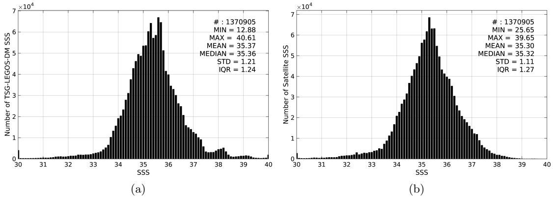
Figure 2: Histograms of SSS from TSG-LEGOS-DM (a) and SMOS-L3-CATDS-CPDC-V3-MONTHLY-25KM (b) considering all match-up pairs per bins of 0.1 over the SMOS coastal zone ( \approx 800 km) 60N-60S Pi-MEP region and for the full satellite product period.
