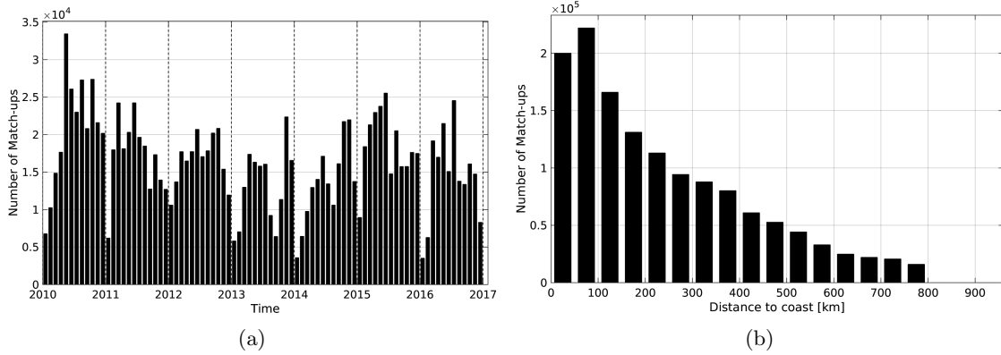
Figure 1: Number of match-ups between TSG-LEGOS-DM and SMOS-L3-CATDS-CPDC-V3-MONTHLY-25KM SSS as a function of time (a) and as function of the distance to coast (b) over the SMOS coastal zone ( \approx 800 km) 60N-60S Pi-MEP region and for the full satellite product period.
