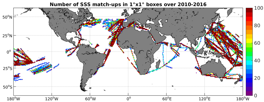
Figure 4: Number of SSS match-ups between TSG-LEGOS-DM SSS and the SMOS-L3-CATDS-CPDC-V3-MONTHLY-25KM SSS product for the SMOS coastal zone ( \geq 800\text{km} ) 60N-60S Pi-MEP region over 1^\circ \times 1^\circ boxes and for the full satellite product period.
