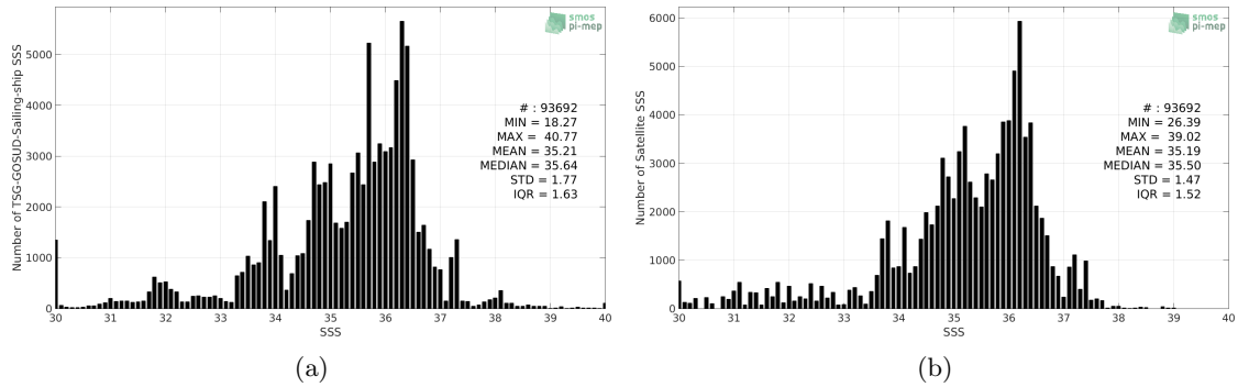
Figure 2: Histograms of SSS from TSG-GOSUD-Sailing-ship (a) and SMOS-L3-CATDS-CPDC-V3-MONTHLY-25KM (b) considering all match-up pairs per bins of 0.1 over the SMOS coastal zone ( \leq 800 km) 60N-60S Pi-MEP region and for the full satellite product period.
