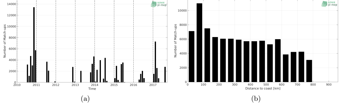
Figure 1: Number of match-ups between TSG-GOSUD-Sailing-ship and SMOS-L3-CATDS-CPDC-V3-MONTHLY-25KM SSS as a function of time (a) and as function of the distance to coast (b) over the SMOS coastal zone ( \leq 800 km) 60N-60S Pi-MEP region and for the full satellite product period.
