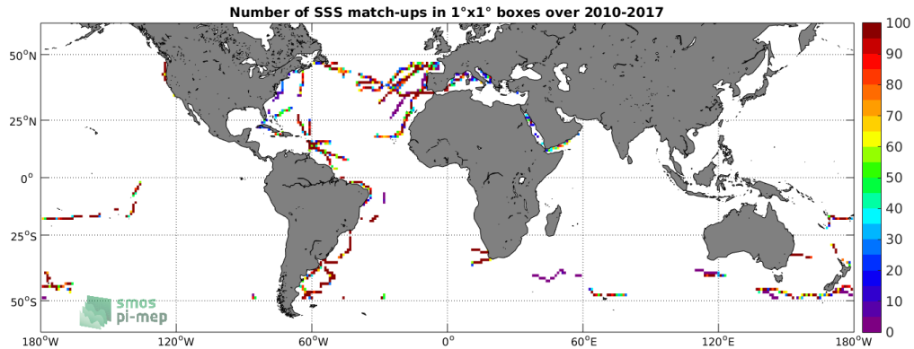
Figure 4: Number of SSS match-ups between TSG-GOSUD-Sailing-ship SSS and the SMOS-L3-CATDS-CPDC-V3-MONTHLY-25KM SSS product for the SMOS coastal zone ( \pm 800\text{km} ) 60^\circ\text{N} - 60^\circ\text{S} Pi-MEP region over 1^\circ \times 1^\circ boxes and for the full satellite product period.
