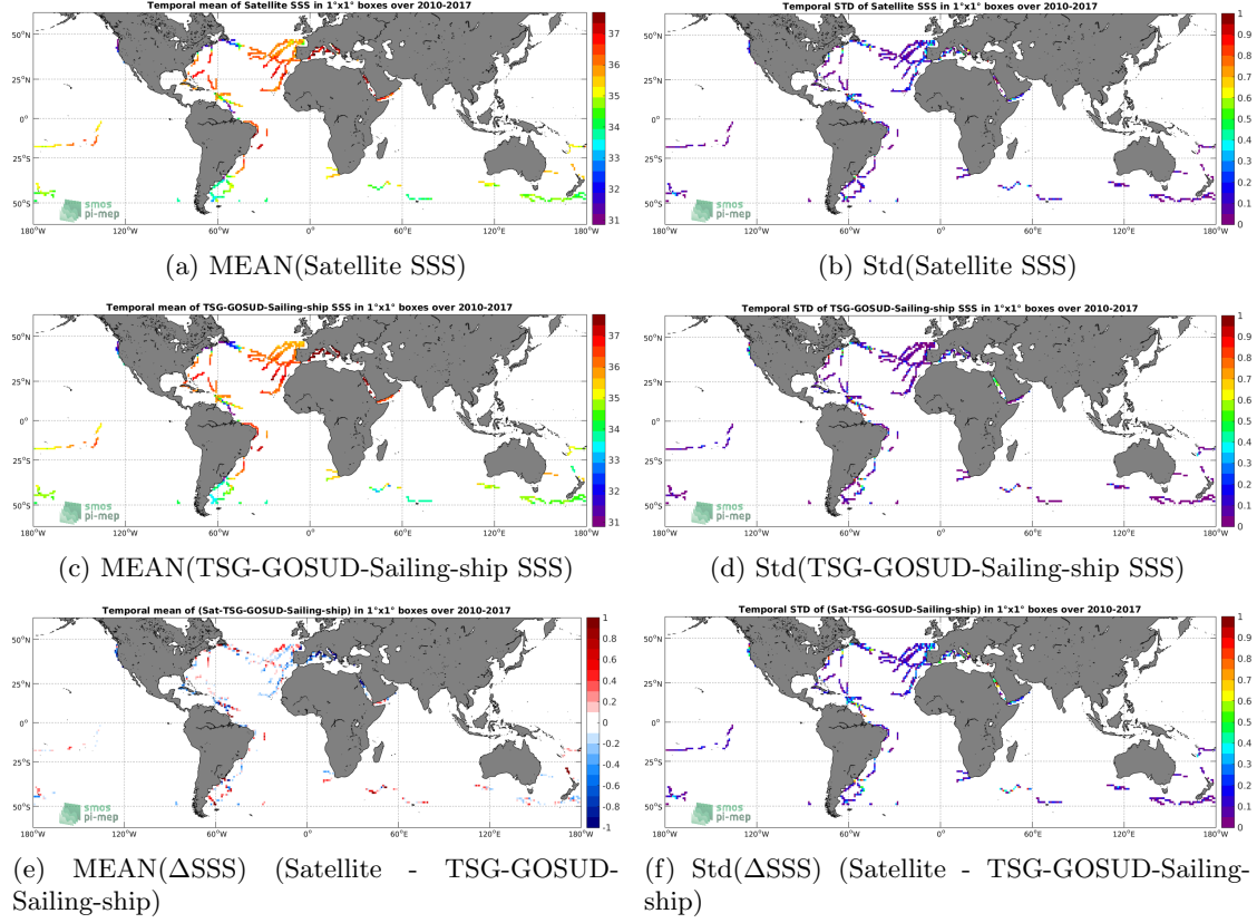
Figure 6: Temporal mean (left) and Std (right) of SSS from SMOS-L3-CATDS-CPDC-V3-MONTHLY-25KM (top), TSG-GOSUD-Sailing-ship (middle), and of \Delta SSS (Satellite - TSG-GOSUD-Sailing-ship). Only match-up pairs are used to generate these maps.
