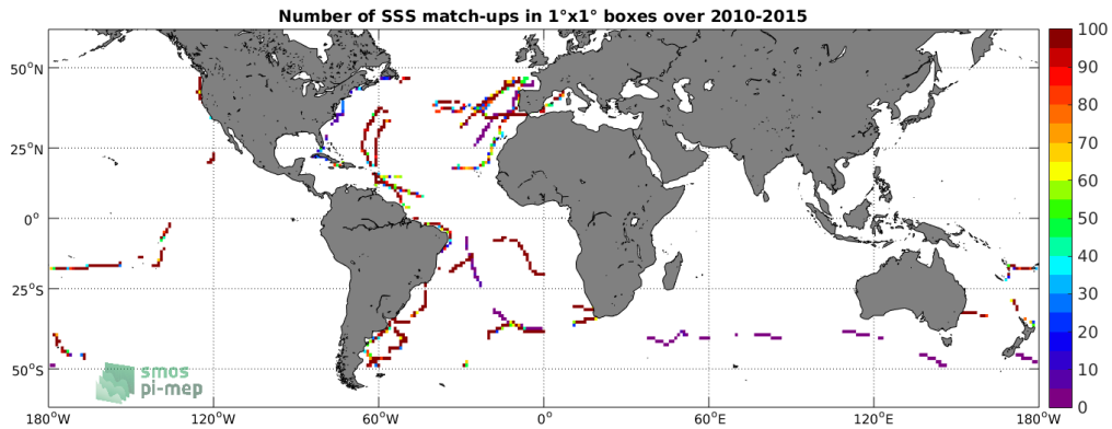
Figure 4: Number of SSS match-ups between TSG-GOSUD-Sailing-ship SSS and the SMOS-L3-CATDS-CPDC-V3-MONTHLY-25KM SSS product for the SMOS coastal zone ( \pm 800 km) 60N-60S Pi-MEP region over 1^\circ \times 1^\circ boxes and for the full satellite product period.
