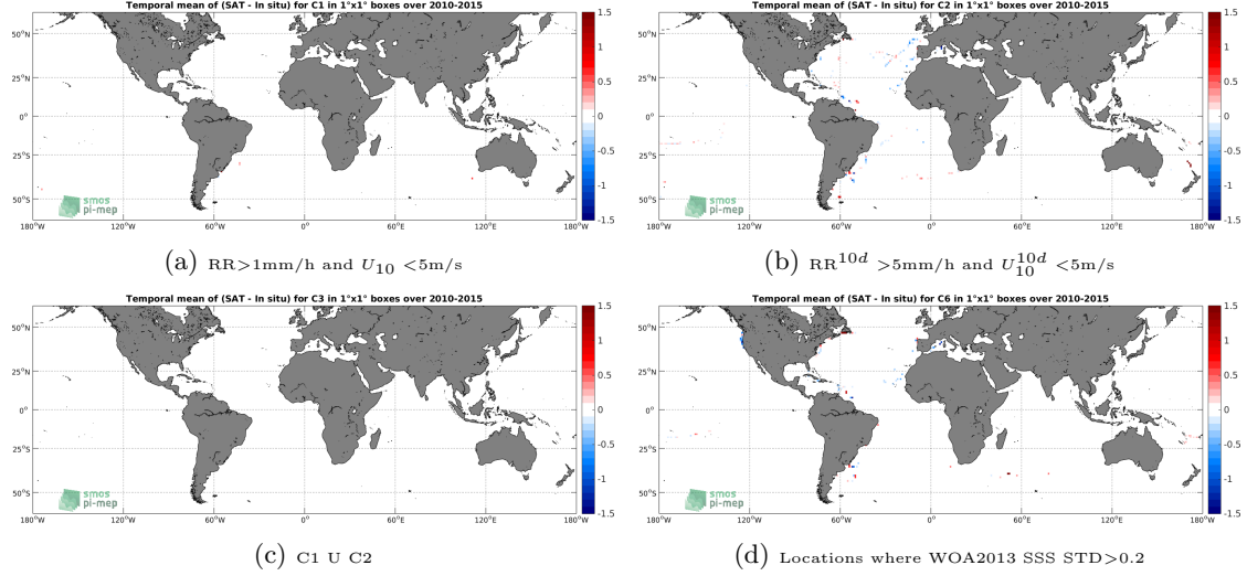
Figure 12: Temporal mean gridded over spatial boxes of size 1^\circ \times 1^\circ of \Delta SSS (SMOS-L3-CATDS-CPDC-V3-MONTHLY-25KM - TSG-GOSUD-Sailing-ship) for 4 different subdatasets corresponding to: RR > 1mm/h and U_{10} < 5 m/s (a), RR 10d > 5mm/h and U_{10}^{10d} < 5 m/s (b), C1 U C2 (c), Locations where WOA2013 SSS STD > 0.2 (d).
