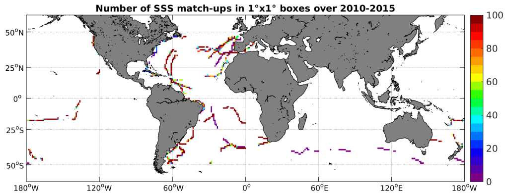
Figure 4: Number of SSS match-ups between TSG-GOSUD-Sailing-ship SSS and the SMOS-L3-CATDS-CPDC-V3-MONTHLY-25KM SSS product for the SMOS coastal zone ( \geq 800\text{km} ) 60^\circ\text{N} - 60^\circ\text{S} Pi-MEP region over 1^\circ \times 1^\circ boxes and for the full satellite product period.
