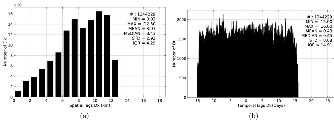
Figure 5: Histograms of the spatial (a) and temporal (b) lags between the time of the TSG-GOSUD-Research-vessel measurements and the date of the corresponding SMOS-L3-CATDS-CPDC-V3-MONTHLY-25KM SSS product.
