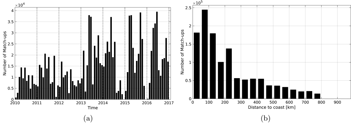
Figure 1: Number of match-ups between TSG-GOSUD-Research-vessel and SMOS-L3-CATDS-CPDC-V3-MONTHLY-25KM SSS as a function of time (a) and as function of the distance to coast (b) over the SMOS coastal zone ( \leq 800 km) 60N-60S Pi-MEP region and for the full satellite product period.
