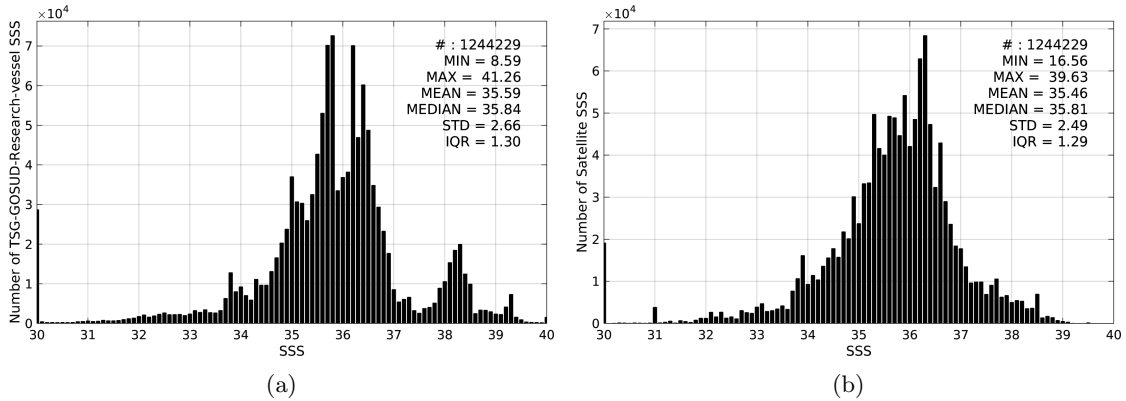
Figure 2: Histograms of SSS from TSG-GOSUD-Research-vessel (a) and SMOS-L3-CATDS-CPDC-V3-MONTHLY-25KM (b) considering all match-up pairs per bins of 0.1 over the SMOS coastal zone ( \leq 800 km) 60N-60S Pi-MEP region and for the full satellite product period.
