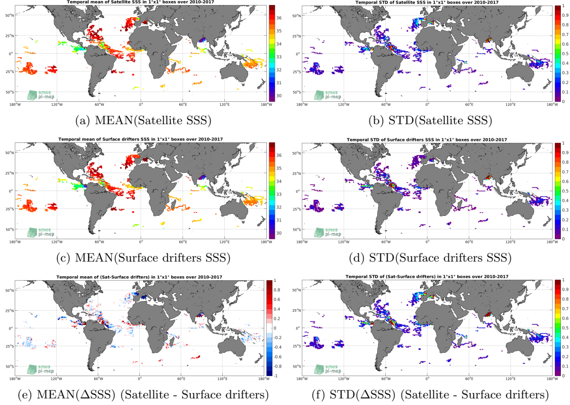
Figure 5: Temporal mean (left) and STD (right) of SSS from SMOS-L3-CATDS-CPDC-V3-MONTHLY-25KM (top), Surface drifters (middle), and of \Delta SSS (Satellite - Surface drifters). Only match-up pairs are used to generate these maps.
