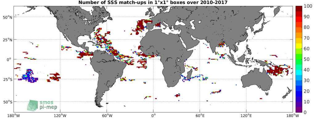
Figure 3: Number of SSS match-ups between Surface drifters SSS and the SMOS-L3-CATDS-CPDC-V3-MONTHLY-25KM SSS product for the SMOS coastal zone ( \leq 800\text{km} ) 60N-60S Pi-MEP region over 1^\circ \times 1^\circ boxes and for the full satellite product period.
