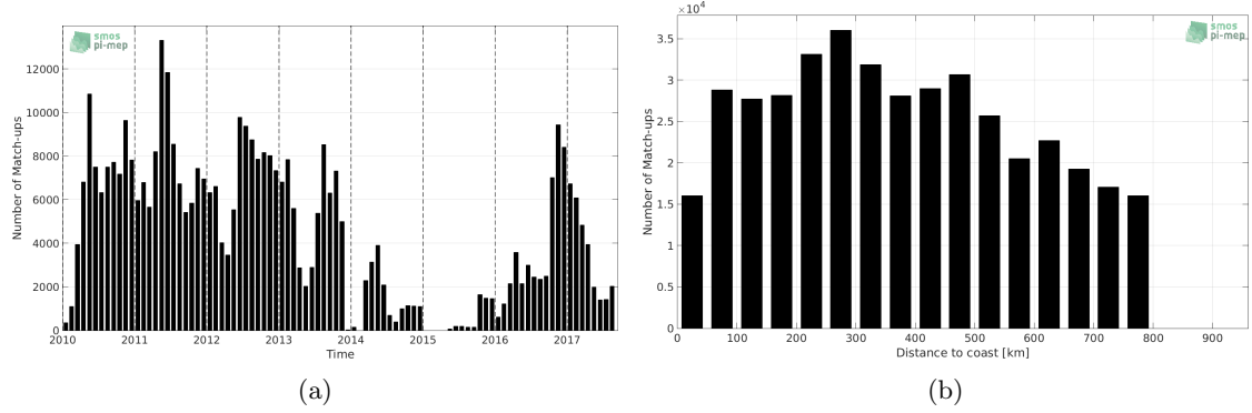
Figure 1: Number of match-ups between Surface drifters and SMOS-L3-CATDS-CPDC-V3-MONTHLY-25KM SSS as a function of time (a) and as function of the distance to coast (b) over the SMOS coastal zone ( \leq 800 km) 60N-60S Pi-MEP region and for the full satellite product period.
