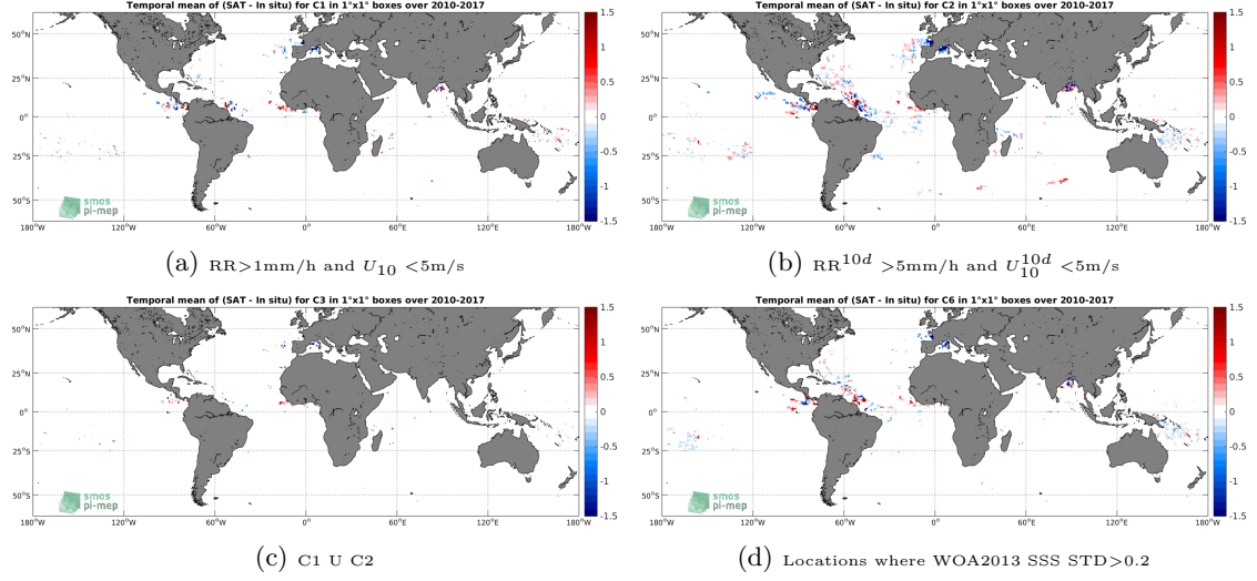
Figure 11: Temporal mean gridded over spatial boxes of size 1^\circ \times 1^\circ of \Delta SSS (SMOS-L3-CATDS-CPDC-V3-MONTHLY-25KM - Surface drifters) for 4 different subdatasets corresponding to: RR > 1\text{mm/h} and U_{10} < 5\text{m/s} (a), RR^{10d} > 5\text{mm/h} and U_{10}^{10d} < 5\text{m/s} (b), C1 U C2 (c), Locations where WOA2013 SSS STD > 0.2 (d).
