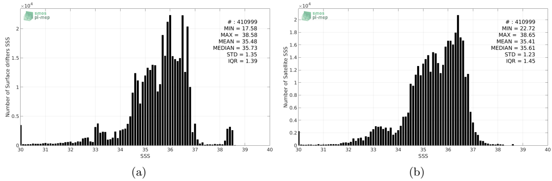
Figure 2: Histograms of SSS from Surface drifters (a) and SMOS-L3-CATDS-CPDC-V3-MONTHLY-25KM (b) considering all match-up pairs per bins of 0.1 over the SMOS coastal zone ( \leq 800 km) 60N-60S Pi-MEP region and for the full satellite product period.
