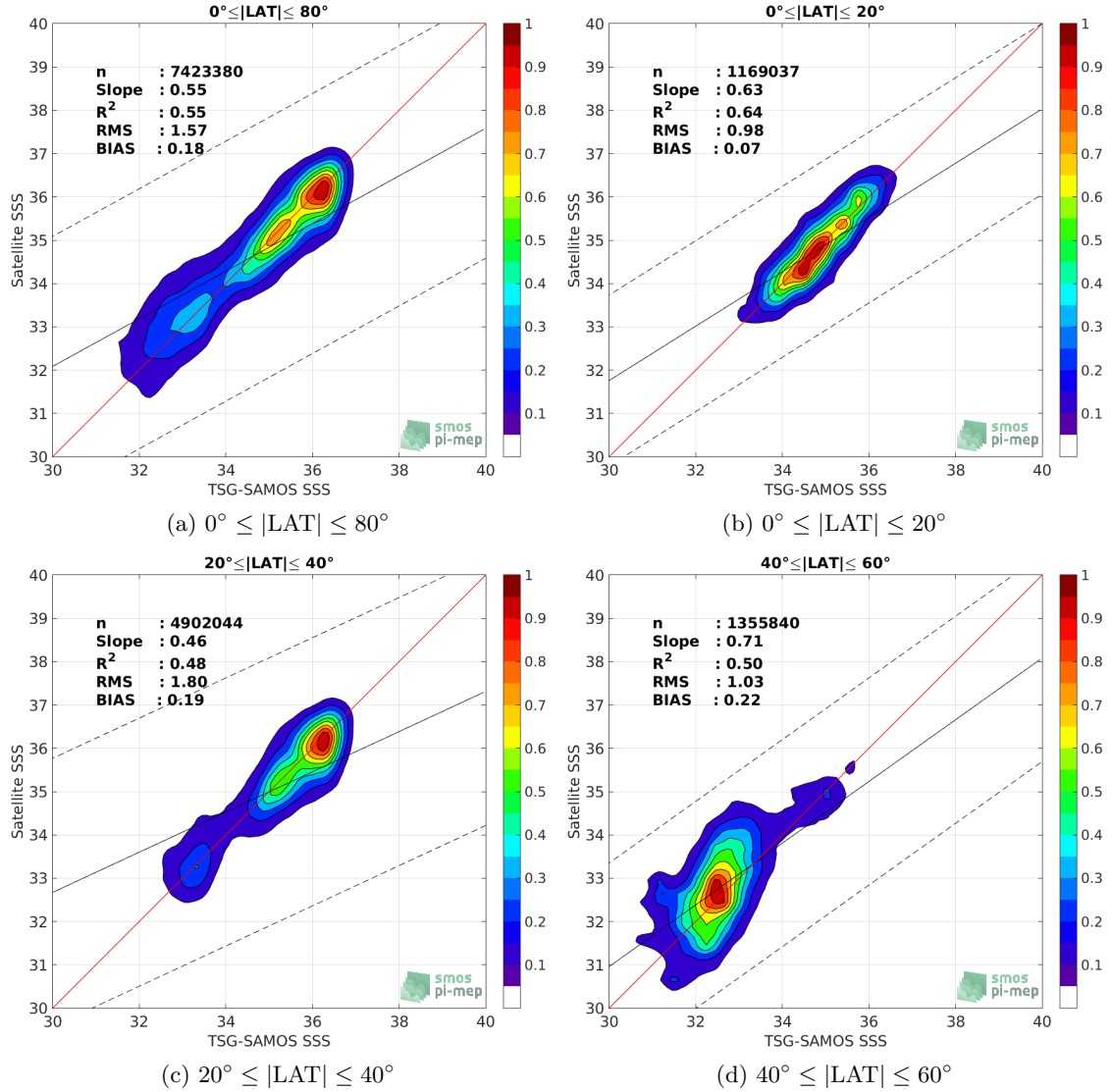
Figure 9: Contour maps of the concentration of SMOS-L3-CATDS-CPDC-V3-10DAYS-25KM SSS (y-axis) versus TSG-SAMOS SSS (x-axis) at match-up pairs for different latitude bands. For each plot, the red line shows x=y . The black thin and dashed lines indicate a linear fit through the data cloud and the \pm 95\% confidence levels, respectively. The number match-up pairs n , the slope and R^2 coefficient of the linear fit, the root mean square (RMS) and the mean bias between satellite and in situ data are indicated for each latitude band in each plots.
