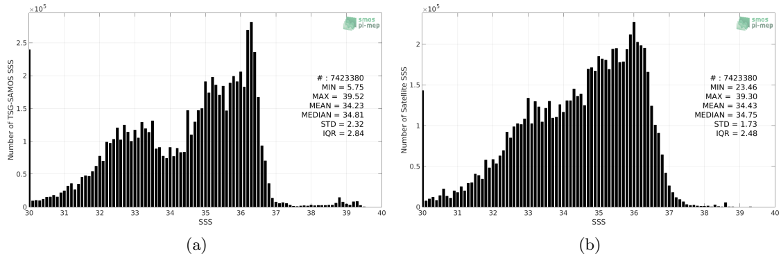
Figure 2: Histograms of SSS from TSG-SAMOS (a) and SMOS-L3-CATDS-CPDC-V3-10DAYS-25KM (b) considering all match-up pairs per bins of 0.1 over the SMOS coastal zone ( \leq 800 km) 60N-60S Pi-MEP region and for the full satellite product period.
