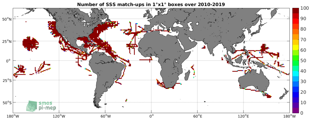
Figure 4: Number of SSS match-ups between TSG-SAMOS SSS and the SMOS-L3-CATDS-CPDC-V3-10DAYS-25KM SSS product for the SMOS coastal zone ( \geq 800\text{km} ) 60^\circ\text{N} - 60^\circ\text{S} Pi-MEP region over 1^\circ \times 1^\circ boxes and for the full satellite product period.
