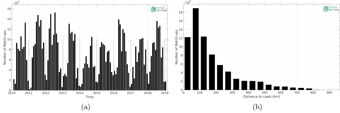
Figure 1: Number of match-ups between TSG-SAMOS and SMOS-L3-CATDS-CPDC-V3-10DAYS-25KM SSS as a function of time (a) and as function of the distance to coast (b) over the SMOS coastal zone ( \leq 800 km) 60N-60S Pi-MEP region and for the full satellite product period.
