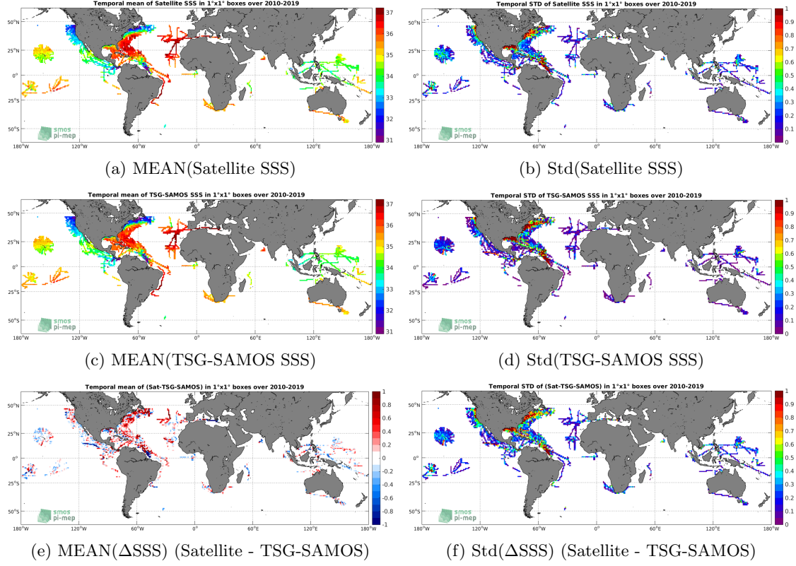
Figure 6: Temporal mean (left) and Std (right) of SSS from SMOS-L3-CATDS-CPDC-V3-10DAYS-25KM (top), TSG-SAMOS (middle), and of \Delta SSS (Satellite - TSG-SAMOS). Only match-up pairs are used to generate these maps.
