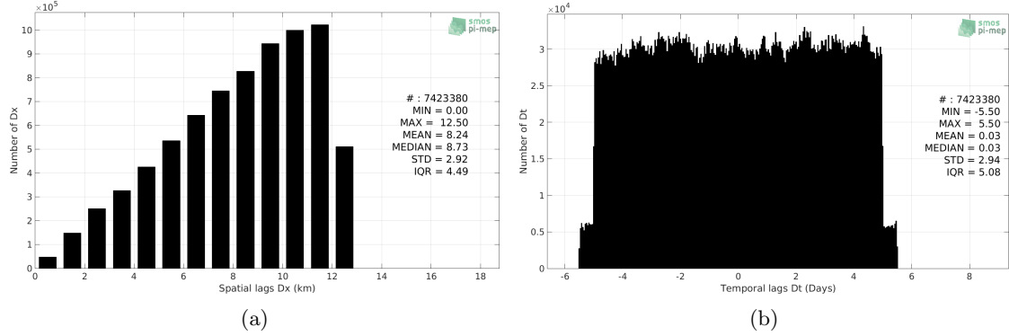
Figure 5: Histograms of the spatial (a) and temporal (b) lags between the time of the TSG-SAMOS measurements and the date of the corresponding SMOS-L3-CATDS-CPDC-V3-10DAYS-25KM SSS product.
