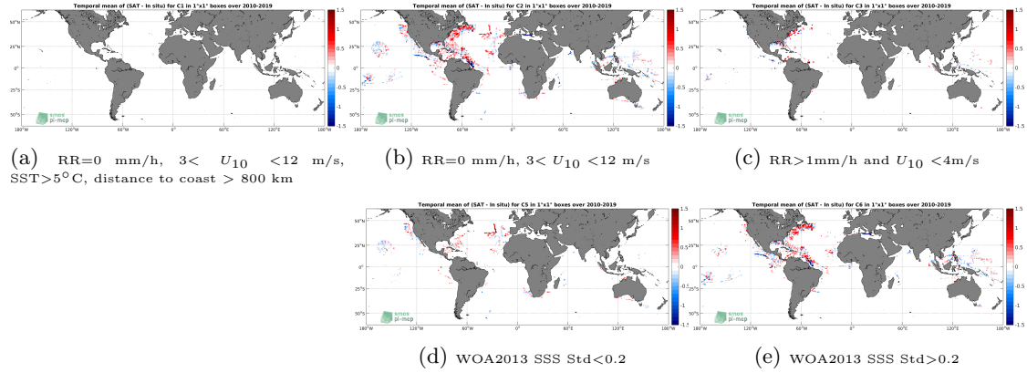
Figure 12: Temporal mean gridded over spatial boxes of size 1^\circ \times 1^\circ of \Delta SSS (SMOS-L3-CATDS-CPDC-V3-10DAYS-25KM - TSG-SAMOS) for 5 different subdatasets corresponding to: RR=0 mm/h, 3 < U_{10} < 12 m/s, SST > 5^\circ\text{C} , distance to coast > 800 km (a), RR=0 mm/h, 3 < U_{10} < 12 m/s (b), RR > 1 mm/h and U_{10} < 4 m/s (c), WOA2013 SSS Std < 0.2 (d), WOA2013 SSS Std > 0.2 (e).
