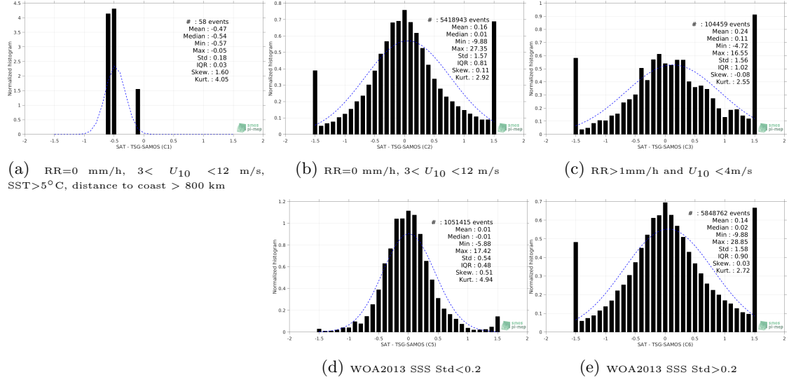
Figure 13: Normalized histogram of \Delta SSS (SMOS-L3-CATDS-CPDC-V3-10DAYS-25KM - TSG-SAMOS) for 5 different subdatasets corresponding to: RR=0 mm/h, 3 < U_{10} < 12 m/s, SST > 5°C, distance to coast > 800 km (a), RR=0 mm/h, 3 < U_{10} < 12 m/s (b), RR > 1mm/h and U_{10} < 4 m/s (c), WOA2013 SSS Std < 0.2 (d), WOA2013 SSS Std > 0.2 (e).
