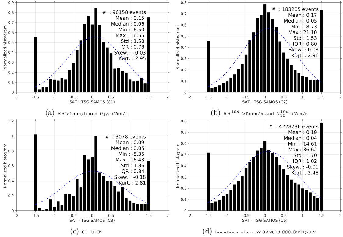
Figure 13: Normalized histogram of \Delta SSS (SMOS-L3-CATDS-CPDC-V3-10DAYS-25KM - TSG-SAMOS) for 6 different subdatasets corresponding to: RR > 1\text{mm/h} and U_{10} < 5\text{m/s} (a), RR^{10d} > 5\text{mm/h} and U_{10}^{10d} < 5\text{m/s} (b), C1 U C2 (c), Locations where WOA2013 SSS STD > 0.2 (d).
