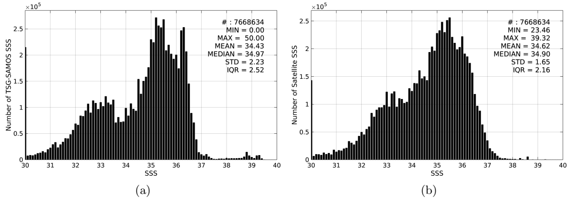
Figure 2: Histograms of SSS from TSG-SAMOS (a) and SMOS-L3-CATDS-CPDC-V3-10DAYS-25KM (b) considering all match-up pairs per bins of 0.1 over the SMOS coastal zone ( \geq 800 km) 60N-60S Pi-MEP region and for the full satellite product period.
