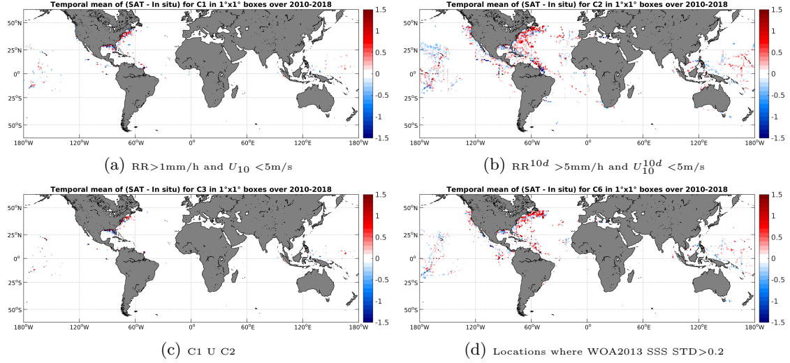
Figure 12: Temporal mean gridded over spatial boxes of size 1^\circ \times 1^\circ of \Delta SSS (SMOS-L3-CATDS-CPDC-V3-10DAYS-25KM - TSG-SAMOS) for 4 different subdatasets corresponding to: RR > 1mm/h and U_{10} < 5 m/s (a), RR^{10d} > 5 mm/h and U_{10}^{10d} < 5 m/s (b), C1 U C2 (c), Locations where WOA2013 SSS STD > 0.2 (d).
