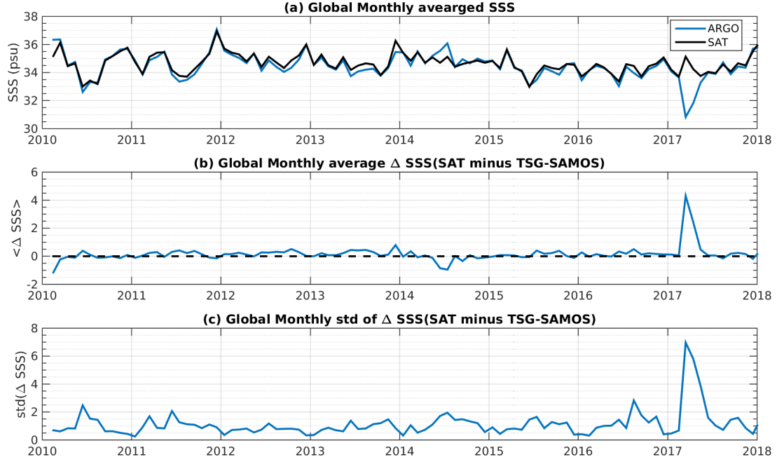
Figure 7: Time series of the monthly averaged mean SSS (top), mean \Delta SSS (Satellite - TSG-SAMOS) and STD of \Delta SSS (Satellite - TSG-SAMOS) over the SMOS coastal zone ( \geq 800\text{km} ) 60N-60S Pi-MEP region considering all match-ups collected by the Pi-MEP platform.
