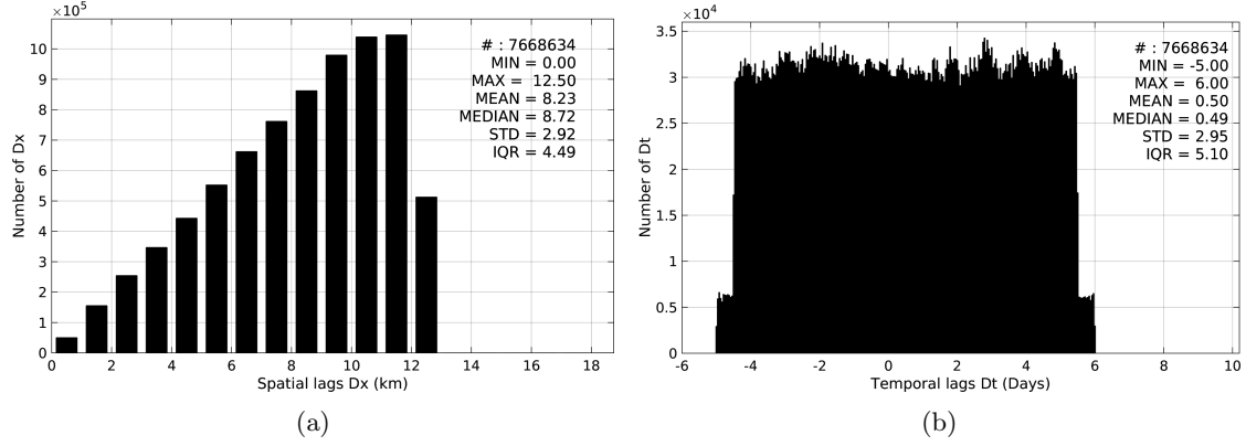
Figure 5: Histograms of the spatial (a) and temporal (b) lags between the time of the TSG-SAMOS measurements and the date of the corresponding SMOS-L3-CATDS-CPDC-V3-10DAYS-25KM SSS product.
