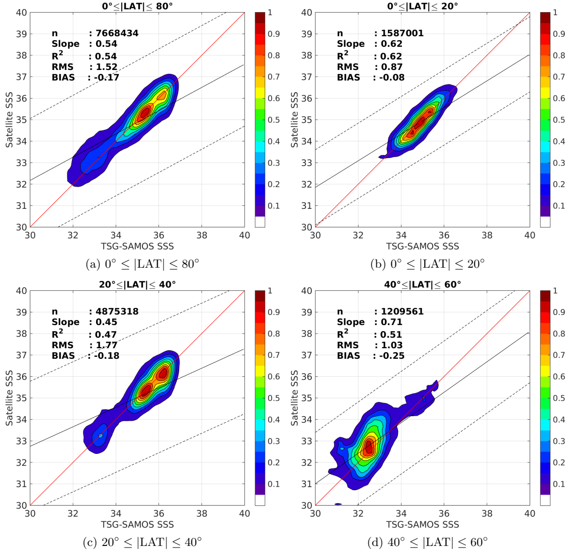
Figure 9: Contour maps of the concentration of SMOS-L3-CATDS-CPDC-V3-10DAYS-25KM SSS (y-axis) versus TSG-SAMOS SSS (x-axis) at match-up pairs for different latitude bands. For each plot, the red line shows x=y . The black thin and dashed lines indicate a linear fit through the data cloud and the \pm 95\% confidence levels, respectively. The number match-up pairs n , the slope and R^2 coefficient of the linear fit, the root mean square (RMS) and the mean bias between satellite and in situ data are indicated for each latitude band in each plots.
