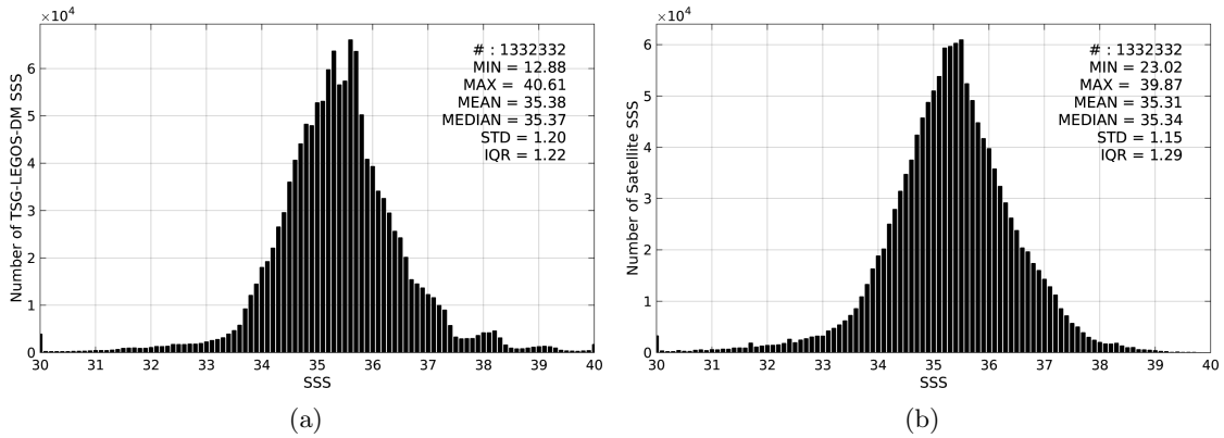
Figure 2: Histograms of SSS from TSG-LEGOS-DM (a) and SMOS-L3-CATDS-CPDC-V3-10DAYS-25KM (b) considering all match-up pairs per bins of 0.1 over the SMOS coastal zone ( \leq 800 km) 60N-60S Pi-MEP region and for the full satellite product period.
