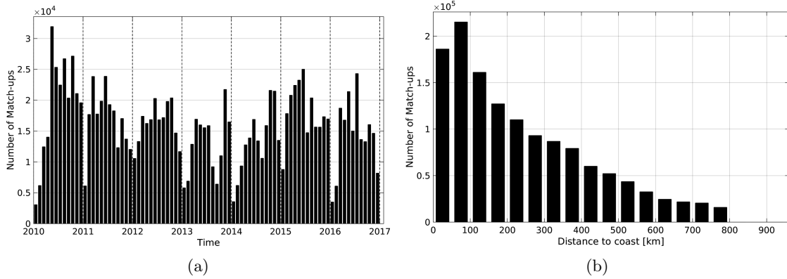
Figure 1: Number of match-ups between TSG-LEGOS-DM and SMOS-L3-CATDS-CPDC-V3-10DAYS-25KM SSS as a function of time (a) and as function of the distance to coast (b) over the SMOS coastal zone ( \leq 800 km) 60N-60S Pi-MEP region and for the full satellite product period.
