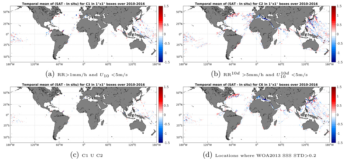
Figure 12: Temporal mean gridded over spatial boxes of size 1^\circ \times 1^\circ of \Delta SSS (SMOS-L3-CATDS-CPDC-V3-10DAYS-25KM - TSG-LEGOS-DM) for 4 different subdatasets corresponding to: RR > 1\text{mm/h} and U_{10} < 5\text{m/s} (a), RR^{10d} > 5\text{mm/h} and U_{10}^{10d} < 5\text{m/s} (b), C1 U C2 (c), Locations where WOA2013 SSS STD > 0.2 (d).
