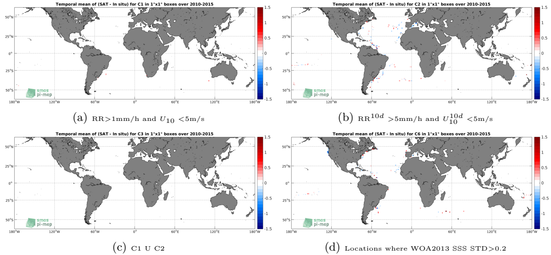
Figure 12: Temporal mean gridded over spatial boxes of size 1^\circ \times 1^\circ of \Delta SSS (SMOS-L3-CATDS-CPDC-V3-10DAYS-25KM - TSG-GOSUD-Sailing-ship) for 4 different subdatasets corresponding to: RR > 1\text{mm/h} and U_{10} < 5\text{m/s} (a), RR^{10d} > 5\text{mm/h} and U_{10}^{10d} < 5\text{m/s} (b), C1 U C2 (c), Locations where WOA2013 SSS STD > 0.2 (d).
