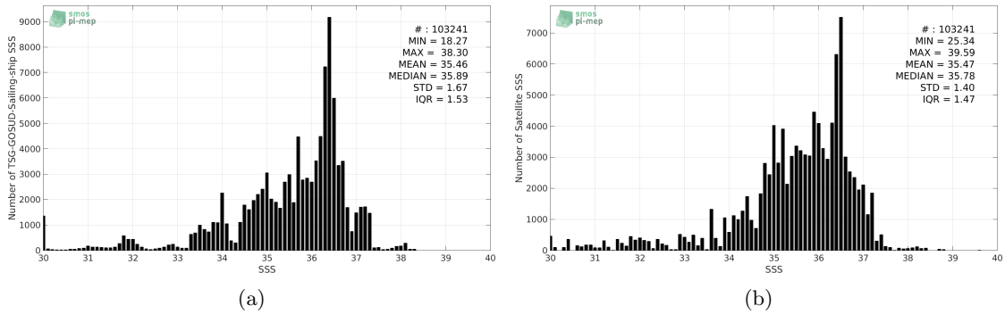
Figure 2: Histograms of SSS from TSG-GOSUD-Sailing-ship (a) and SMOS-L3-CATDS-CPDC-V3-10DAYS-25KM (b) considering all match-up pairs per bins of 0.1 over the SMOS coastal zone ( \approx 800\text{km} ) 60N-60S Pi-MEP region and for the full satellite product period.
