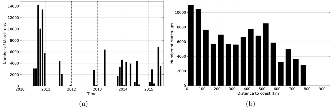
Figure 1: Number of match-ups between TSG-GOSUD-Sailing-ship and SMOS-L3-CATDS-CPDC-V3-10DAYS-25KM SSS as a function of time (a) and as function of the distance to coast (b) over the SMOS coastal zone ( \geq 800 km) 60N-60S Pi-MEP region and for the full satellite product period.
