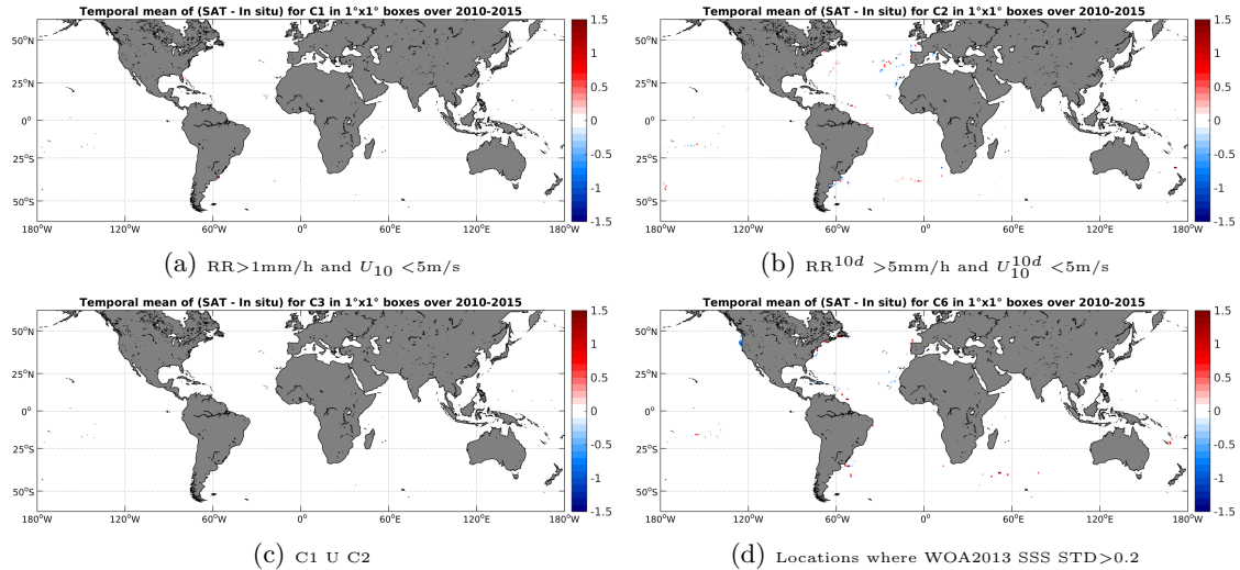
Figure 12: Temporal mean gridded over spatial boxes of size 1^\circ \times 1^\circ of \Delta SSS (SMOS-L3-CATDS-CPDC-V3-10DAYS-25KM - TSG-GOSUD-Sailing-ship) for 4 different subdatasets corresponding to:RR >1 mm/h and U_{10} < 5 m/s (a), RR^{10d} > 5 mm/h and U_{10}^{10d} < 5 m/s (b), C1 U C2 (c),Locations where WOA2013 SSS STD >0.2 (d).
