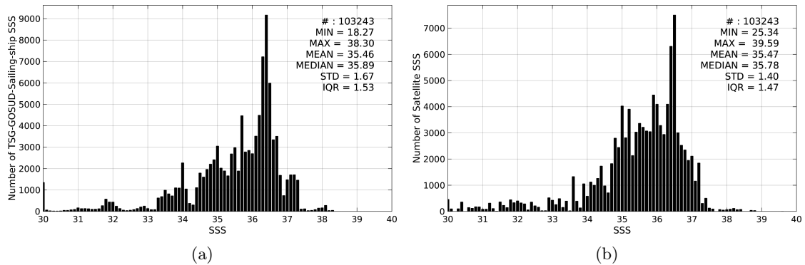
Figure 2: Histograms of SSS from TSG-GOSUD-Sailing-ship (a) and SMOS-L3-CATDS-CPDC-V3-10DAYS-25KM (b) considering all match-up pairs per bins of 0.1 over the SMOS coastal zone ( \geq 800 km) 60N-60S Pi-MEP region and for the full satellite product period.
