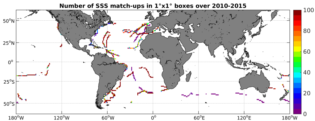
Figure 4: Number of SSS match-ups between TSG-GOSUD-Sailing-ship SSS and the SMOS-L3-CATDS-CPDC-V3-10DAYS-25KM SSS product for the SMOS coastal zone ( \approx 800\text{km} ) 60N-60S Pi-MEP region over 1^\circ \times 1^\circ boxes and for the full satellite product period.
