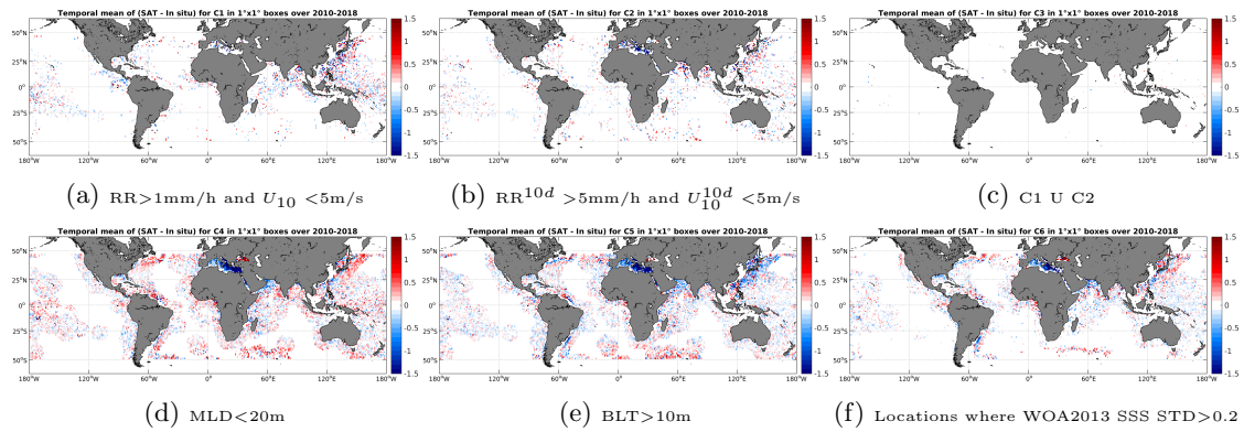
Figure 12: Temporal mean gridded over spatial boxes of size 1^\circ \times 1^\circ of \Delta SSS (SMOS-L3-CATDS-CPDC-V3-10DAYS-25KM - Argo) for 6 different subdatasets corresponding to:RR >1 mm/h and U_{10} < 5 m/s (a), RR ^{10d} > 5 mm/h and U_{10}^{10d} < 5 m/s (b), C1 U C2 (c),MLD <20 m (d),BLT >10 m (e),Locations where WOA2013 SSS STD >0.2 (f).
