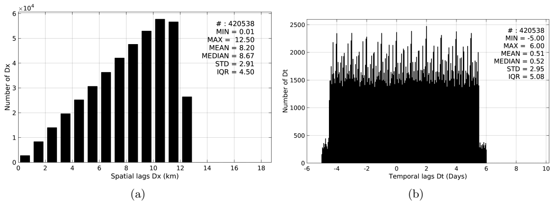
Figure 5: Histograms of the spatial (a) and temporal (b) lags between the time of the Argo measurements and the date of the corresponding SMOS-L3-CATDS-CPDC-V3-10DAYS-25KM SSS product.
