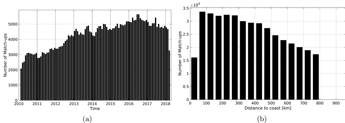
Figure 1: Number of match-ups between Argo and SMOS-L3-CATDS-CPDC-V3-10DAYS-25KM SSS as a function of time (a) and as function of the distance to coast (b) over the SMOS coastal zone ( \pm 800 km) 60N-60S Pi-MEP region and for the full satellite product period.
