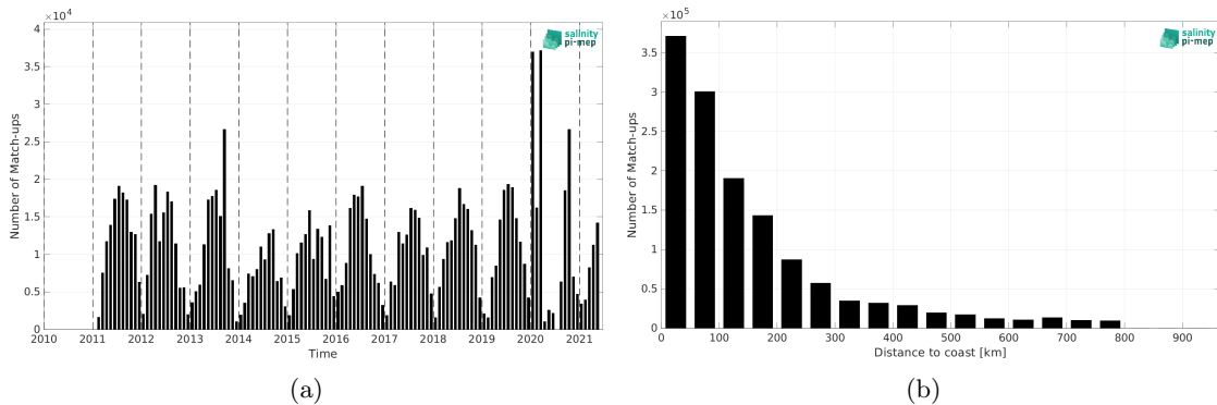
Figure 2: Number of match-ups between TSG (SAMOS) and SMOS SSS L3 v2 - 9-Days (BEC) SSS as a function of time (a) and as function of the distance to coast (b) over the SMOS coastal zone (<800km) 60N-60S Pi-MEP region and for the full satellite product period.
