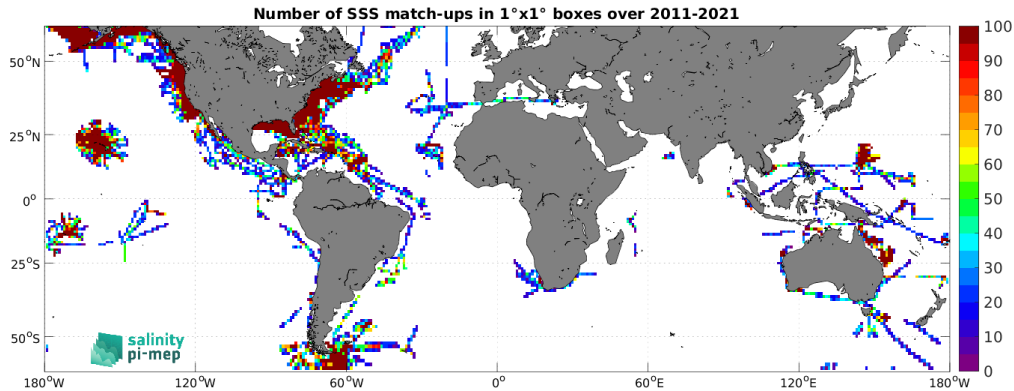
Figure 5: Number of SSS match-ups between TSG (SAMOS) SSS and the SMOS SSS L3 v2 - 9-Days (BEC) SSS product for the SMOS coastal zone (<800km) 60N-60S Pi-MEP region over 1^\circ \times 1^\circ boxes and for the full satellite product period.
