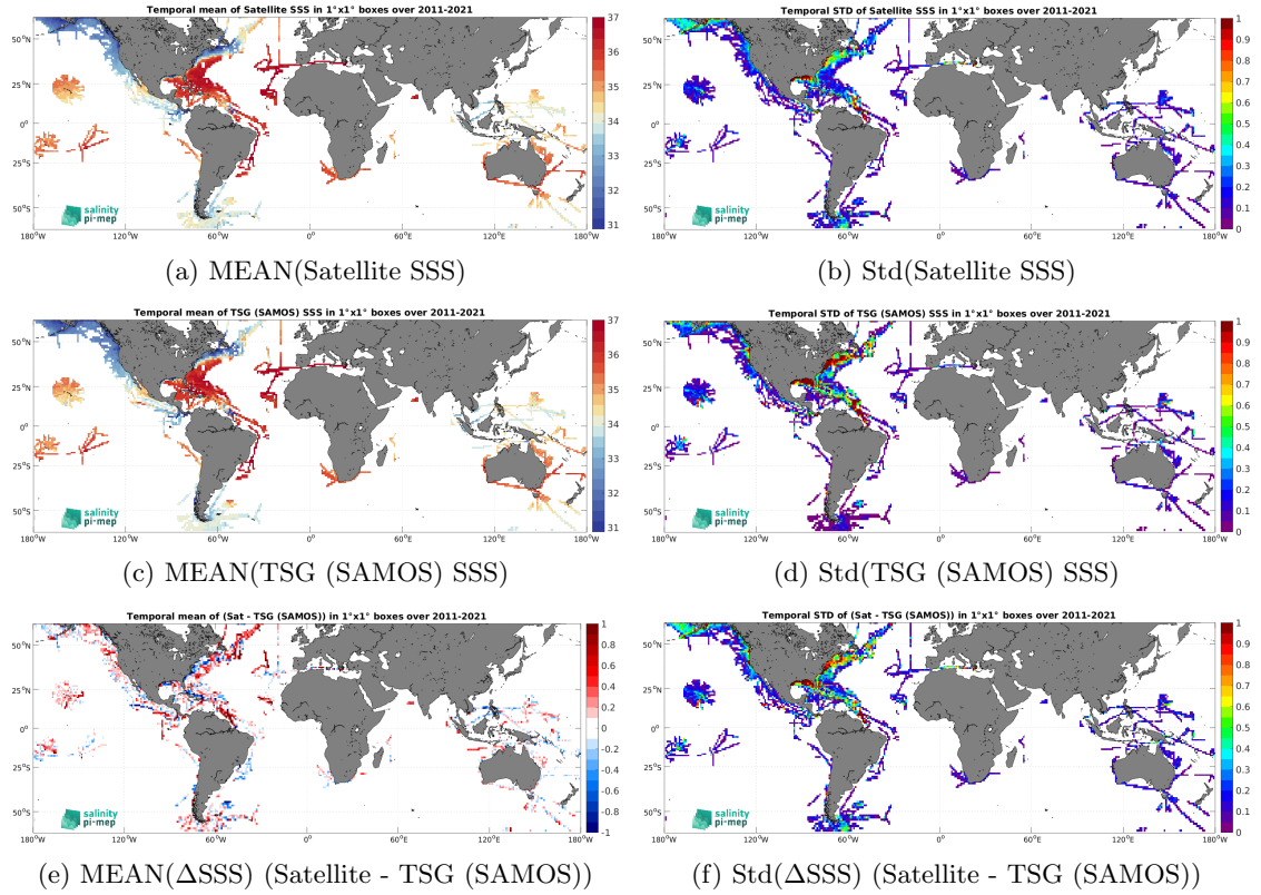
Figure 7: Temporal mean (left) and Std (right) of SSS from SMOS SSS L3 v2 - 9-Days (BEC) (top), TSG (SAMOS) (middle), and of \Delta SSS (Satellite - TSG (SAMOS)). Only match-up pairs are used to generate these maps.
