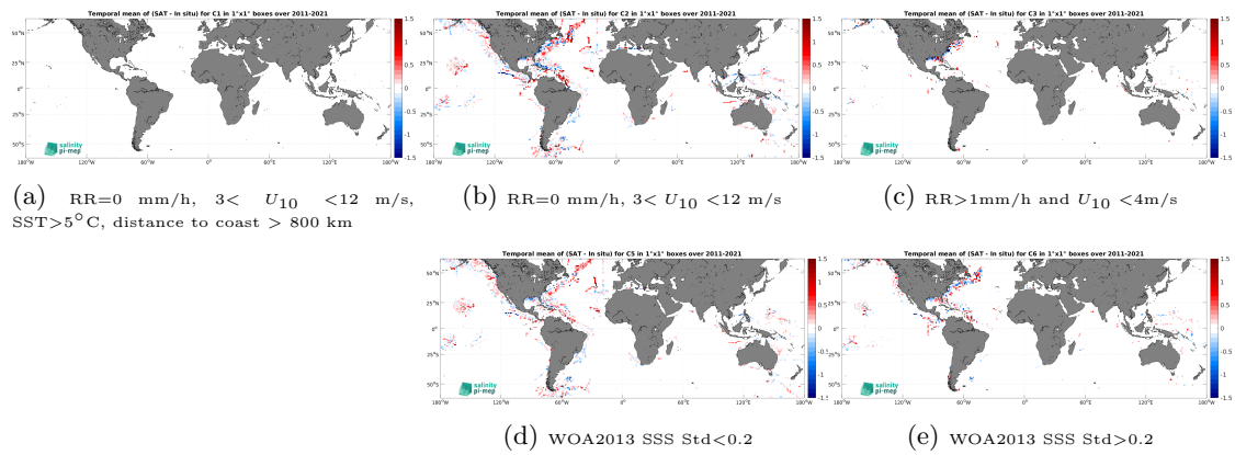
Figure 14: Temporal mean gridded over spatial boxes of size 1^\circ \times 1^\circ of \Delta\text{SSS} (SMOS SSS L3 v2 - 9-Days (BEC) - TSG (SAMOS)) for 5 different subdatasets corresponding to:RR=0 mm/h, 3 < U_{10} < 12 m/s, SST >5^\circ\text{C} , distance to coast > 800 km (a), RR=0 mm/h, 3 < U_{10} < 12 m/s (b), RR >1 mm/h and U_{10} < 4 m/s (c), WOA2013 SSS Std <0.2 (d), WOA2013 SSS Std >0.2 (e).
